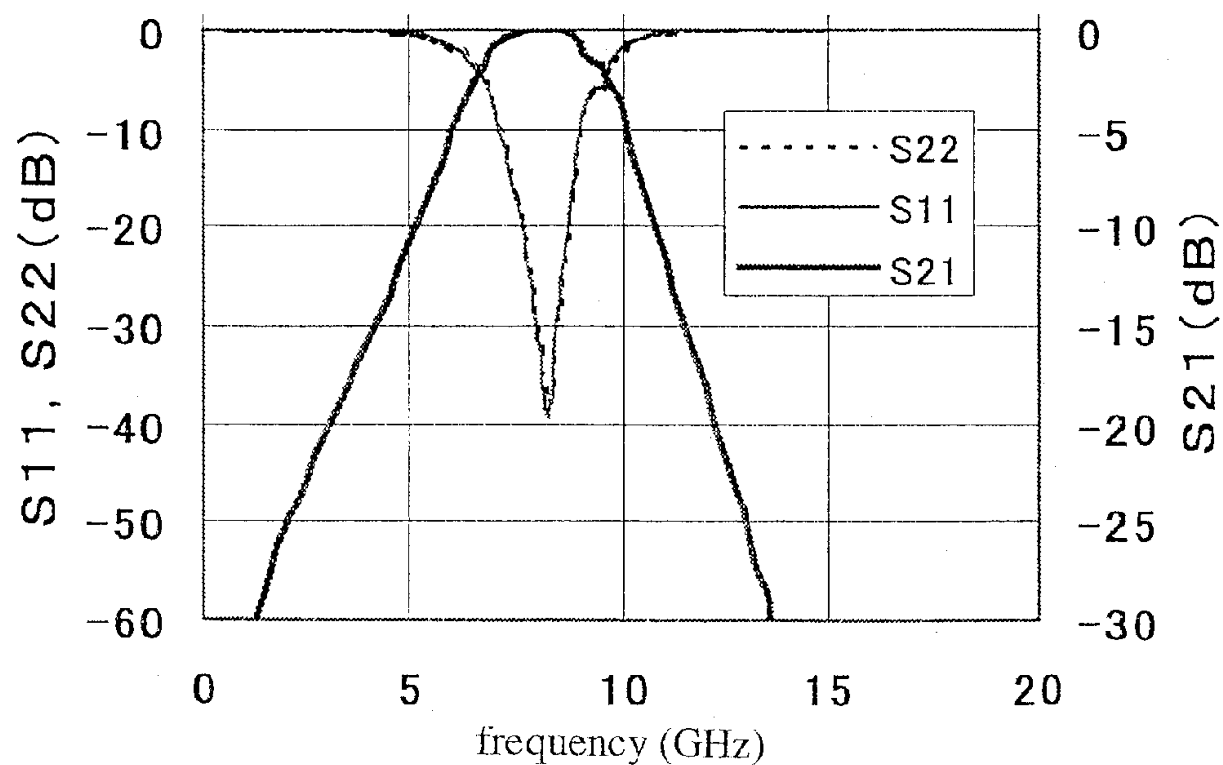
(b) Example characteristics for narrow band bandpass filter
