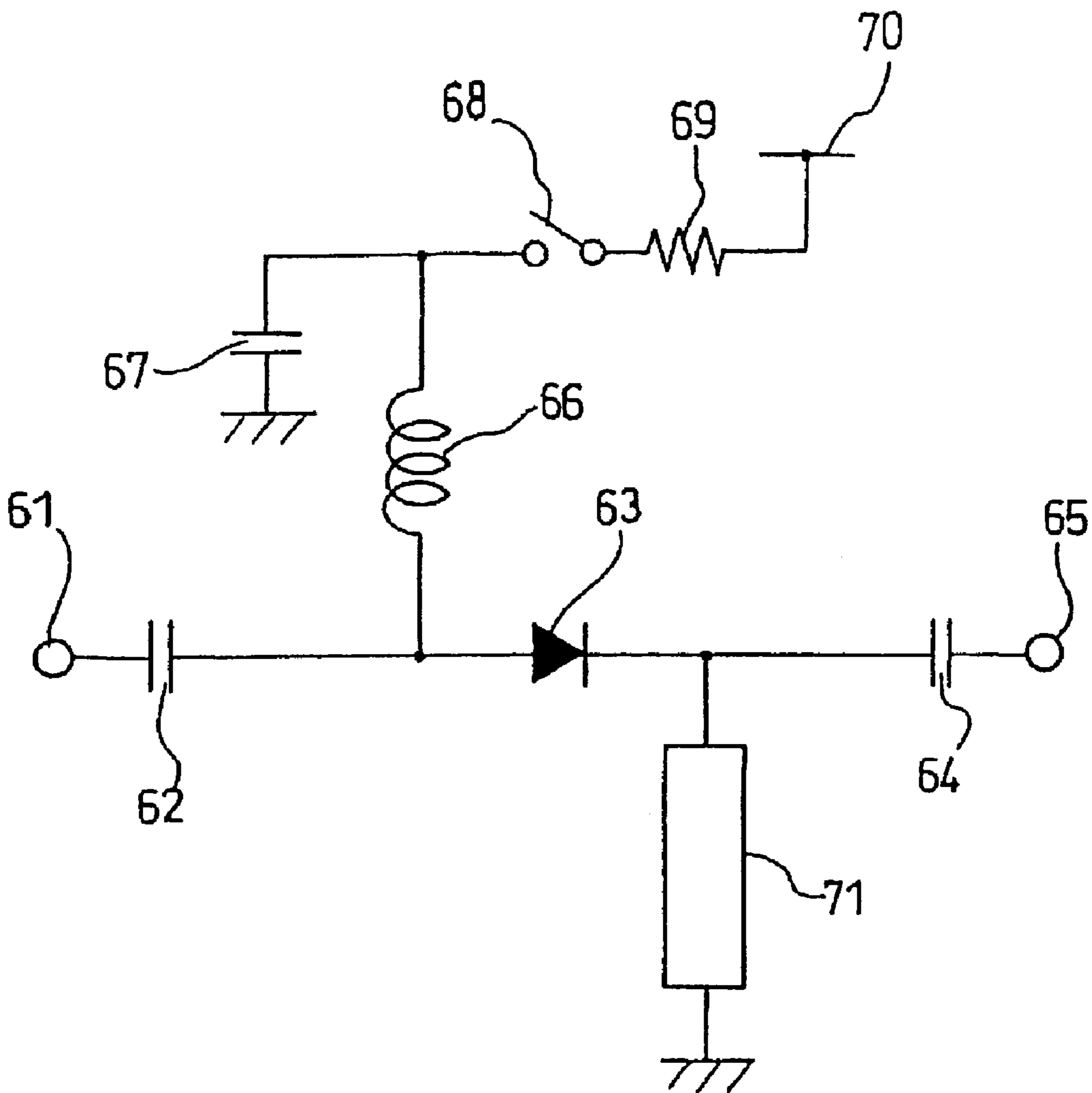
FIG. 8 PRIOR ART
