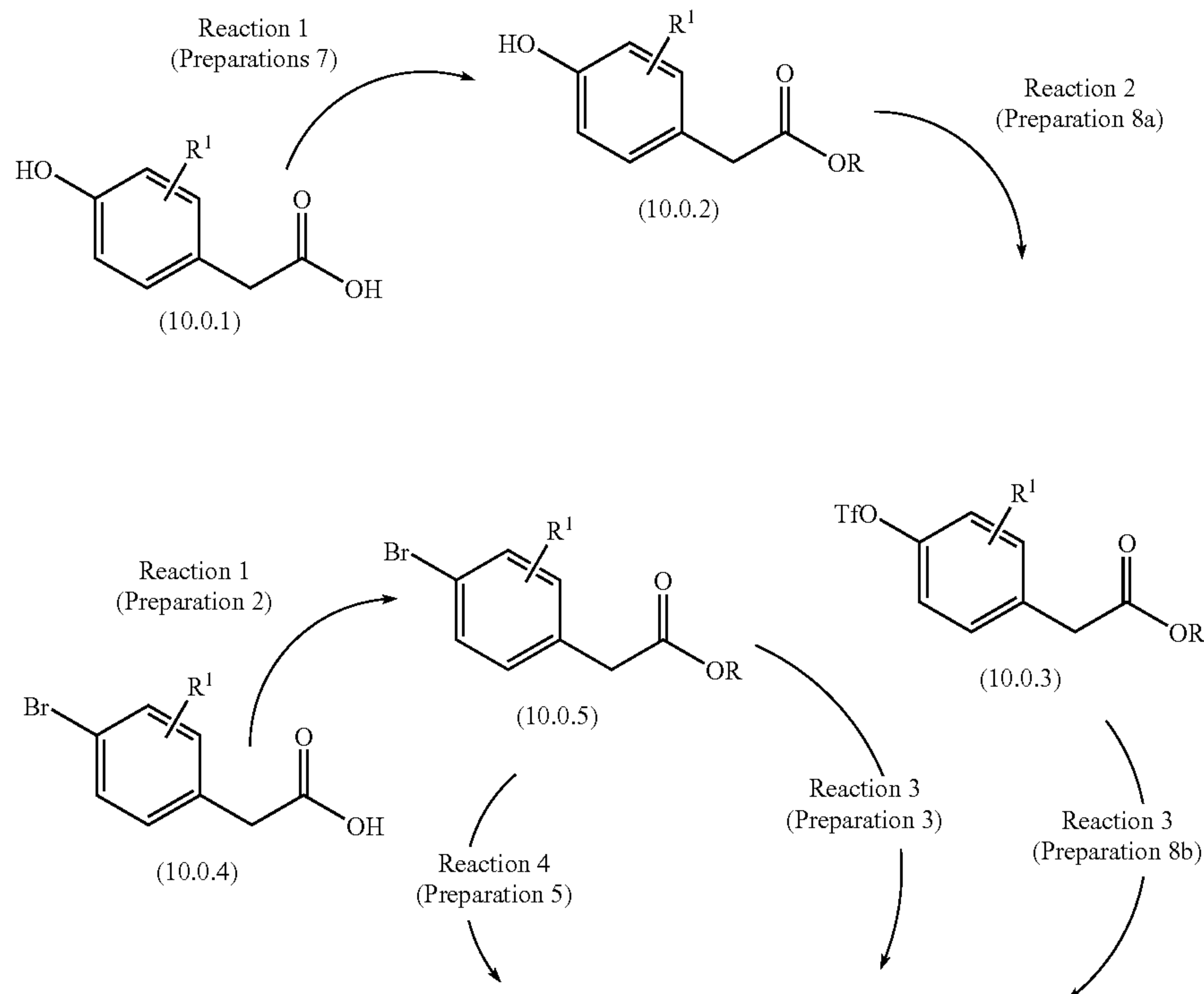
SYNTHESIS SCHEME (10.0.0)
