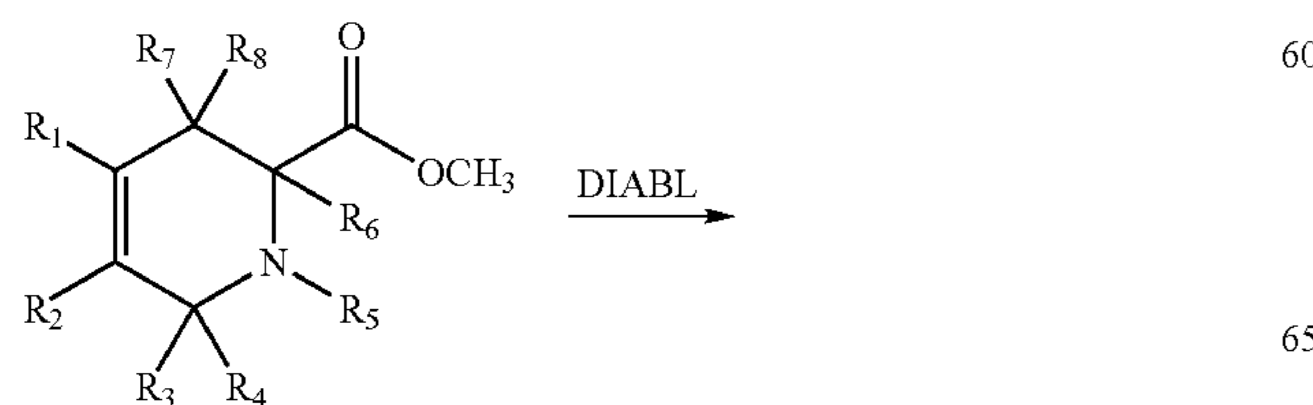
Scheme 3
