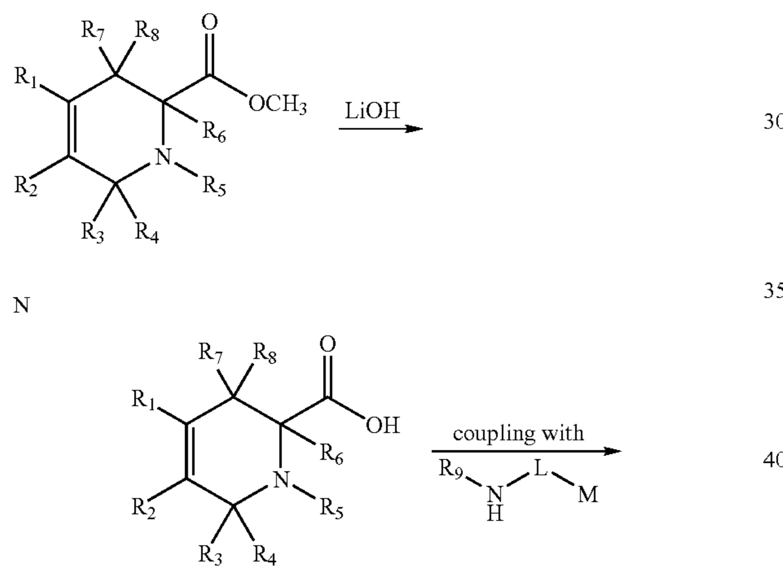
Scheme 2
