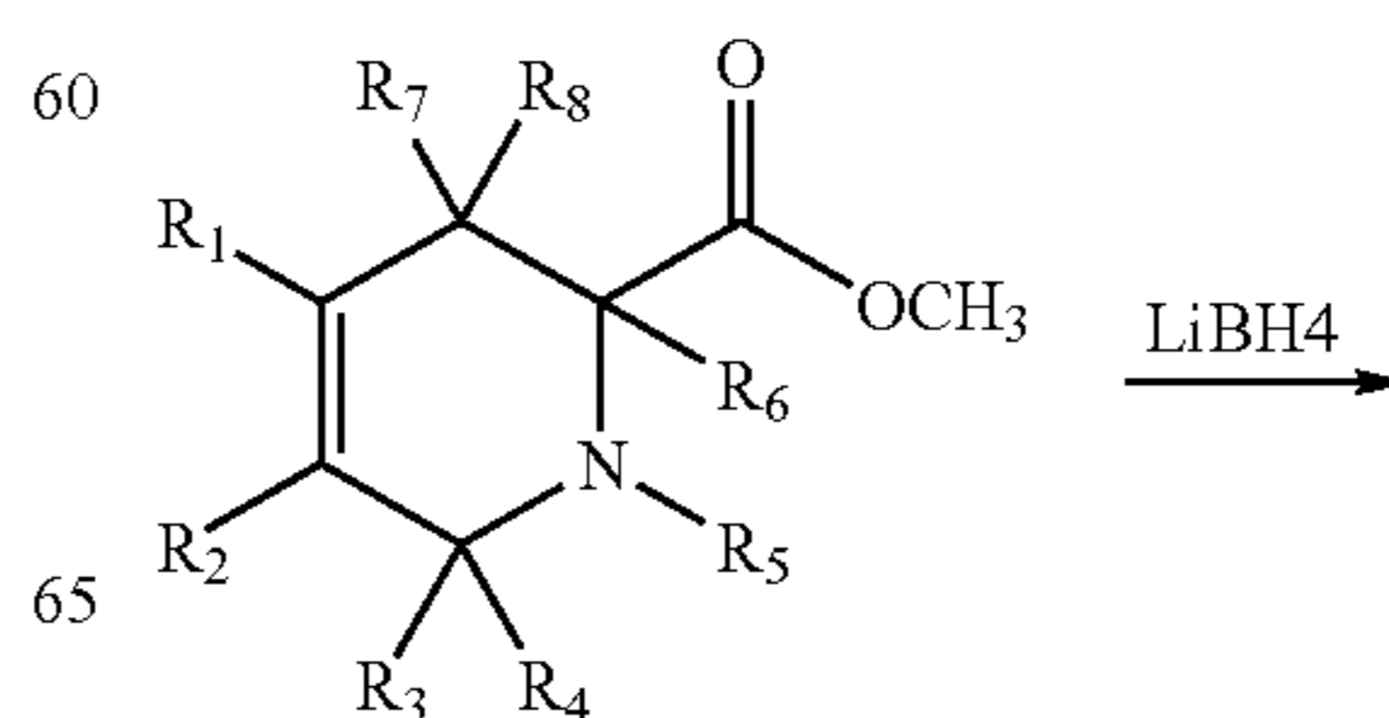
Scheme 4
