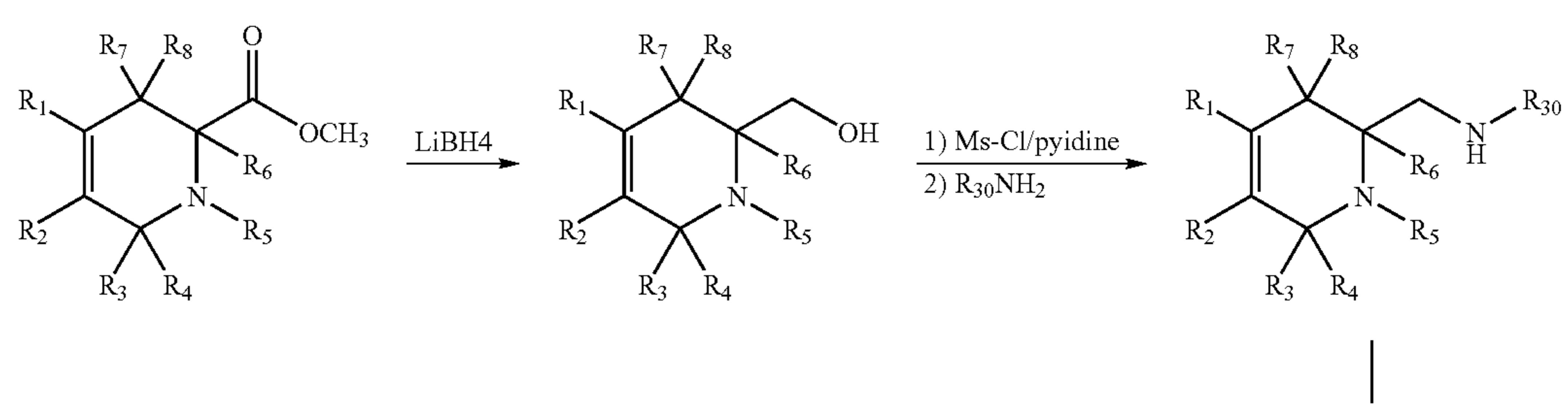
Scheme 5
