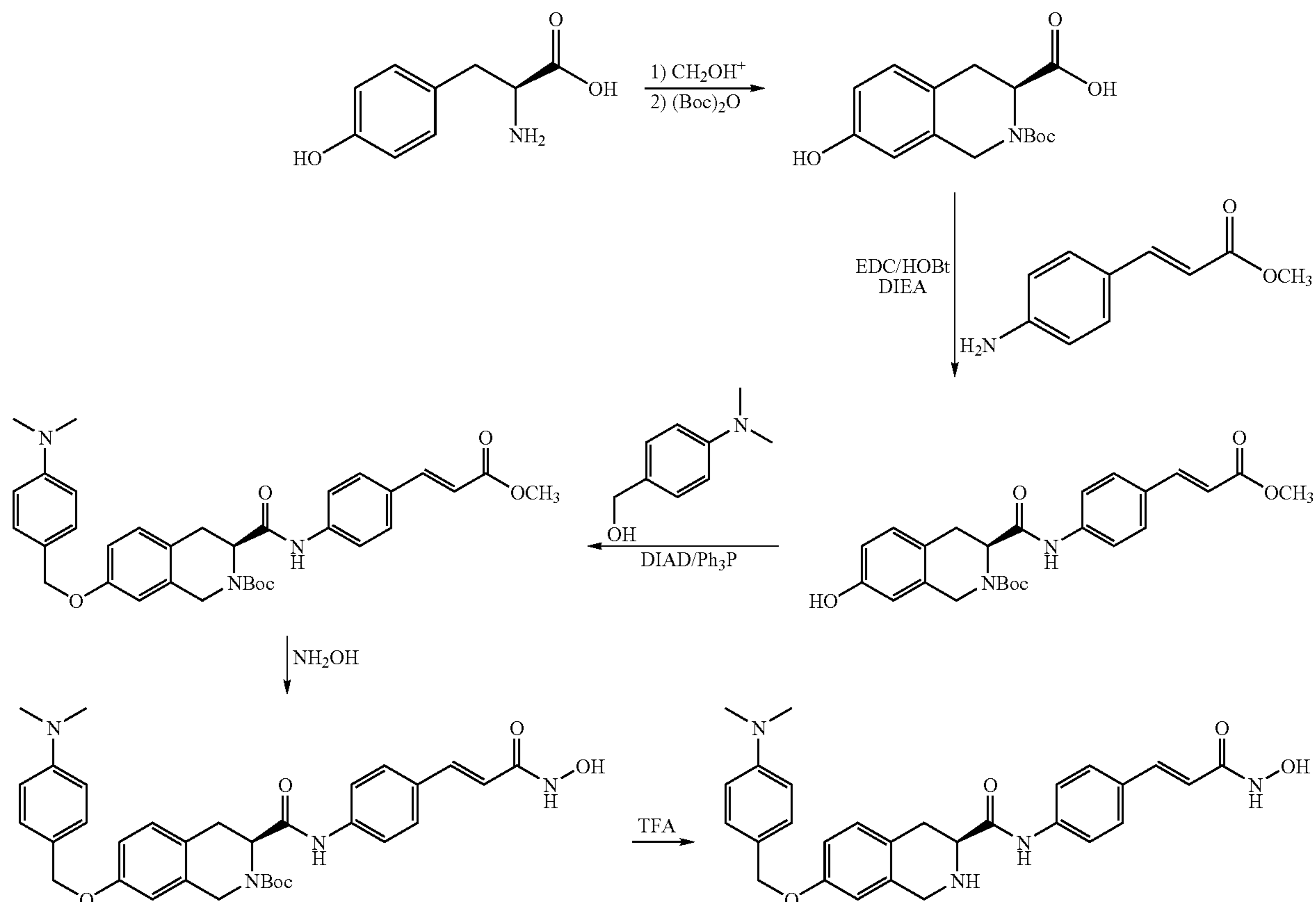
Scheme 7
