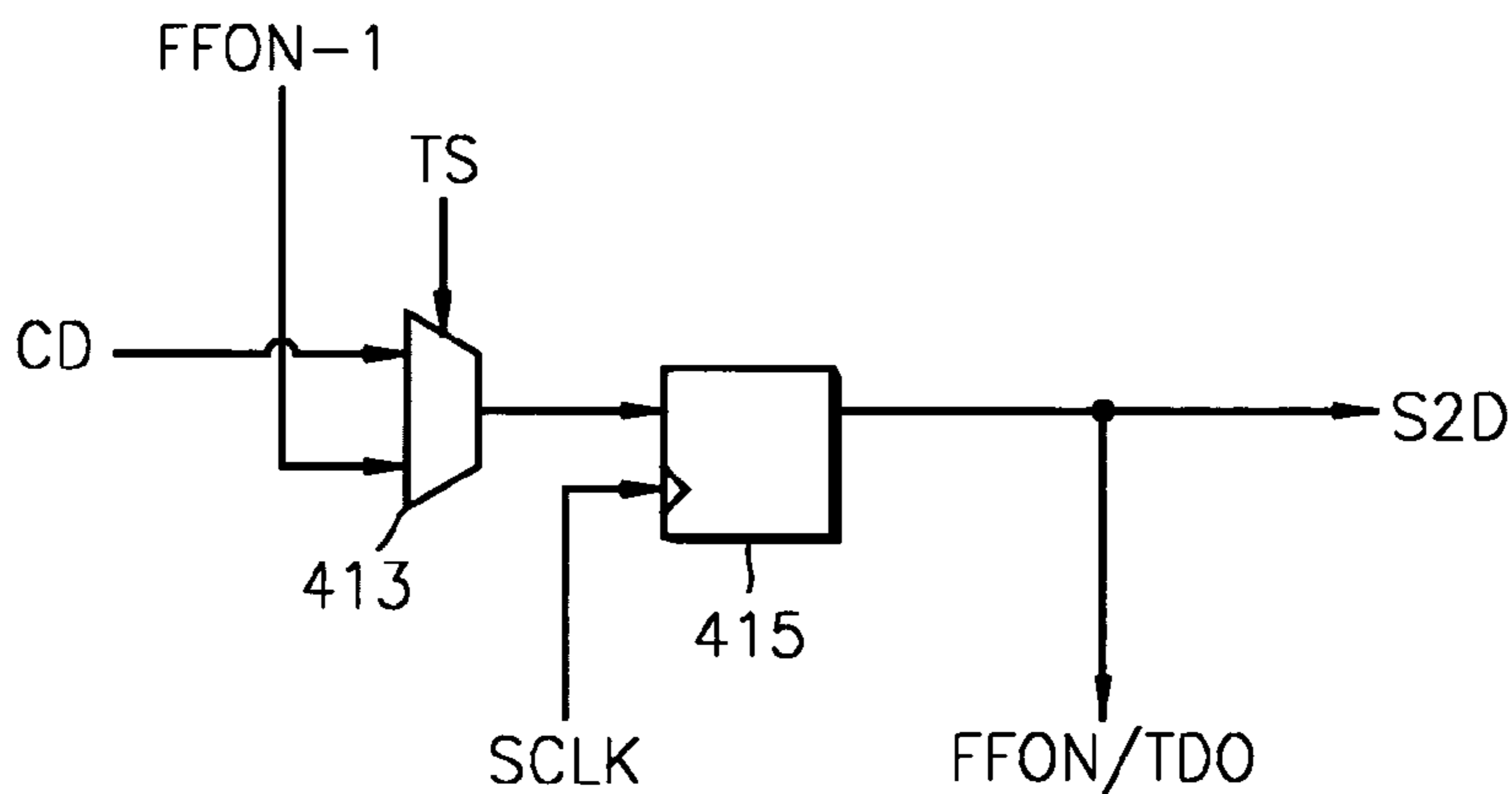
FIG. 4 (PRIOR ART)
