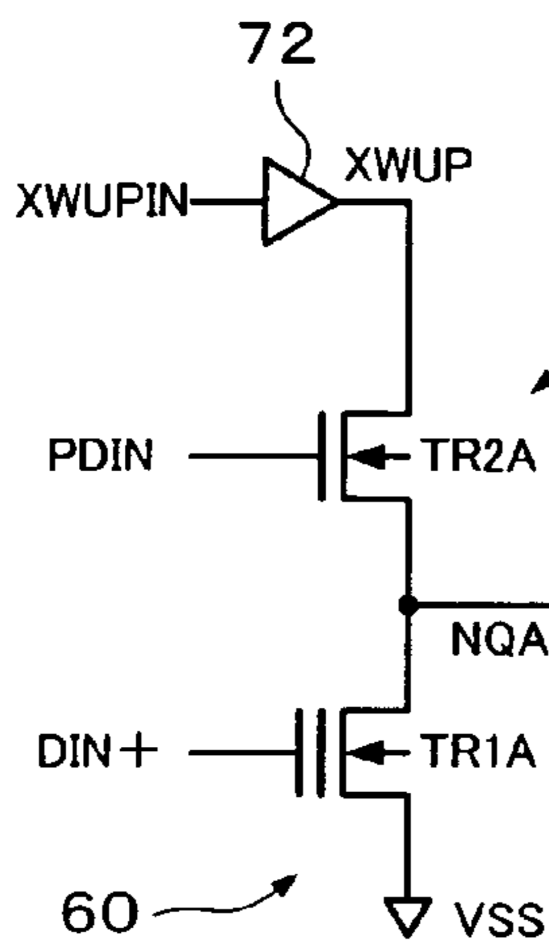
TRANSMITTER CIRCUIT
