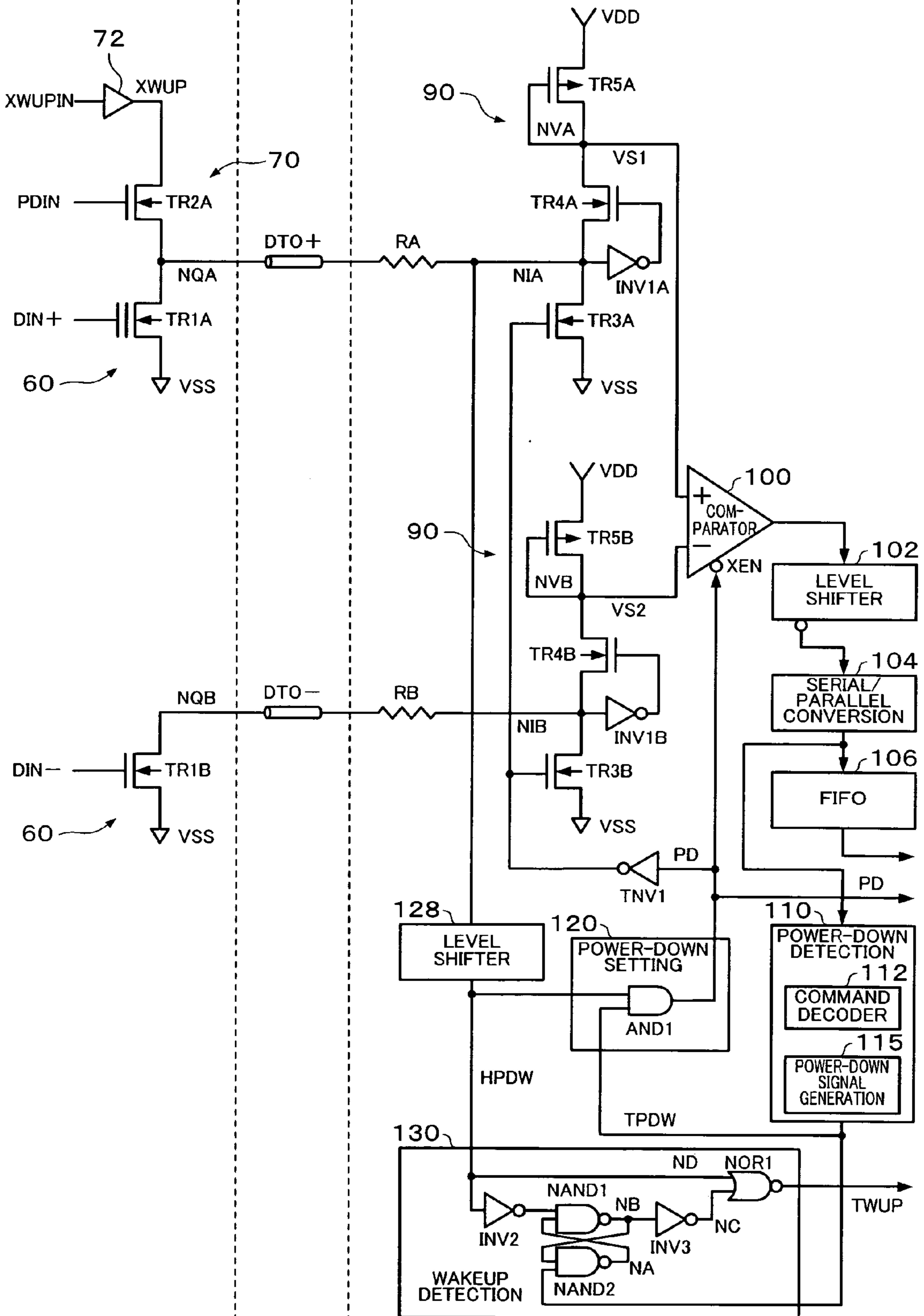
TRANSMITTER CIRCUIT
