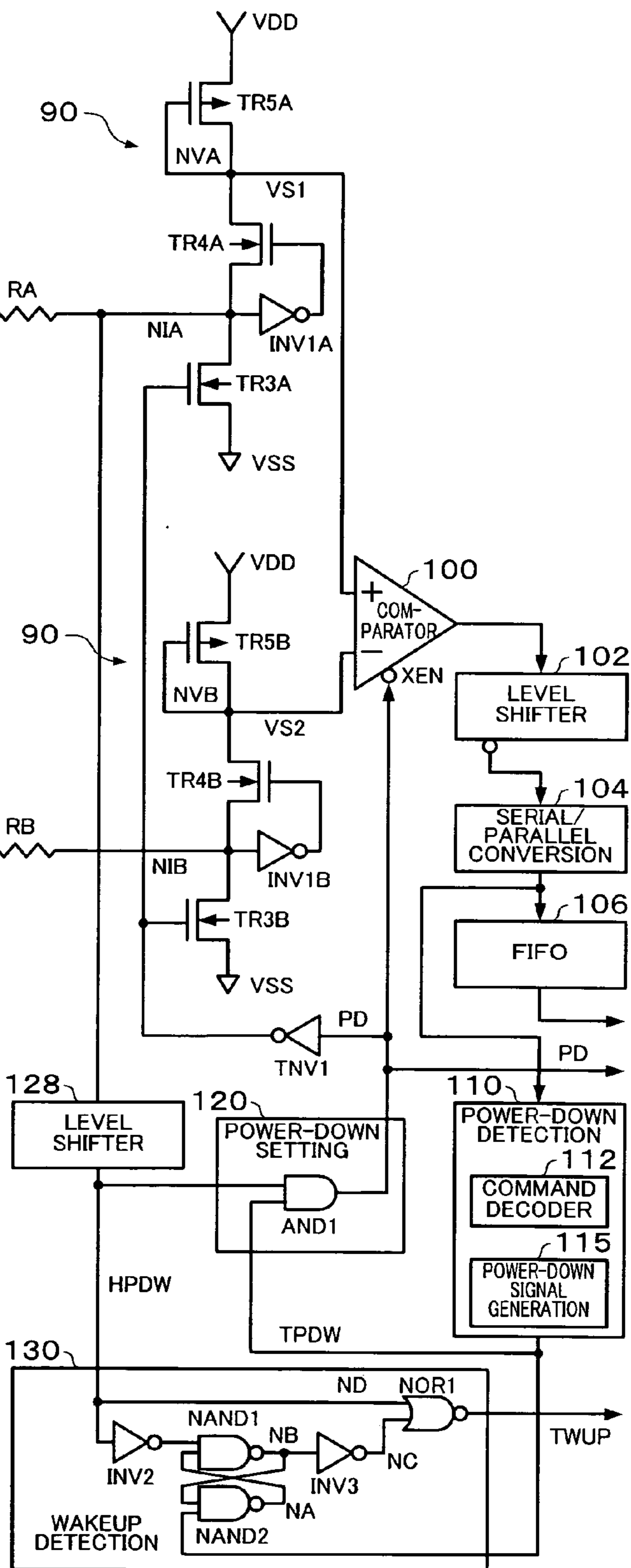
RECEIVER CIRCUIT
