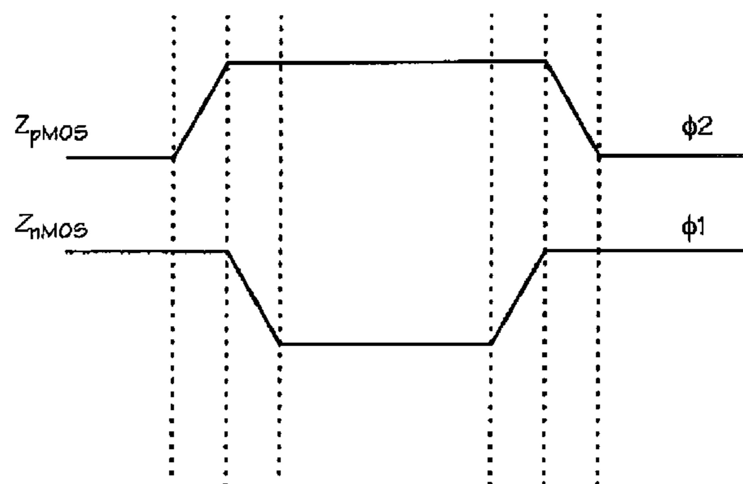
Non-overlapping clocks
