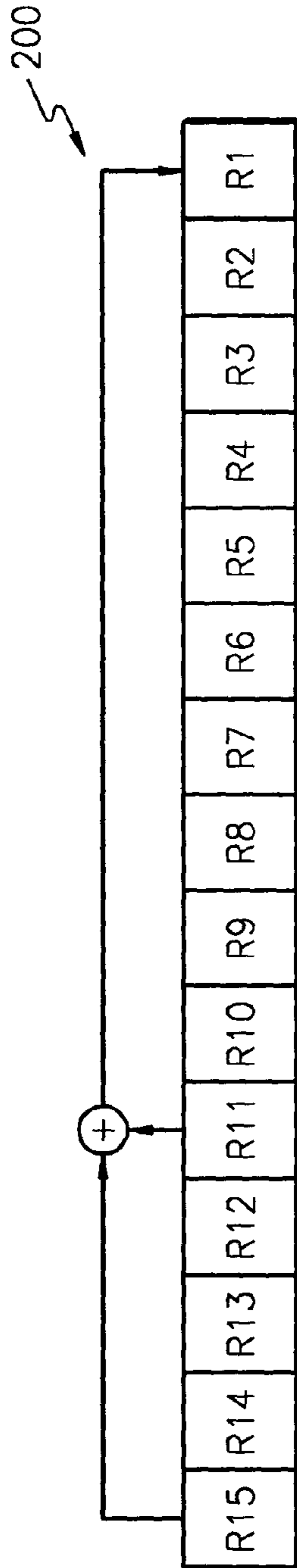
FIG. 2 (PRIOR ART)
