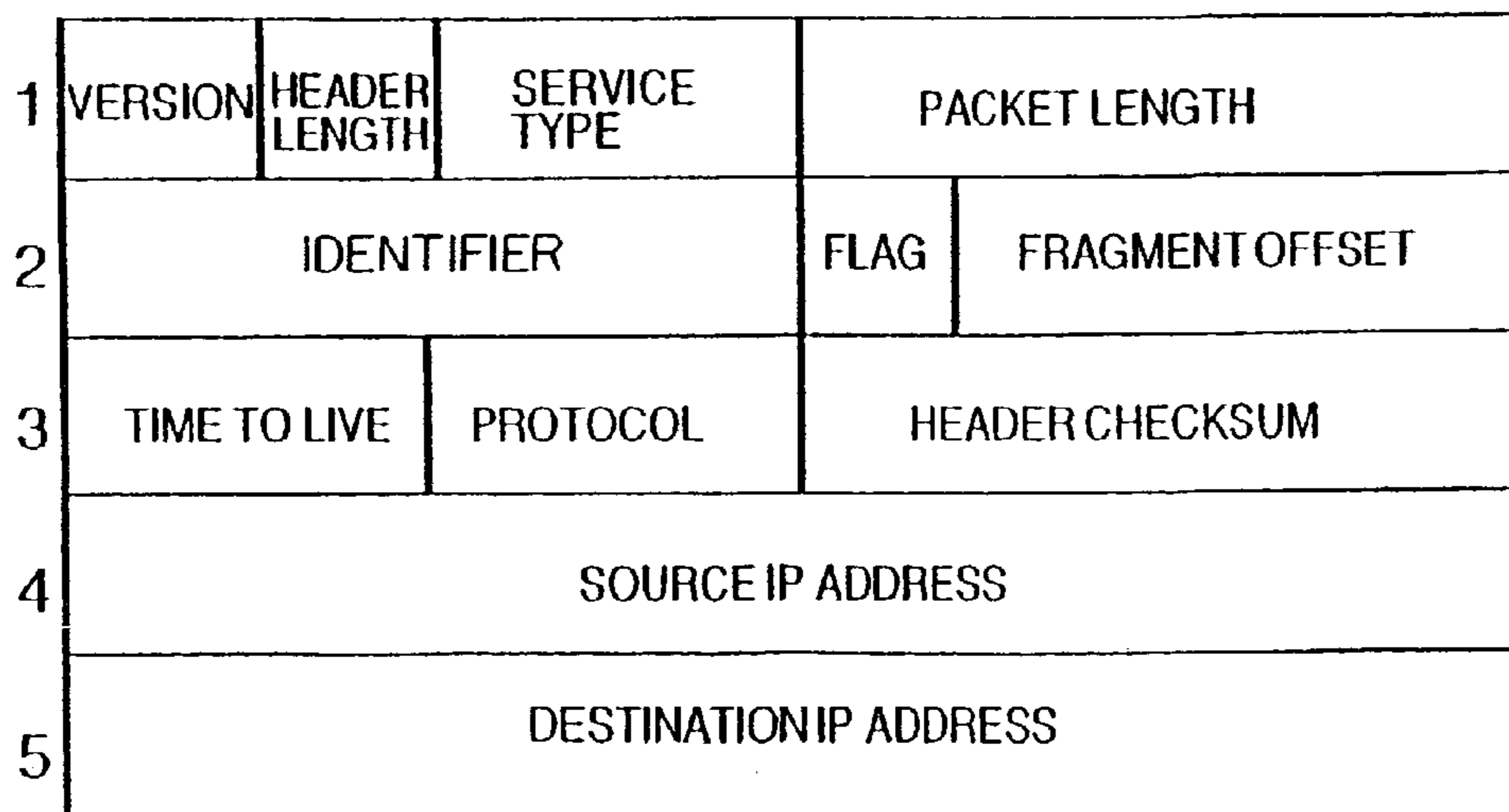
FIG. 11B IPv4 HEADER FORMAT
