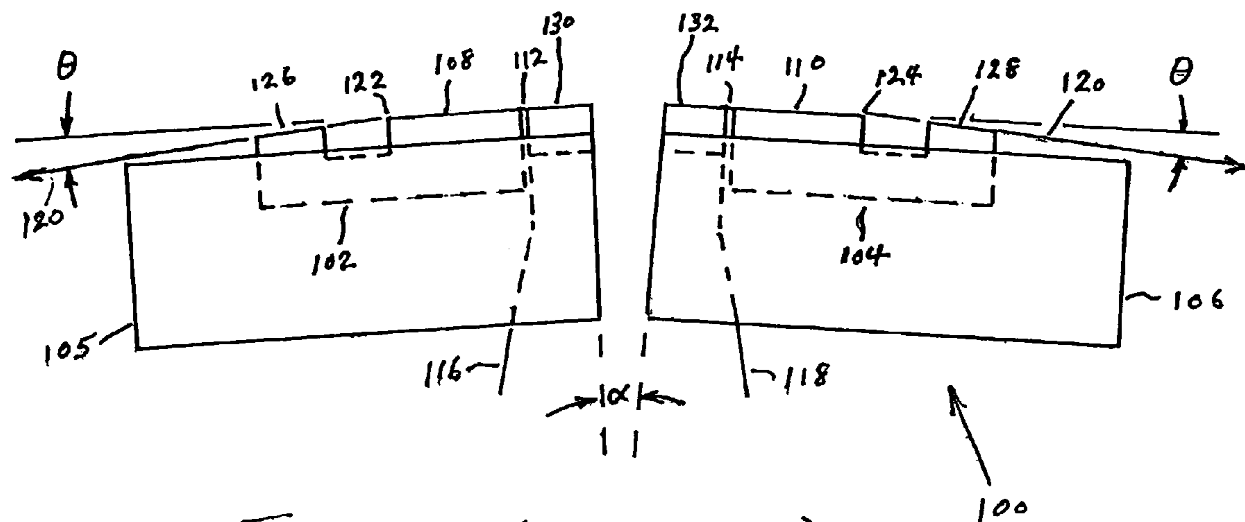
FIG. 1 (PRIOR ART)
