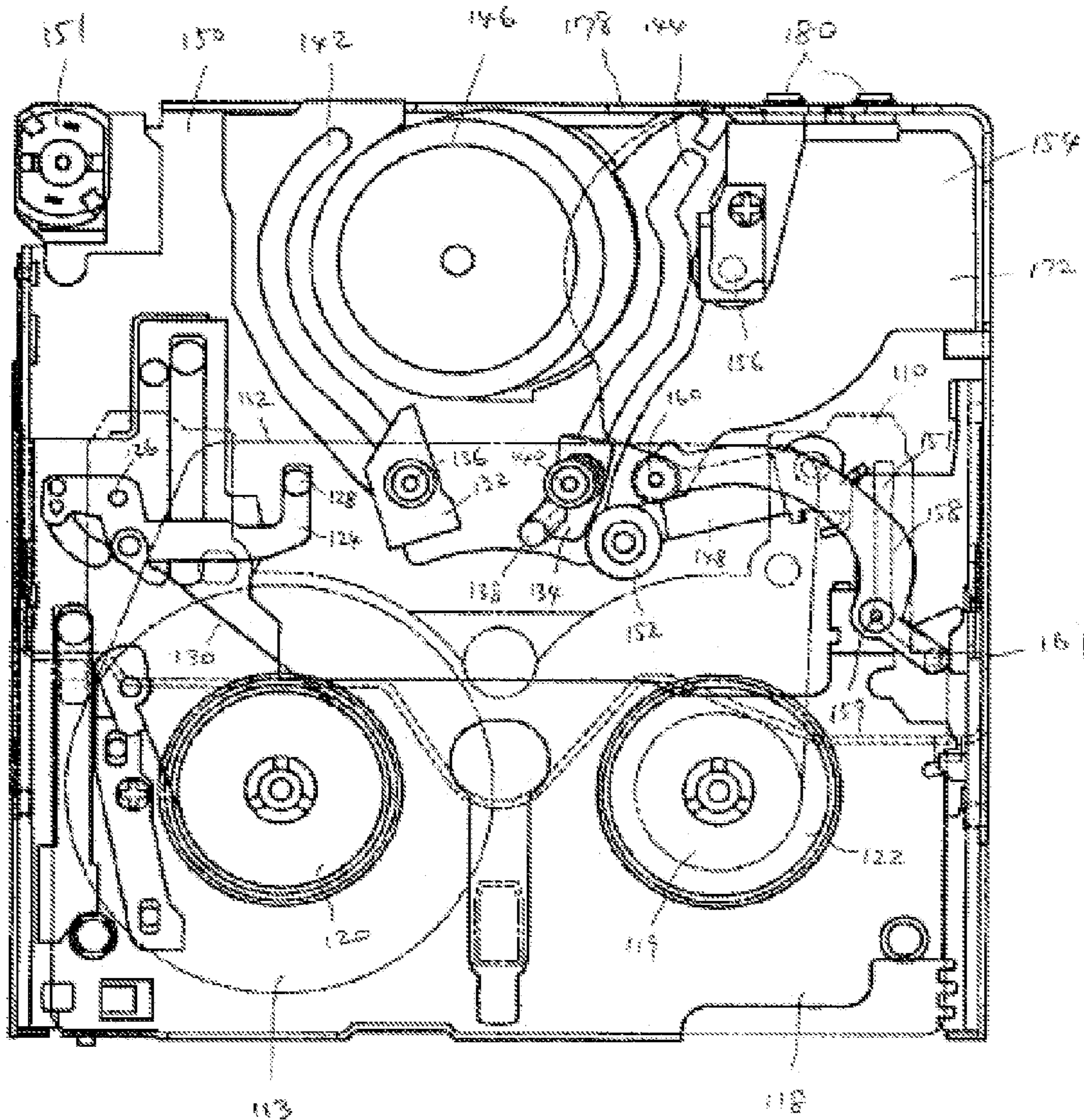
FIG.8 CONVENTIONAL ART
