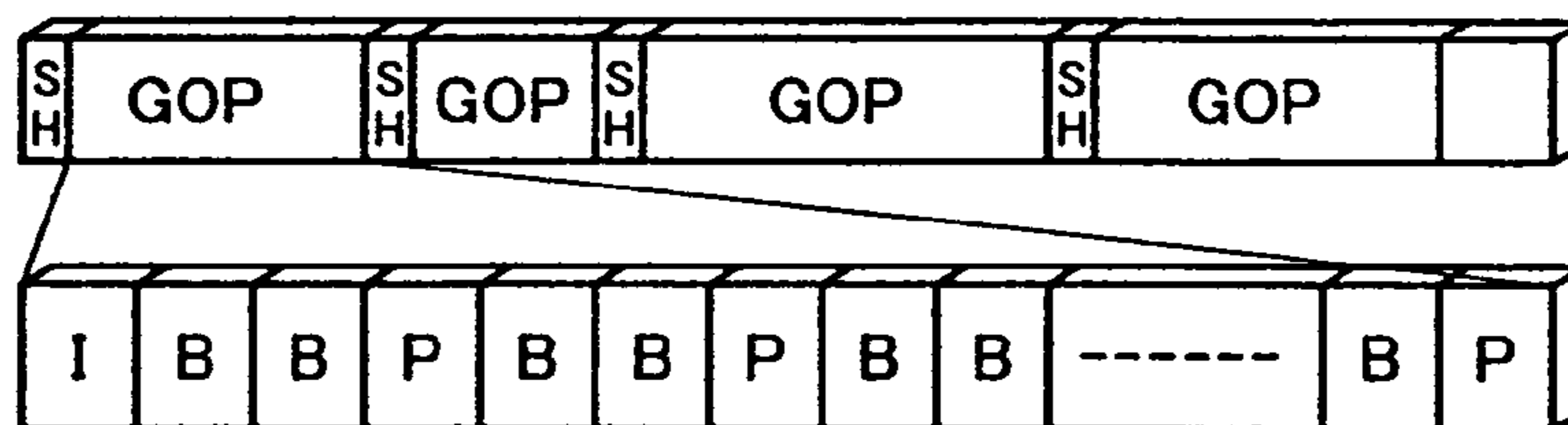
FIG.12 PRIOR ART
