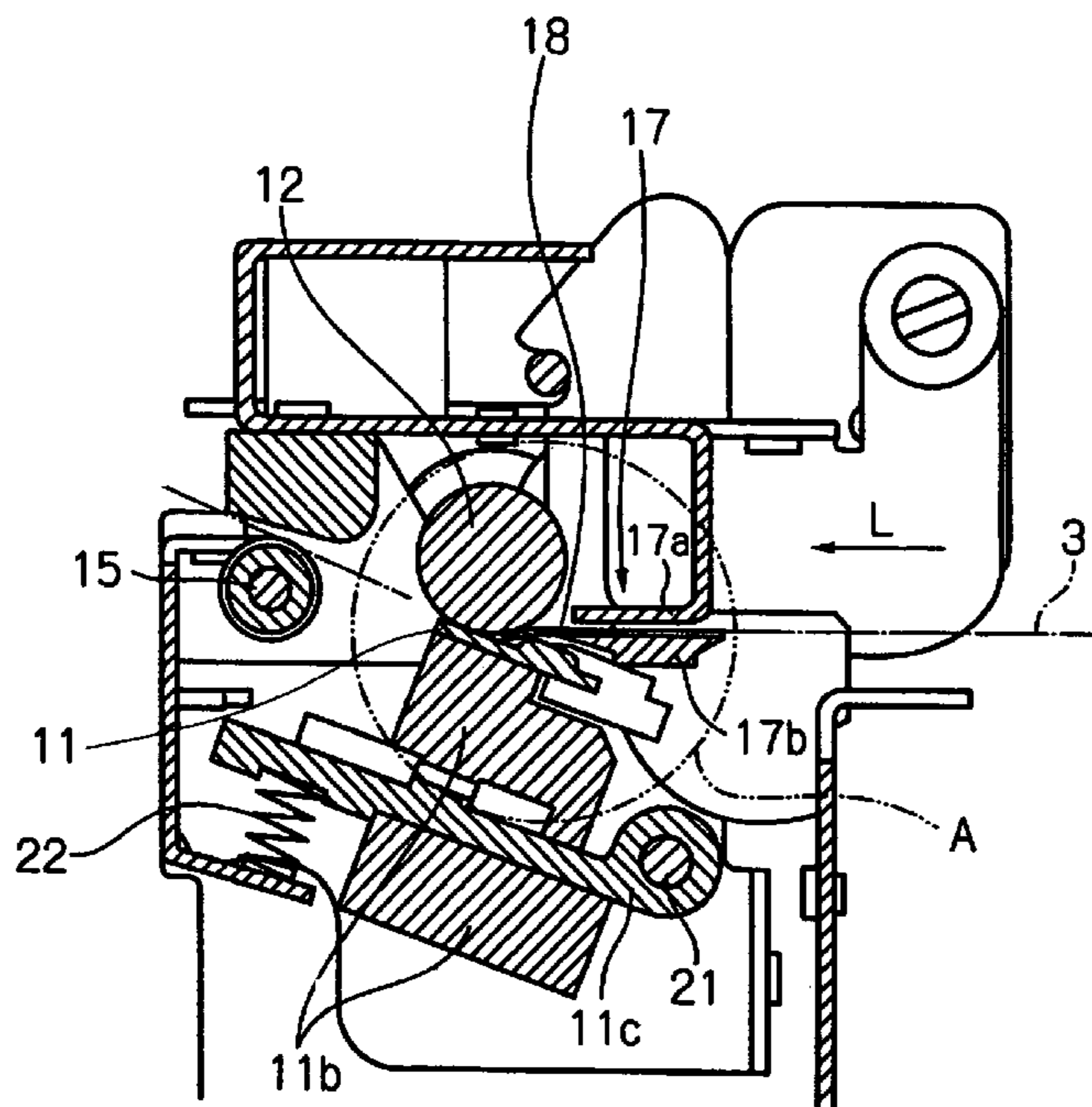
10 THERMAL ACTIVATION DEVICE
