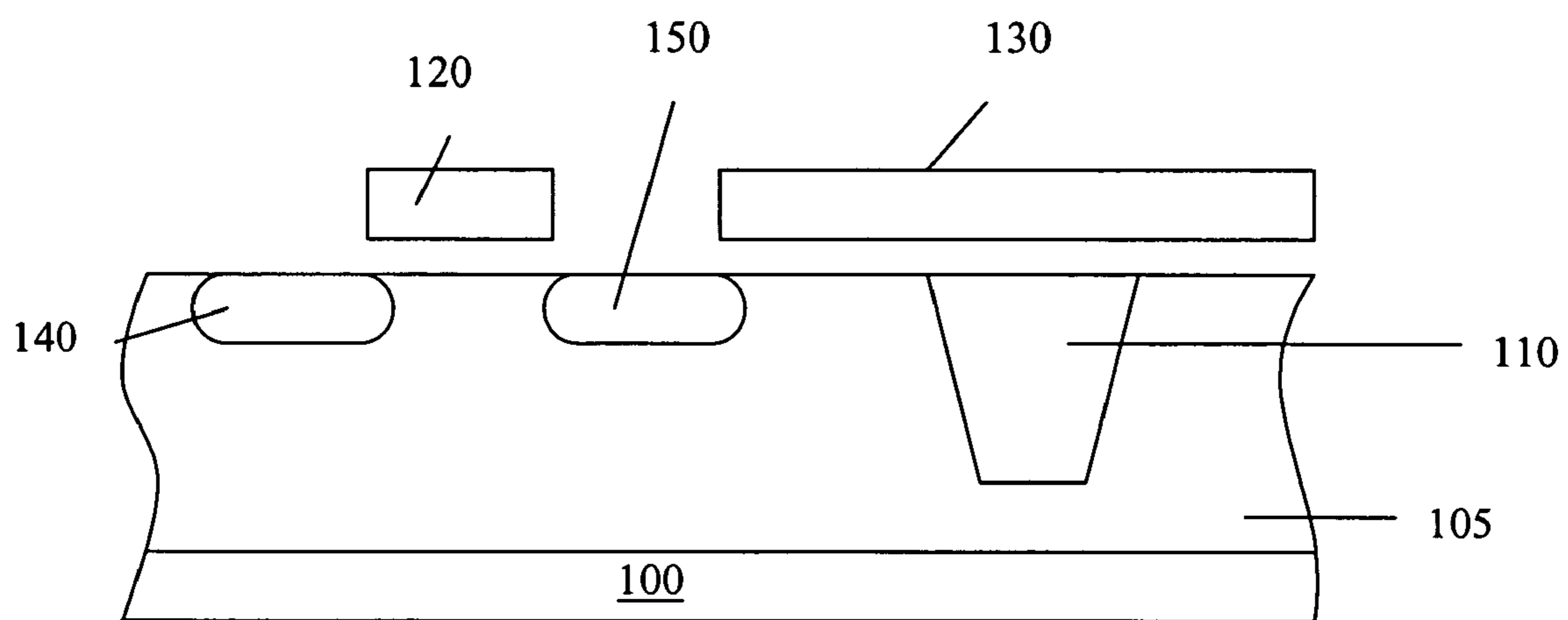
FIG. 1 (PRIOR ART)
