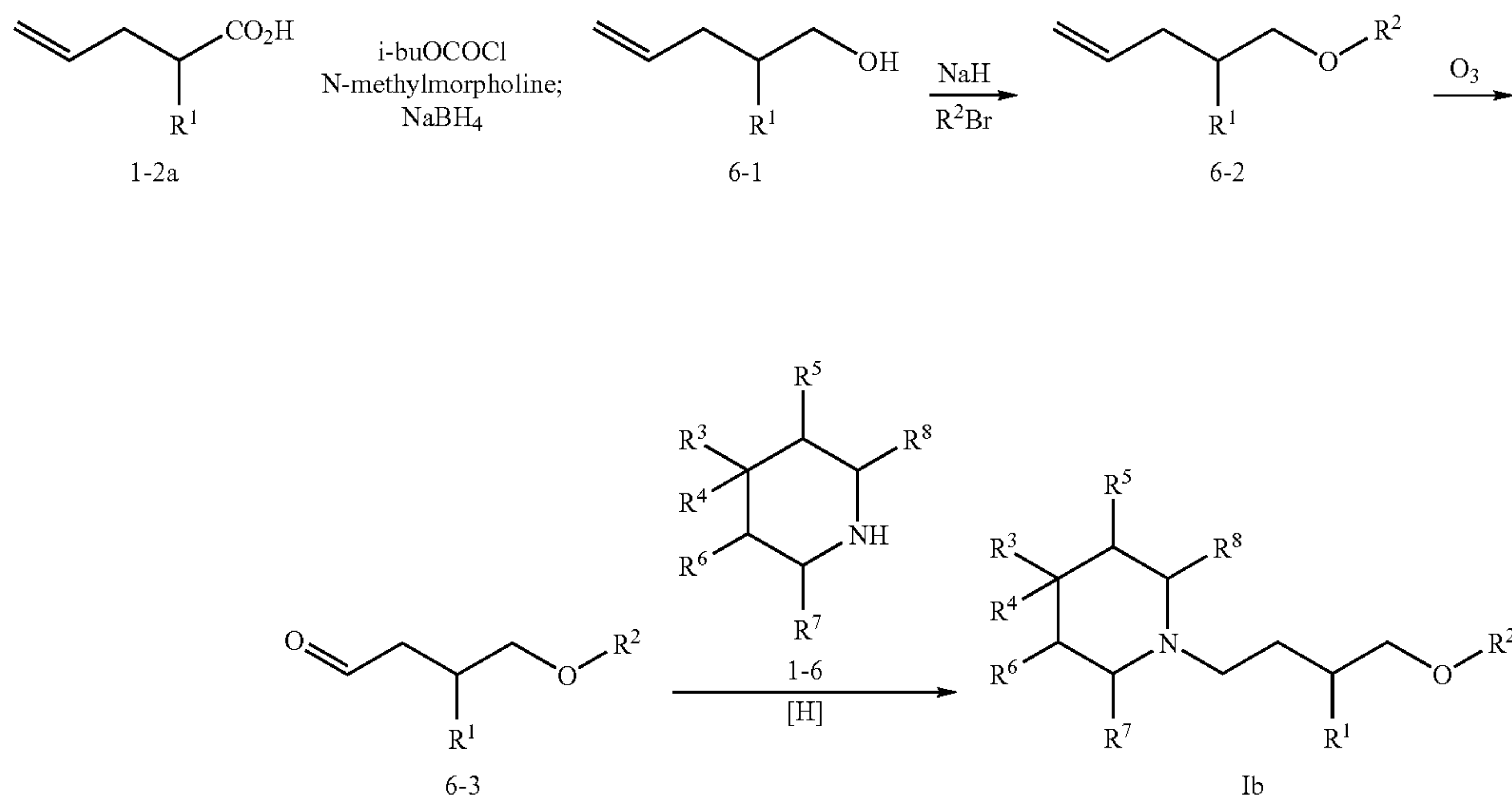
SCHEME 6
