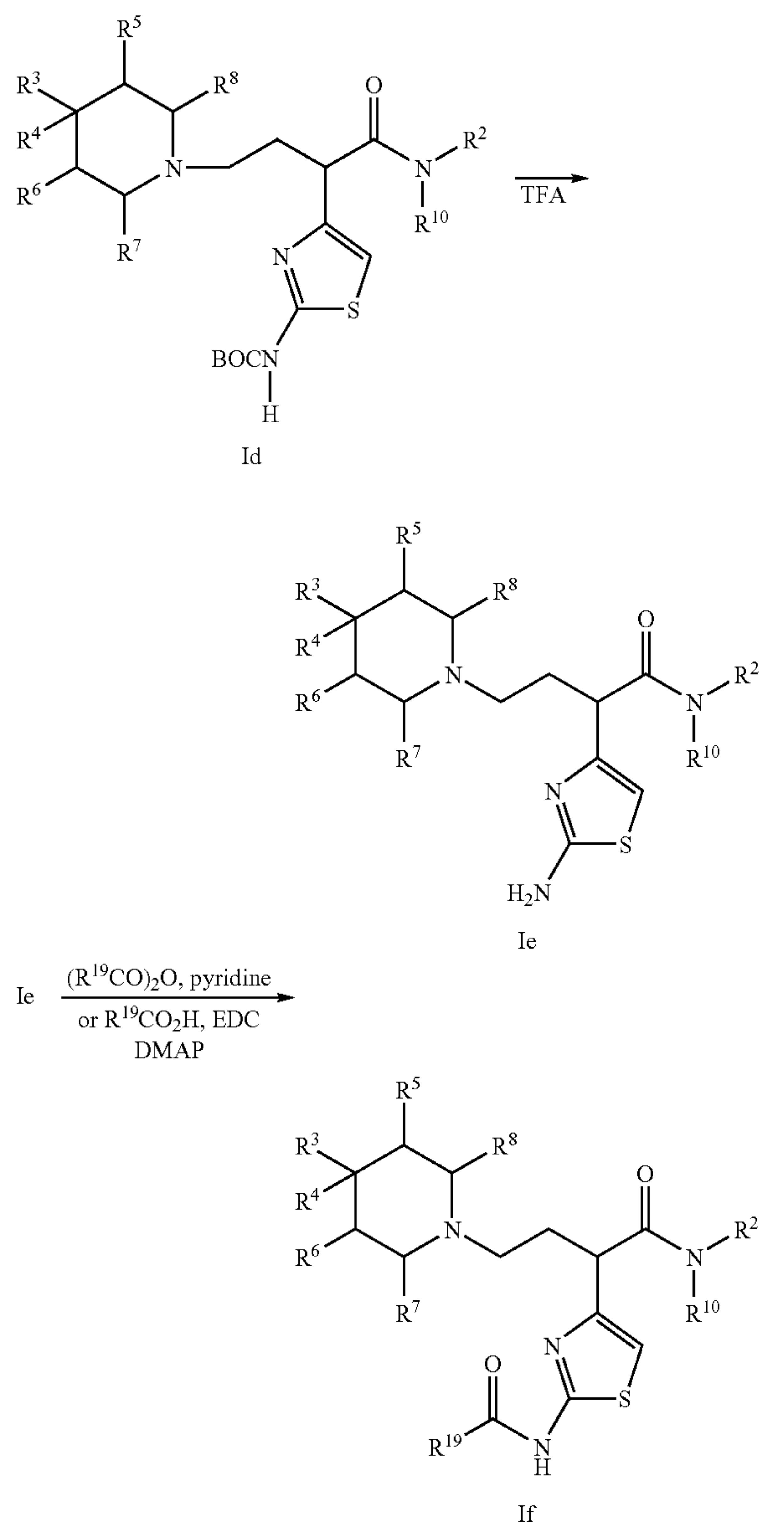
SCHEME 7
