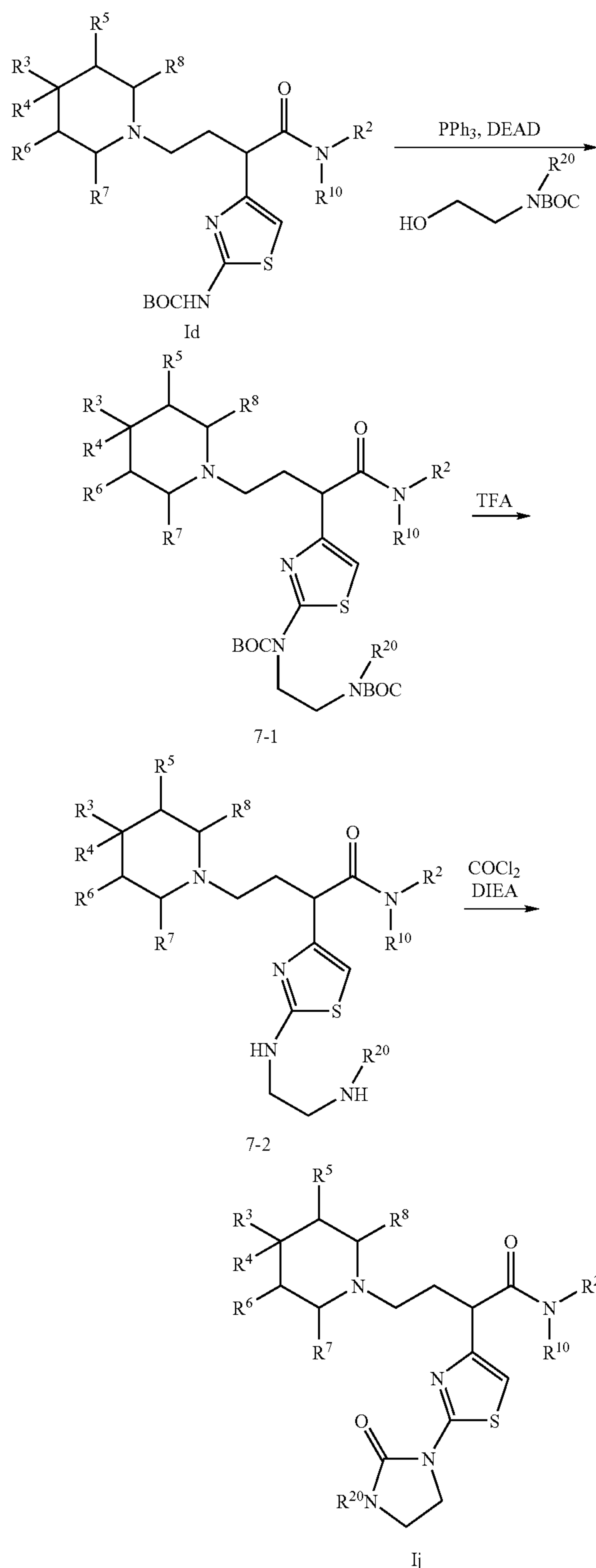
SCHEME 7A
