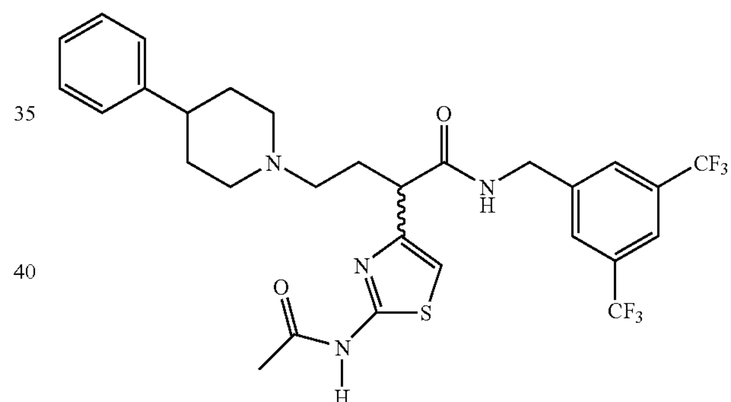
2-(2-Acetylamino-thiazol-4-yl)-N-(3,5-bis-trifluoromethyl-benzyl)-4-(phenyl-4'-piperidine)-1'-butyramide
