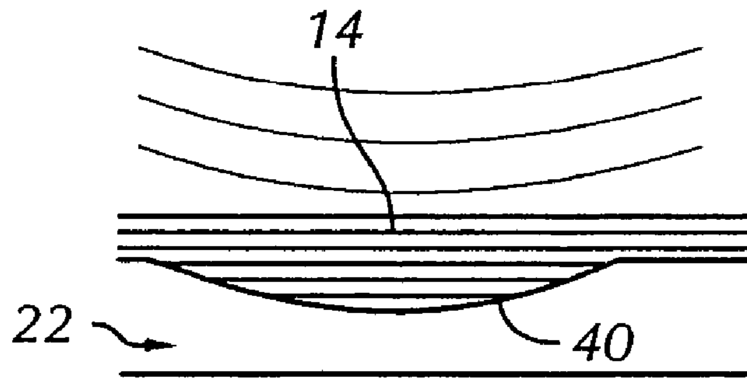
FIG. 8 (Prior Art)
