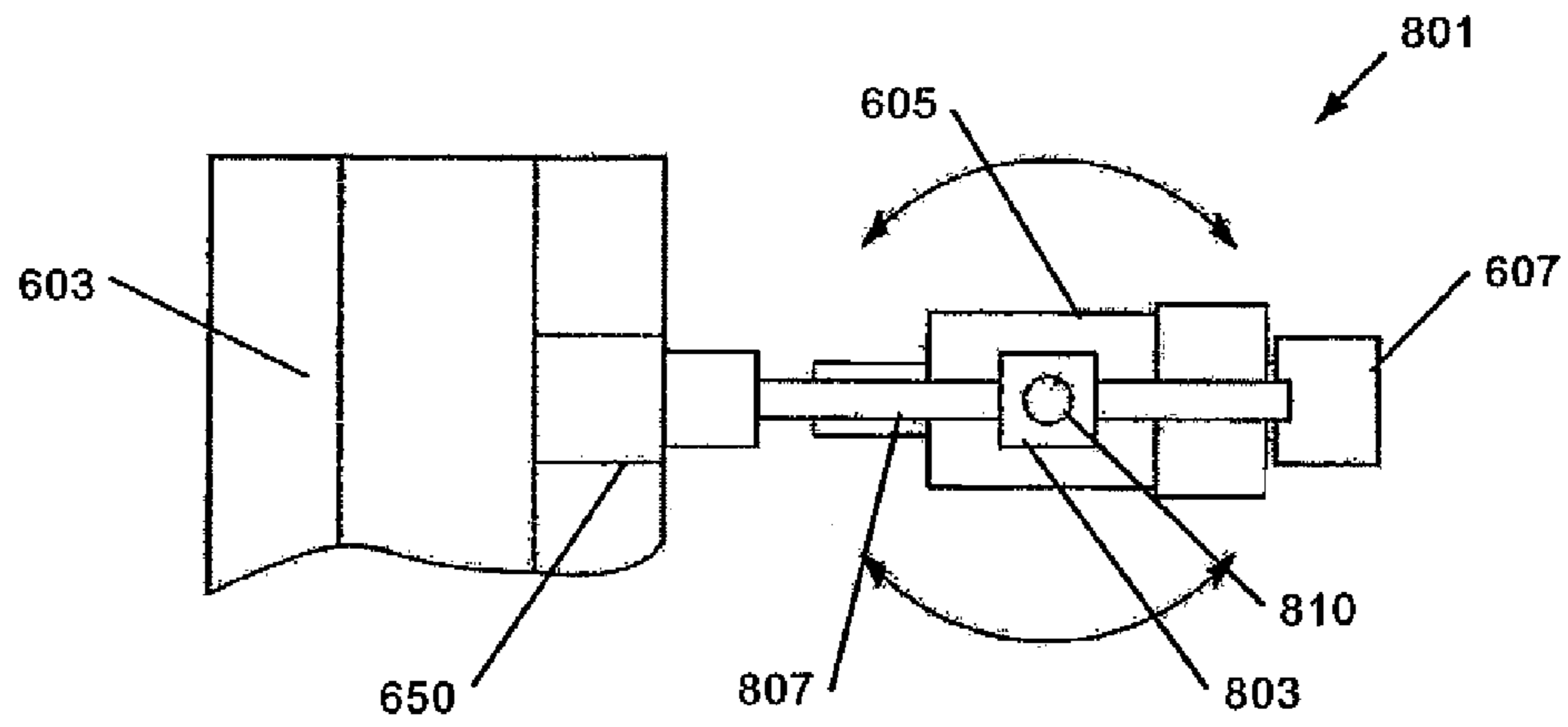
Figure 28D
