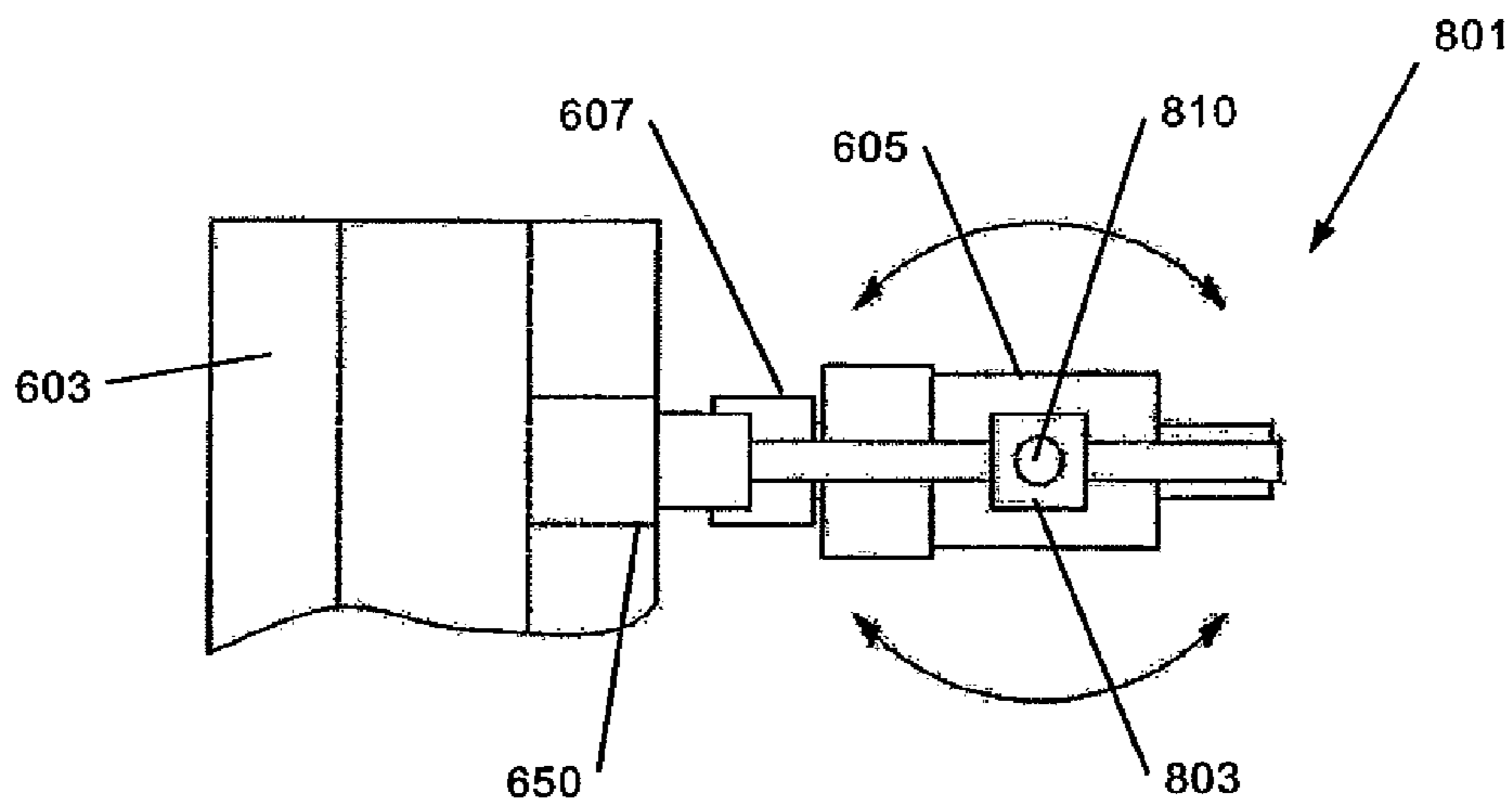
Figure 28B
