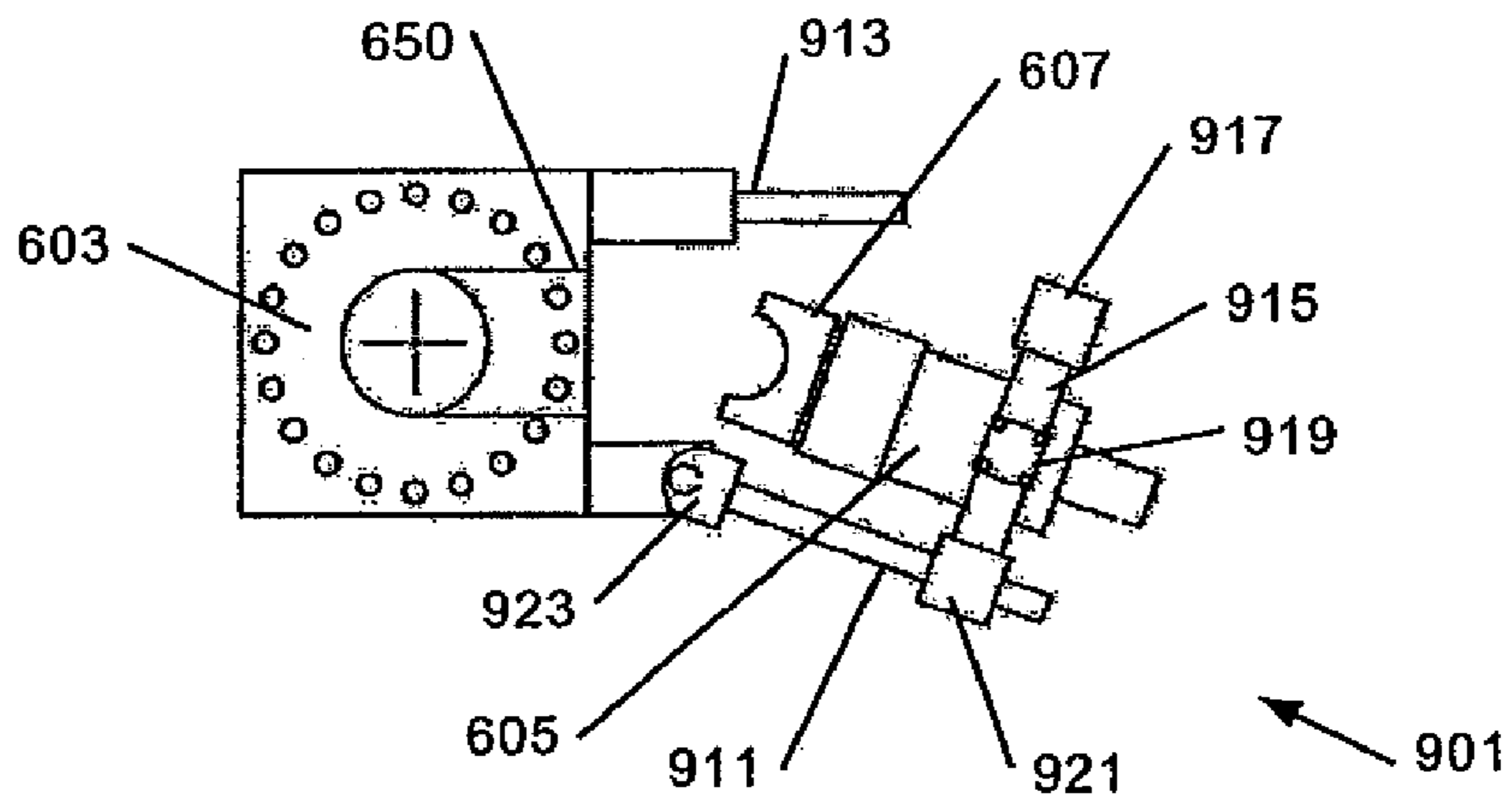
Figure 29D
