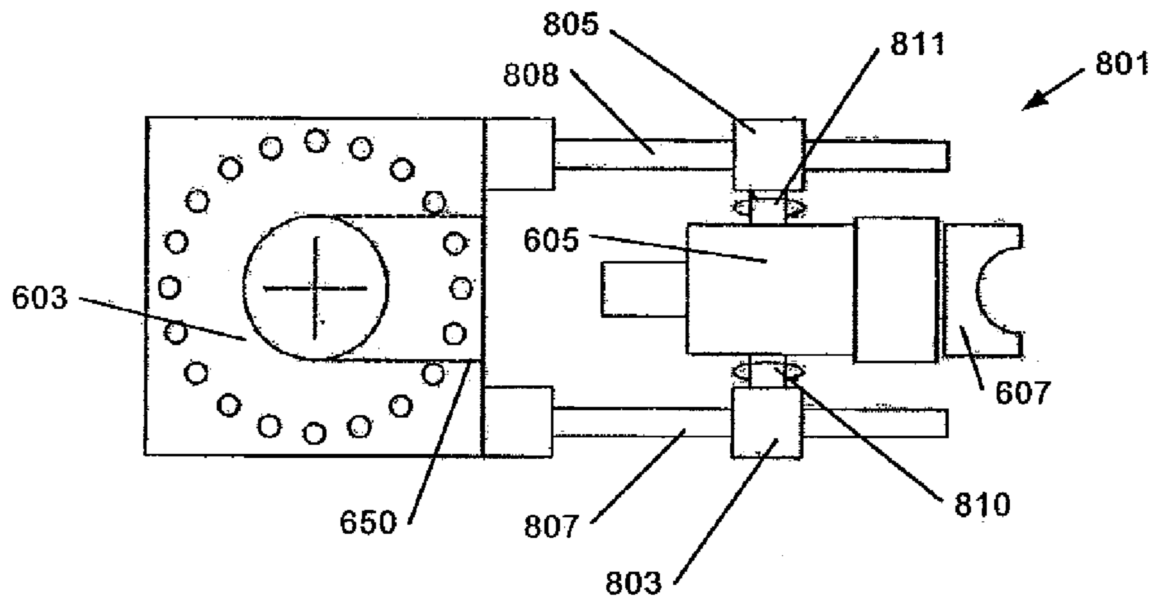
Figure 28C
