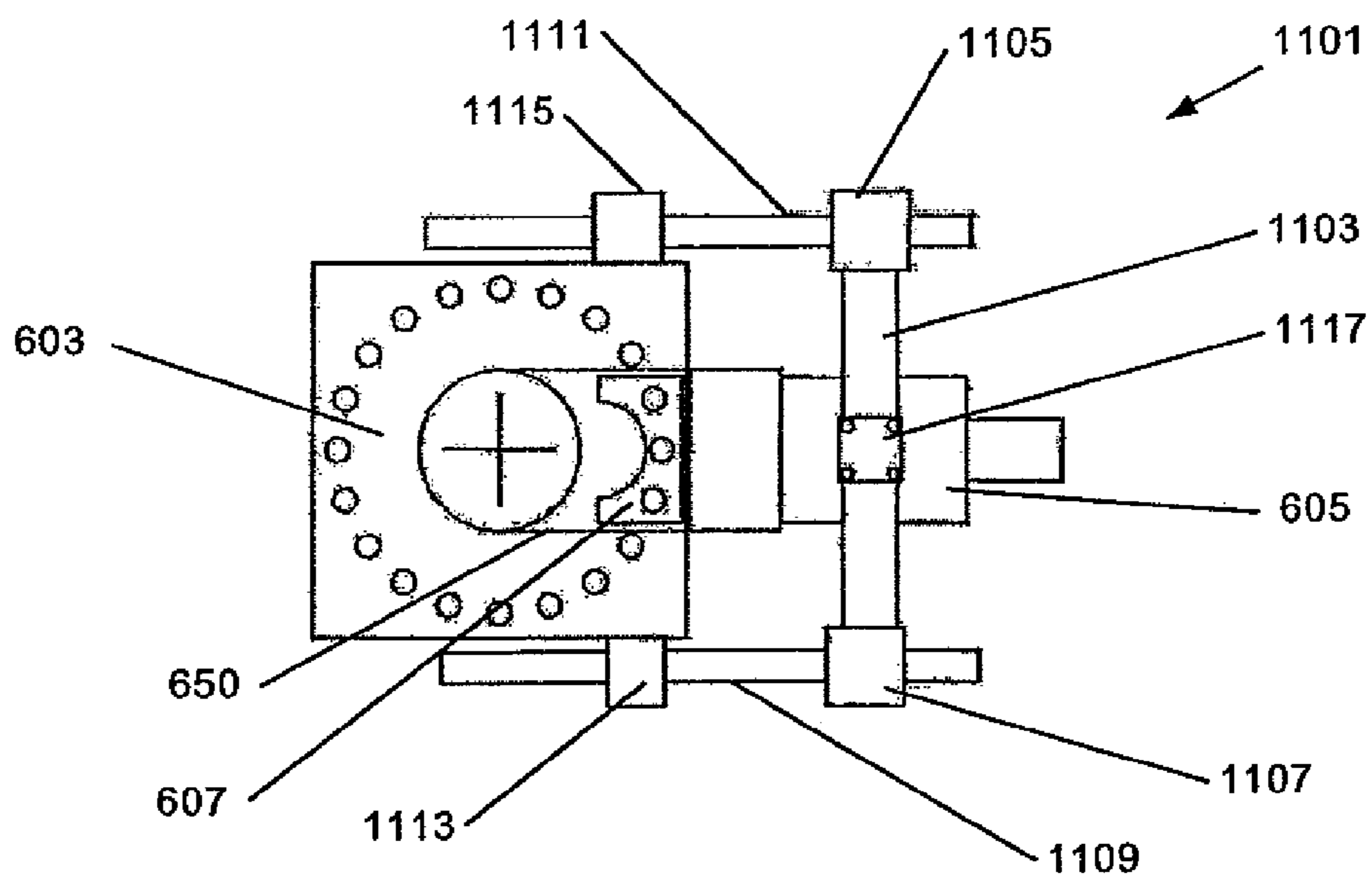
Figure 31B
