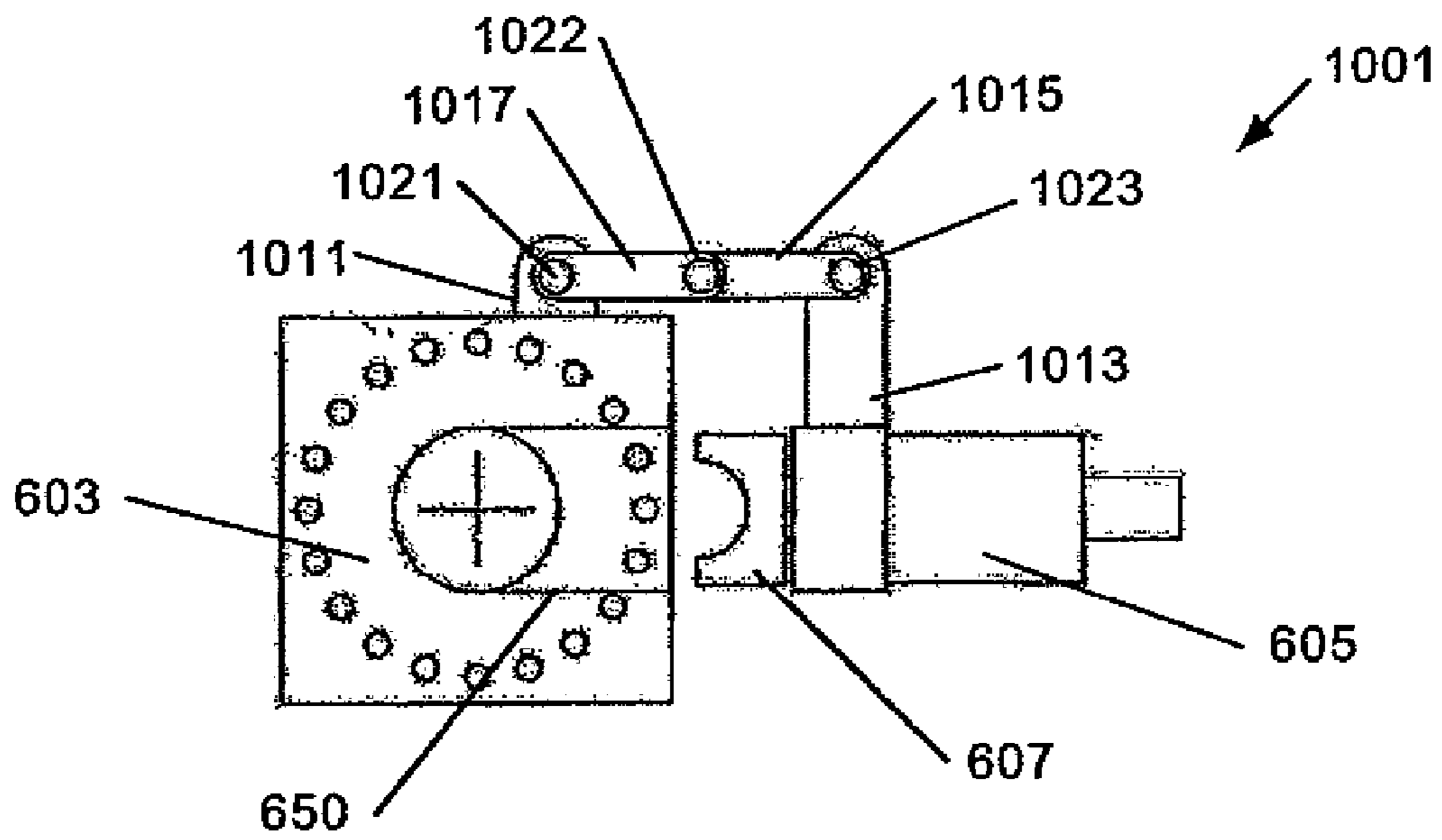
Figure 30B
