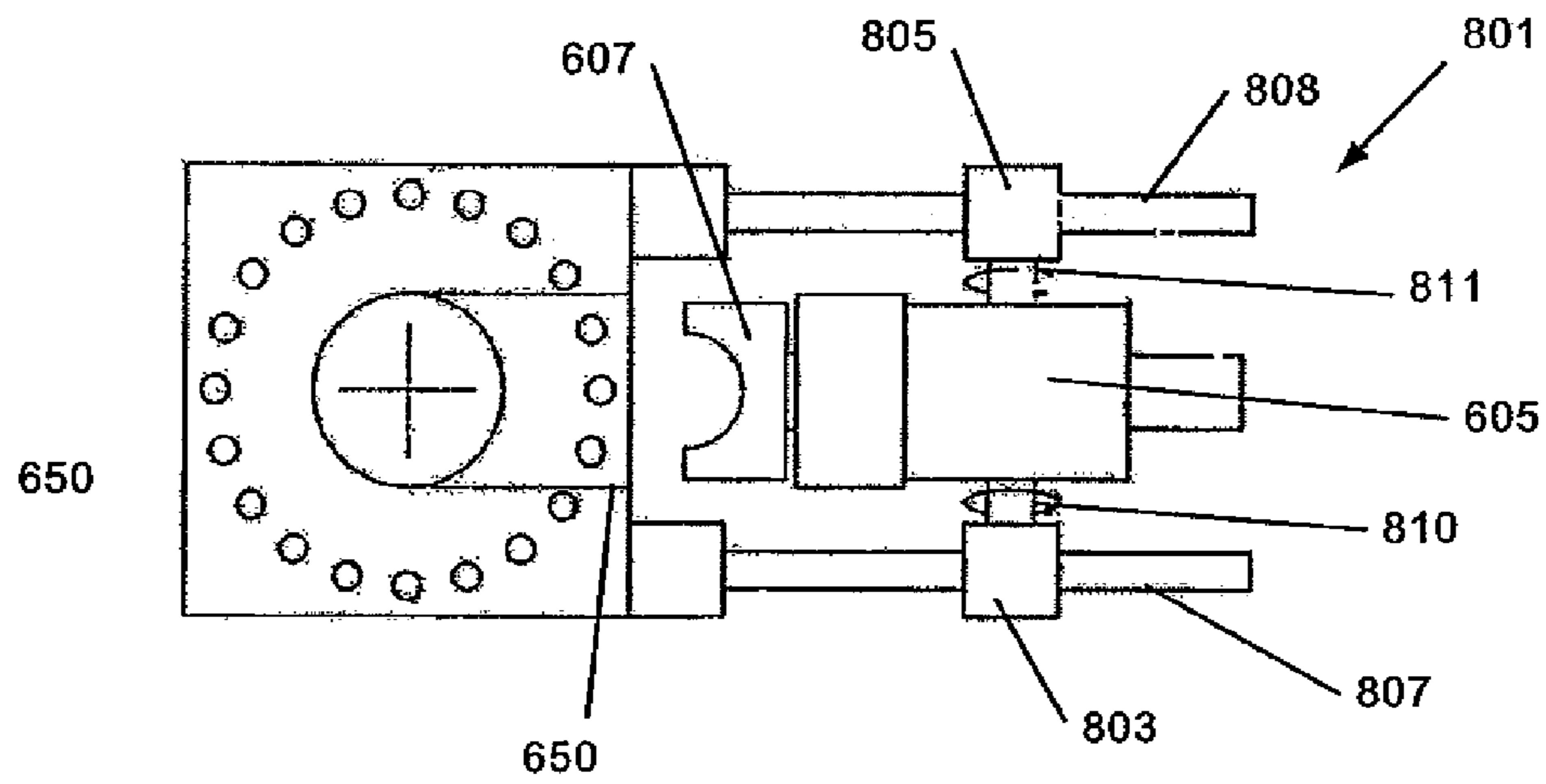
Figure 28A
