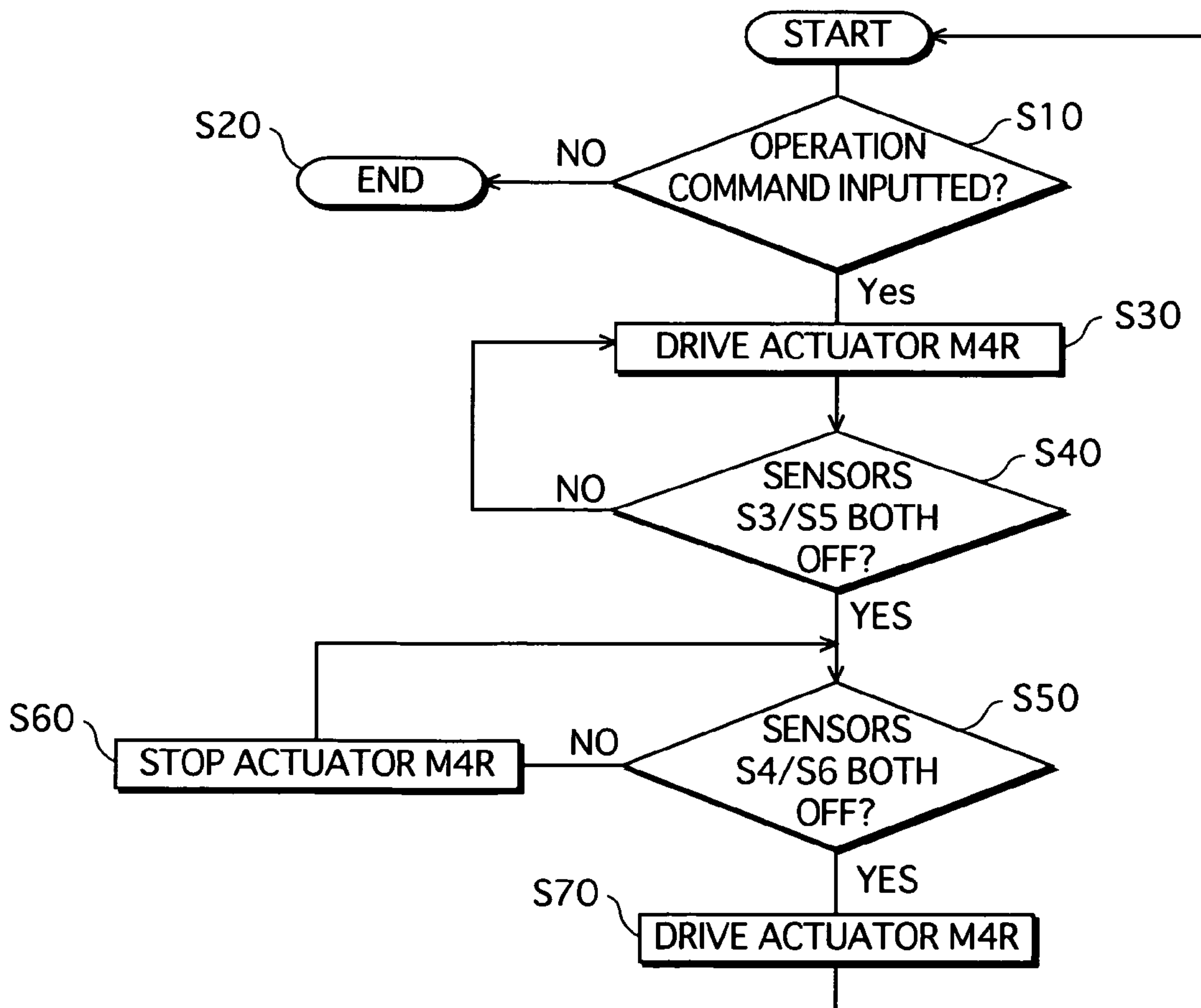
HORIZONTAL SYNC FLOWCHART
