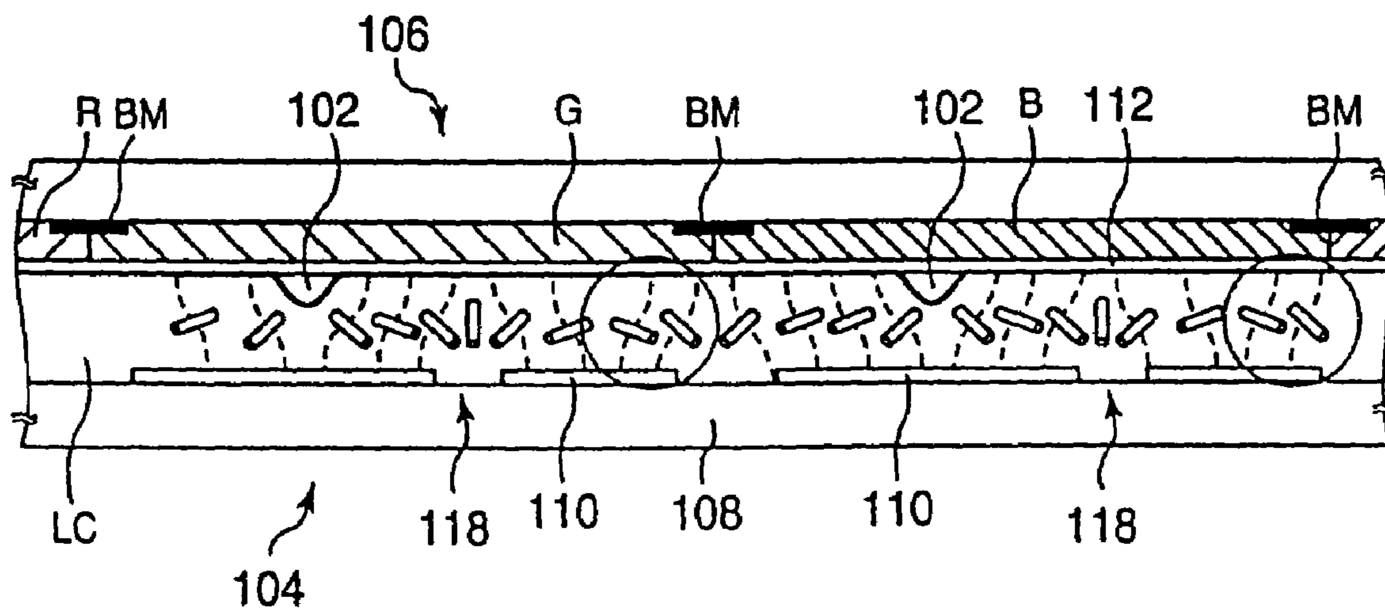
PRIOR ART FIG.40
