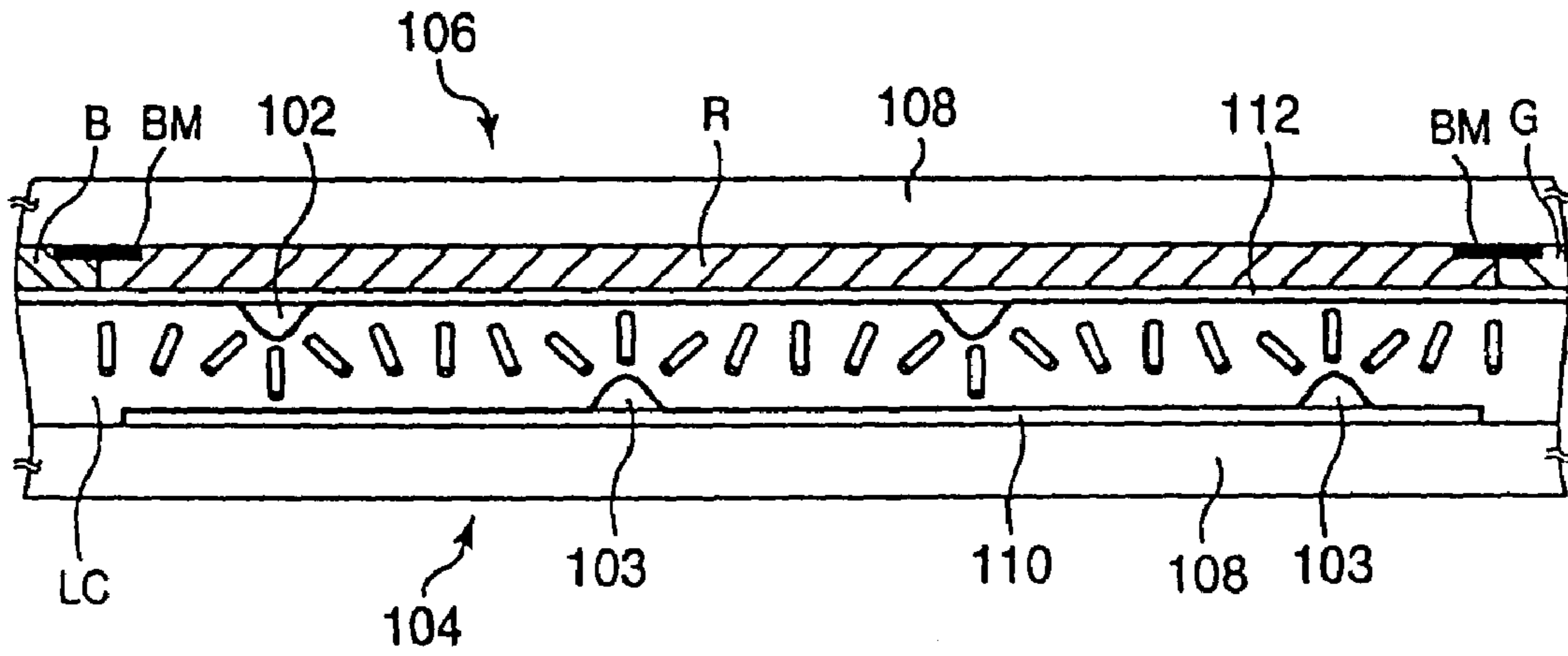
PRIOR ART FIG.37
