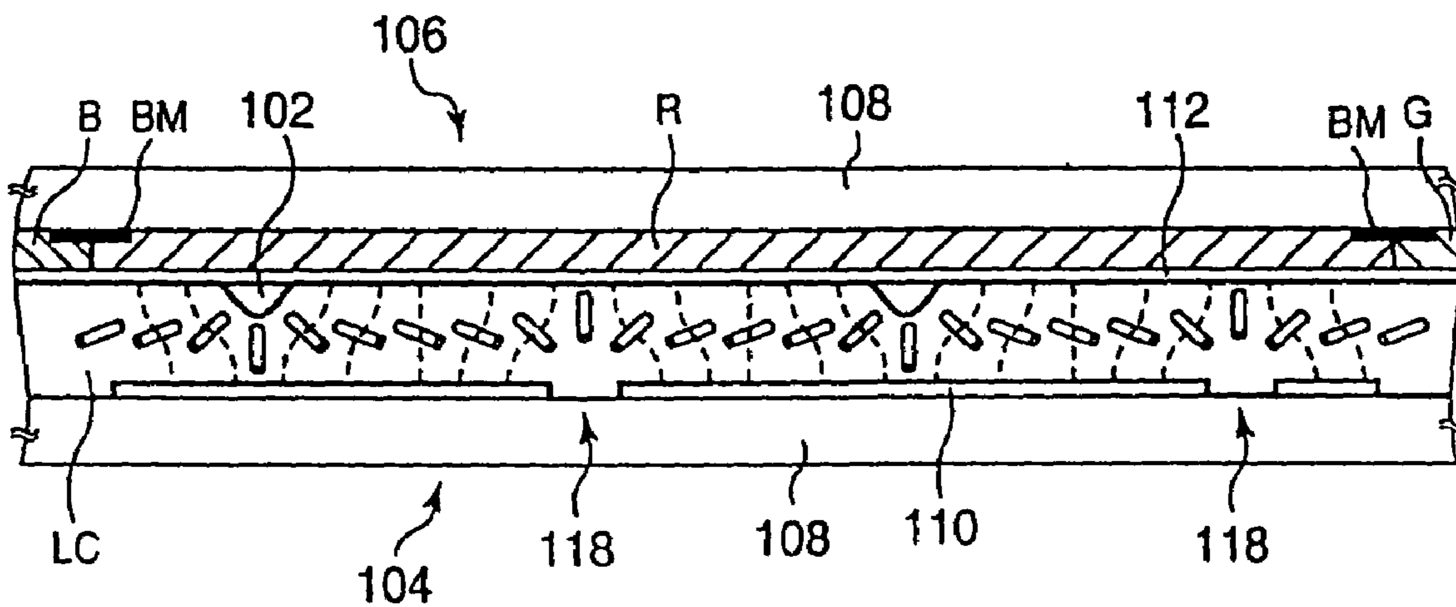
PRIOR ART FIG.39
