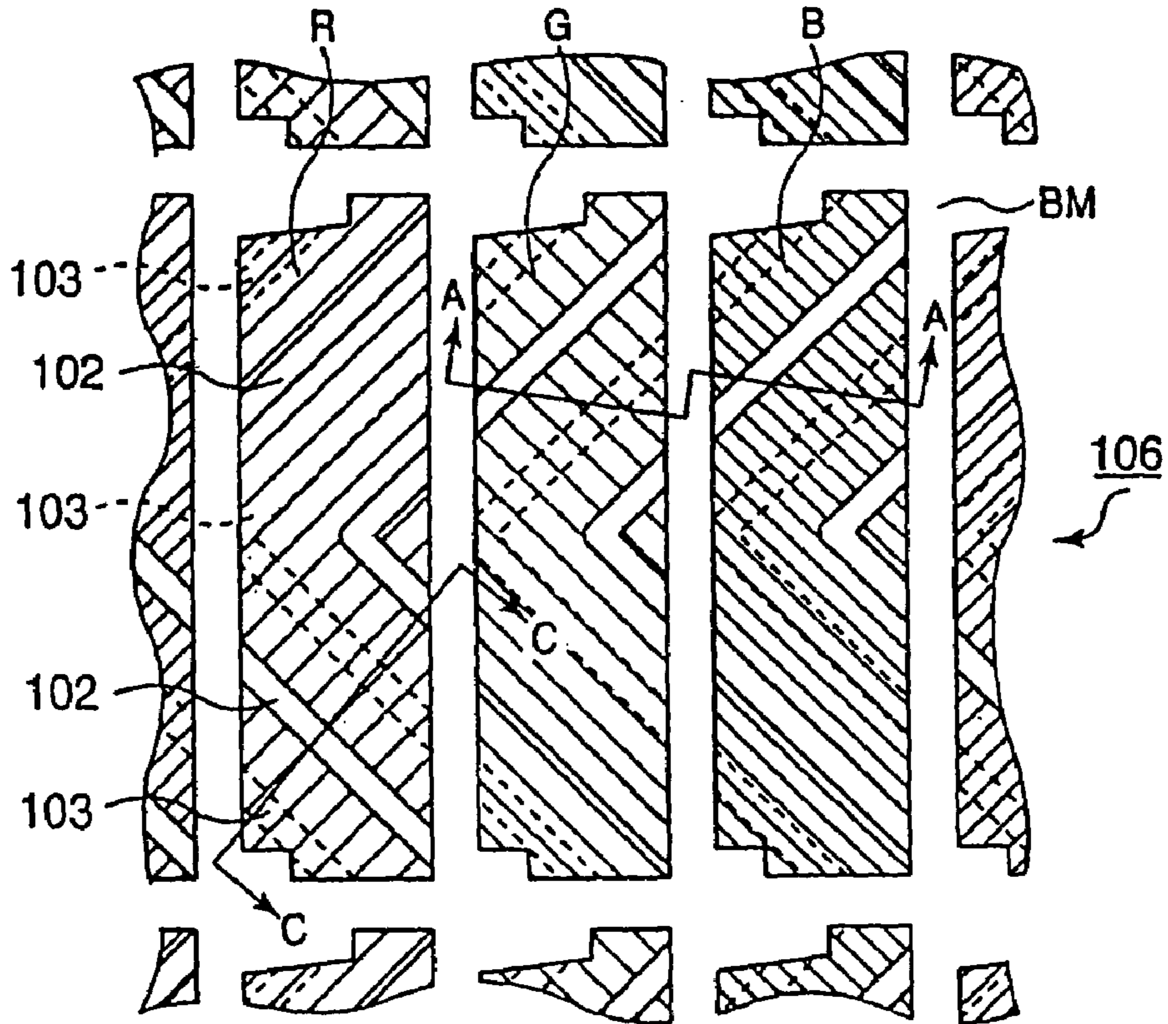
PRIOR ART FIG.35
