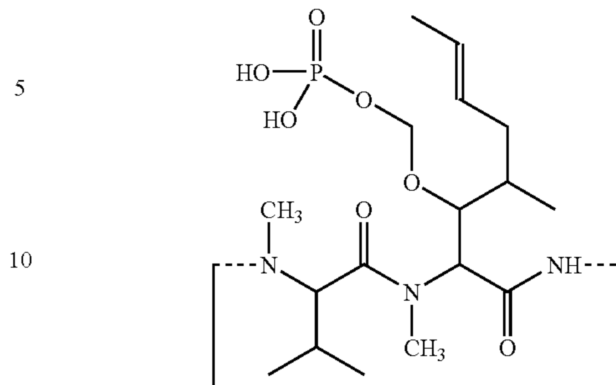
Cyclosporin A
