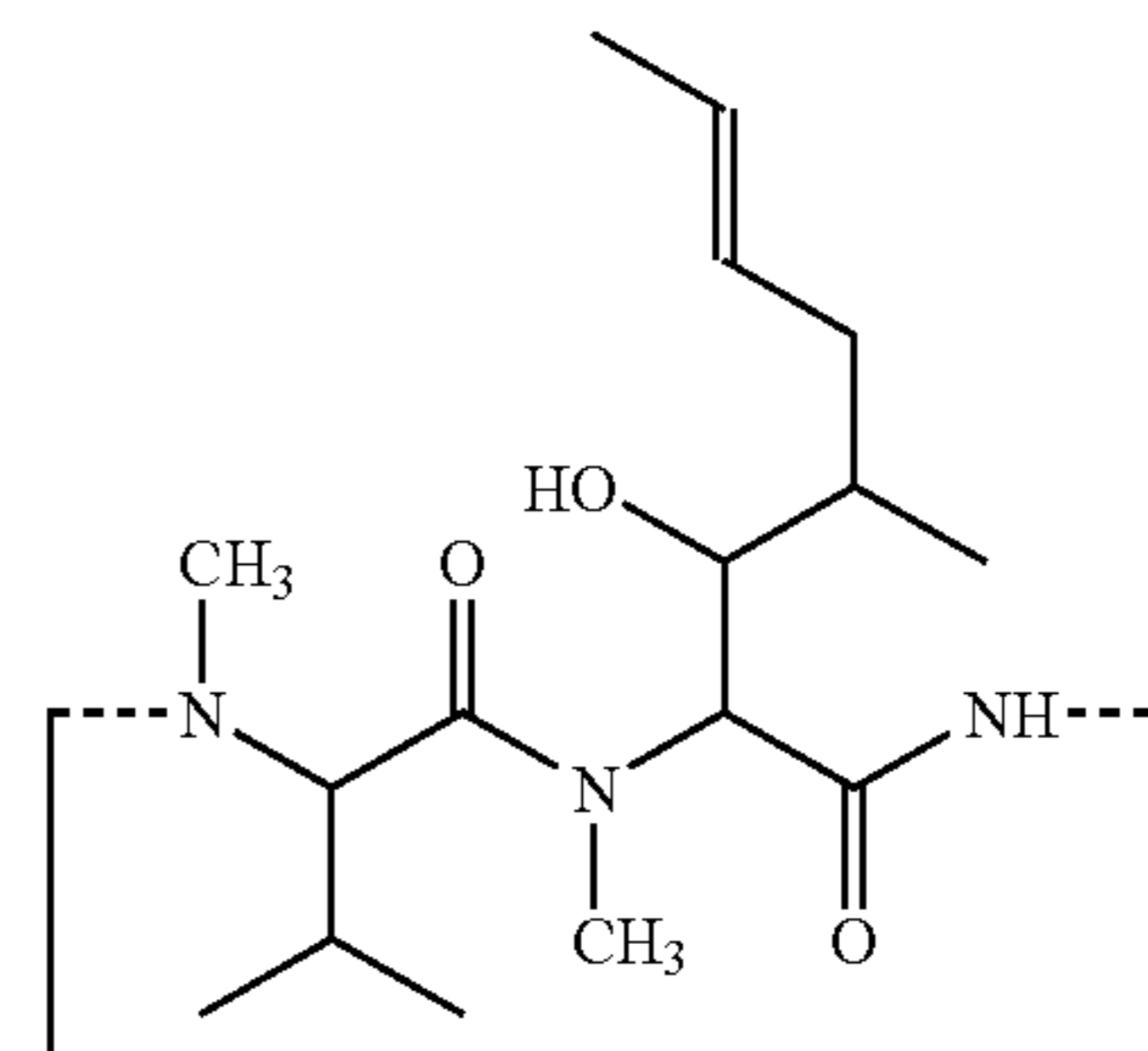
Cyclosporin A
