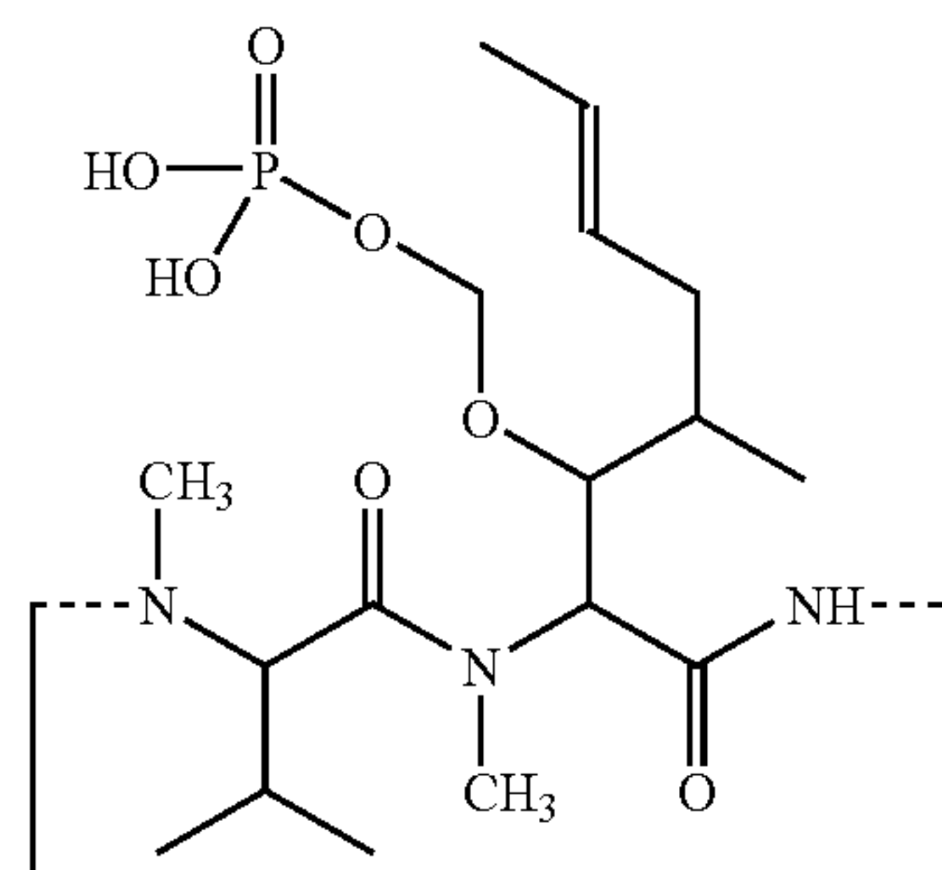
Cyclosporin A
