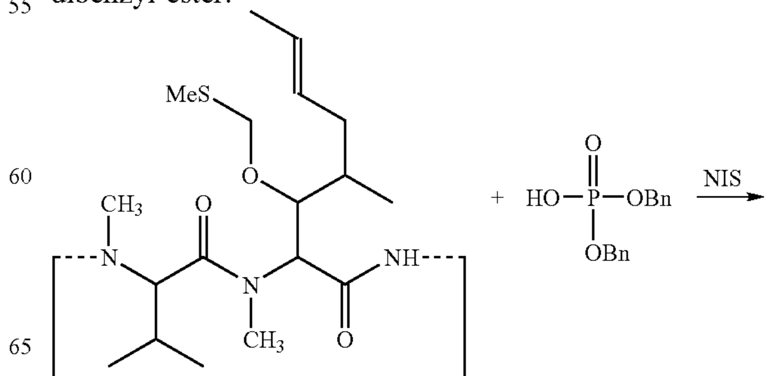
Cyclosporin A
