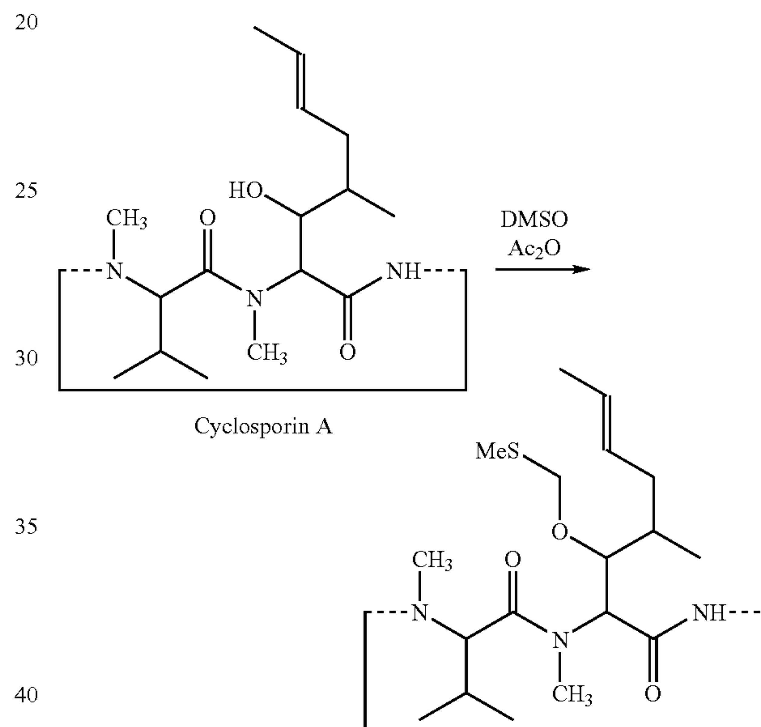
Cyclosporin A
