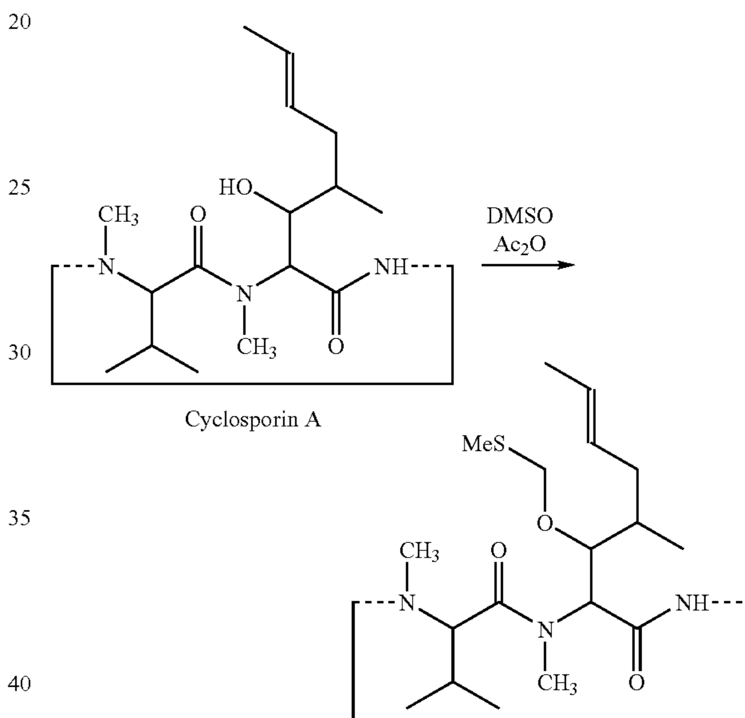
Cyclosporin A
