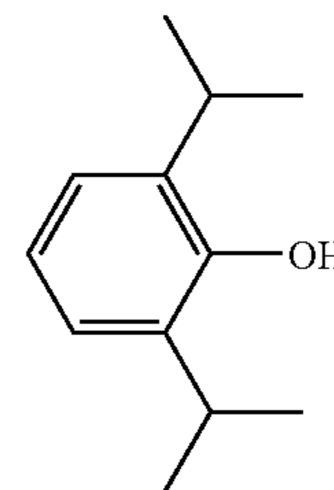
Propofol (2, 6-diisopropylphenol)
