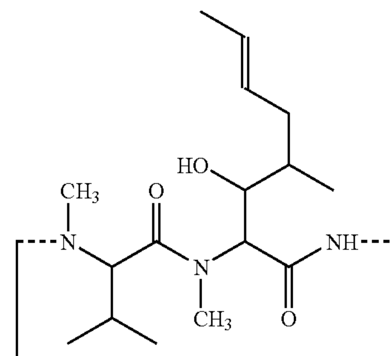
Cyclosporin A
