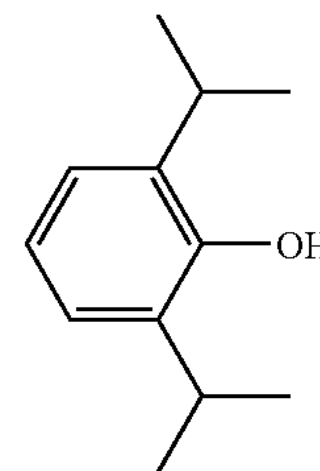
Propofol (2, 6-diisopropylphenol)
