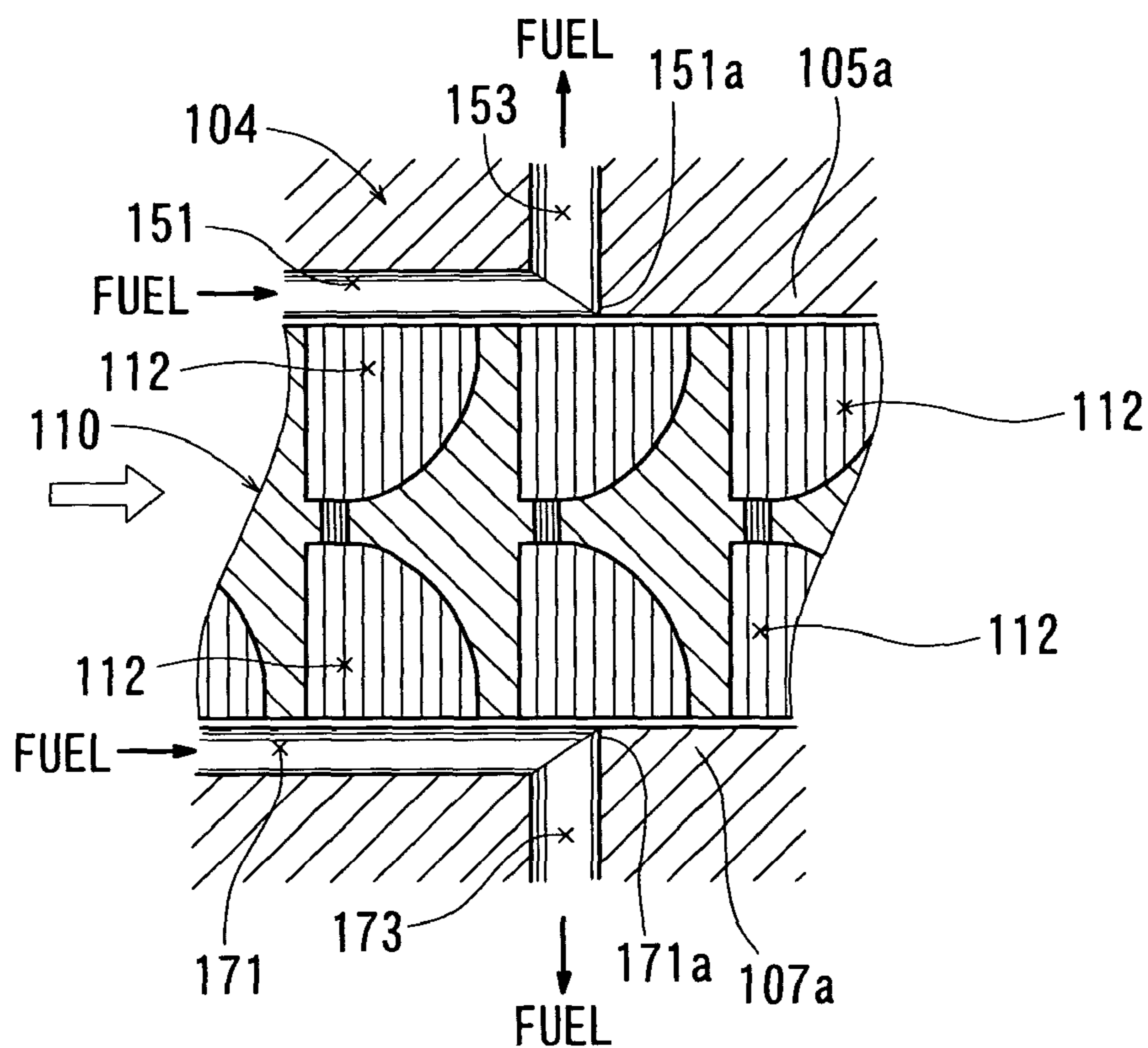
FIG. 24 PRIOR ART
