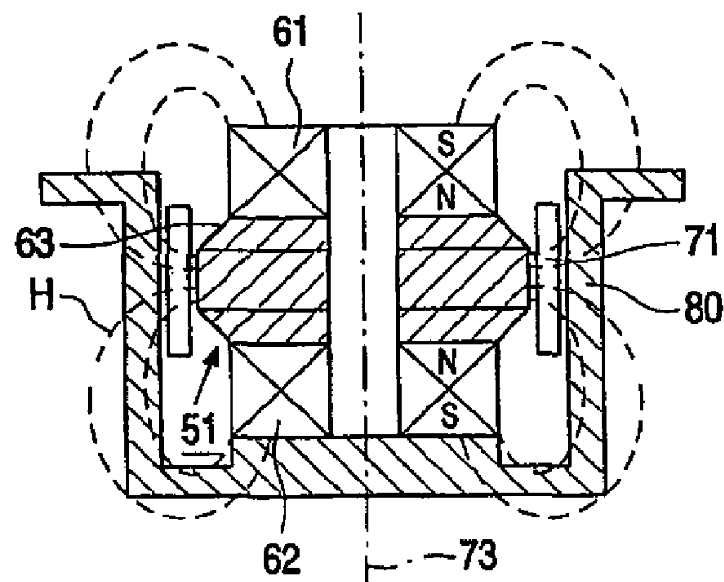
FIG. 3 [PRIOR ART]
