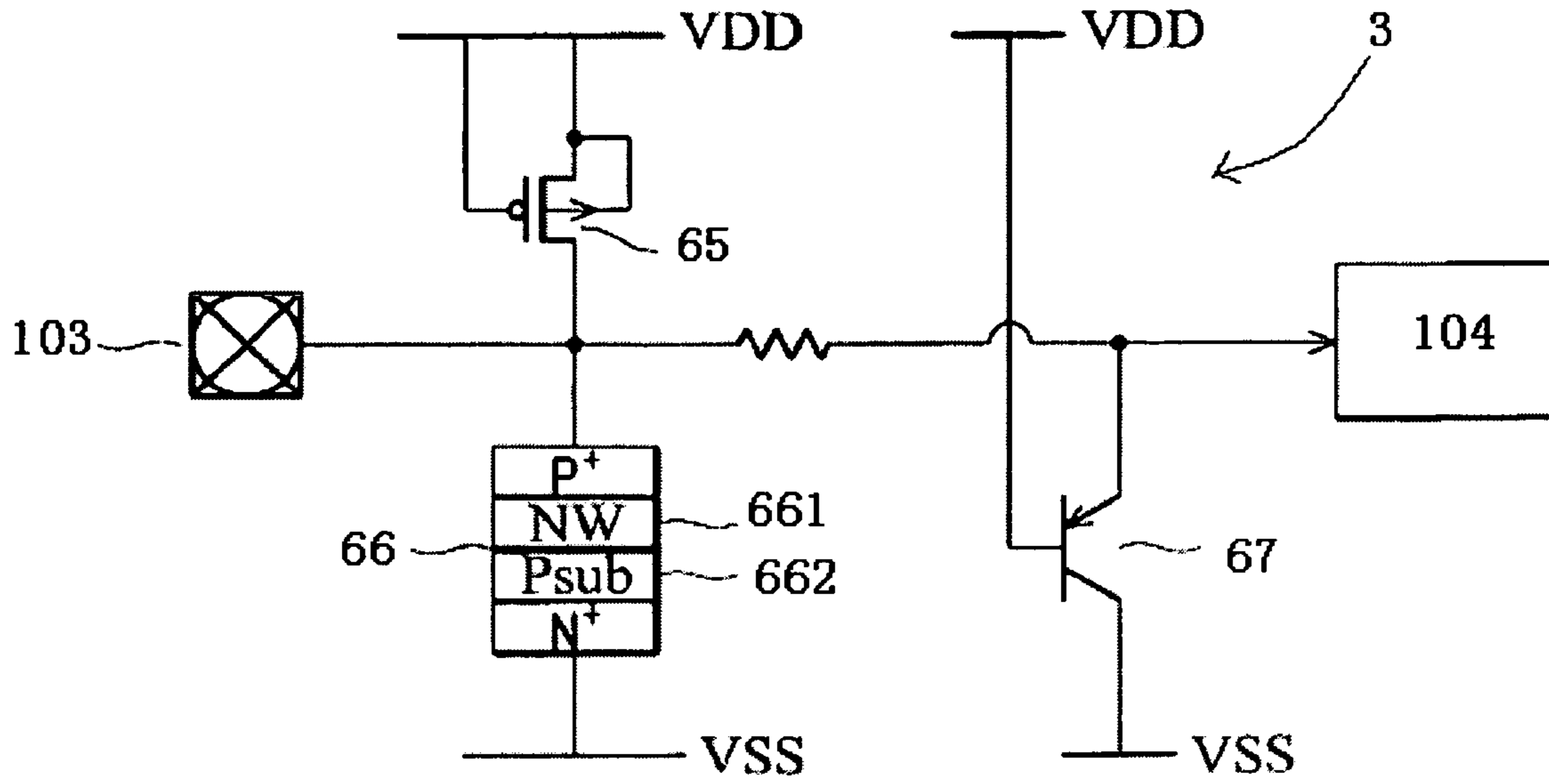
FIG.3 (Prior art)
