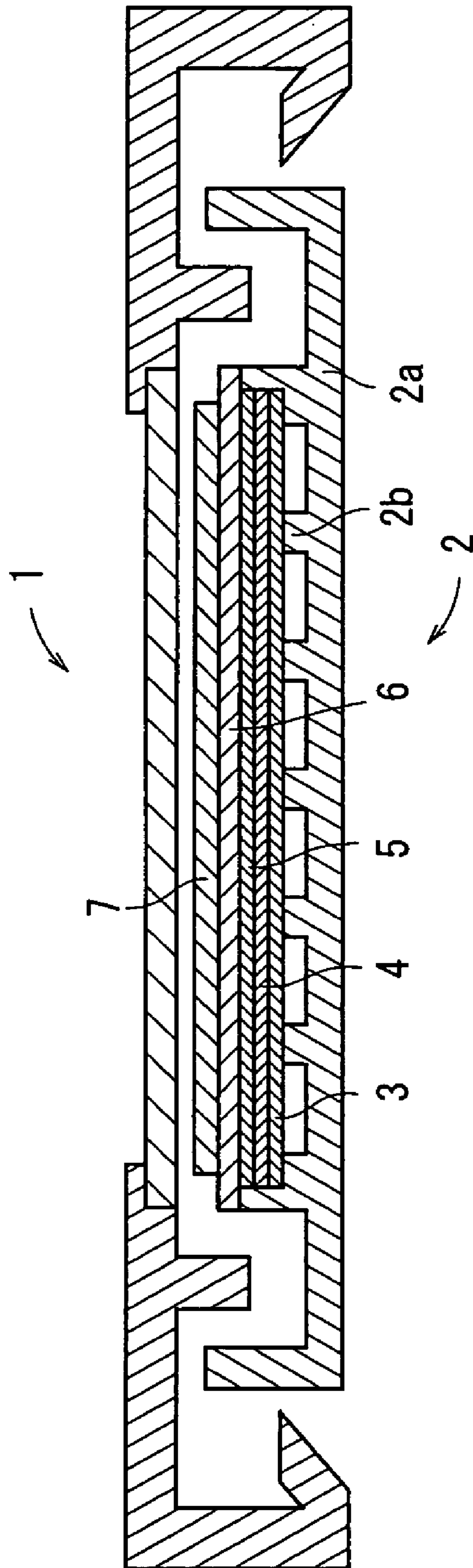
FIG. 14 PRIOR ART
