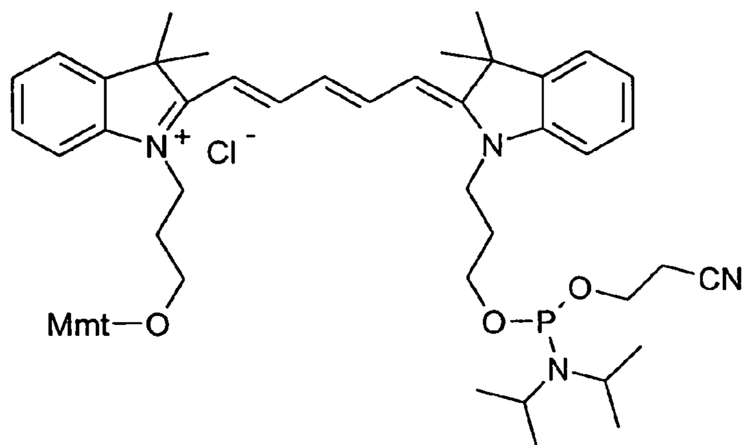
Cyanin-5 phosphoramidite 11
