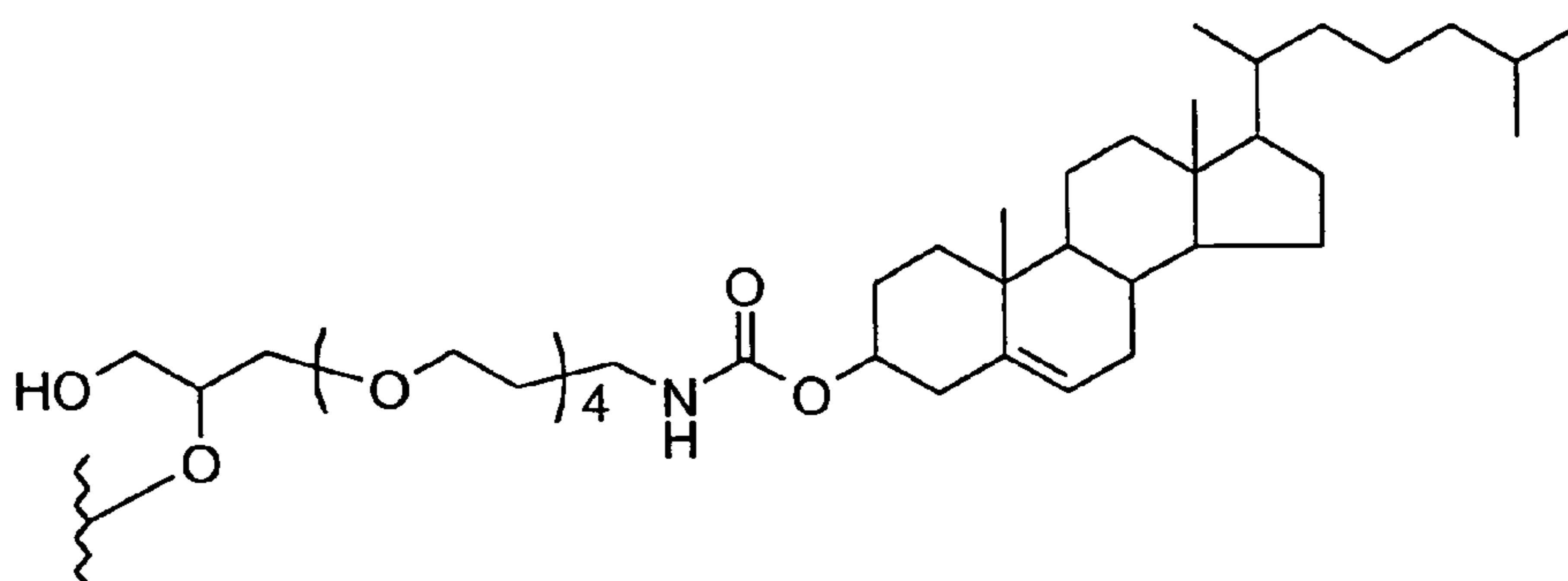
Cholesterol
