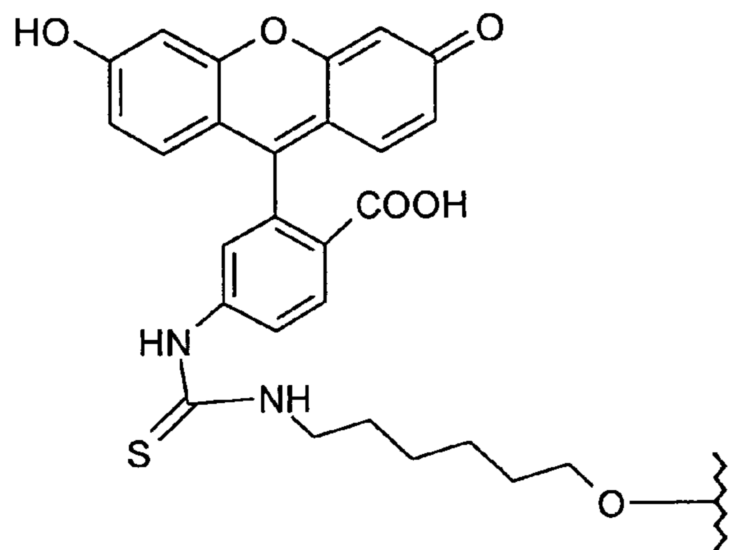
Fluorescein (Thiourea)
