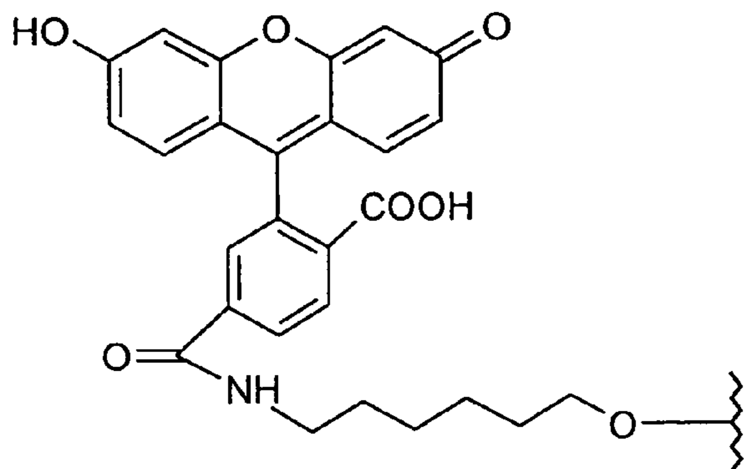
Fluorescein (Amide)
