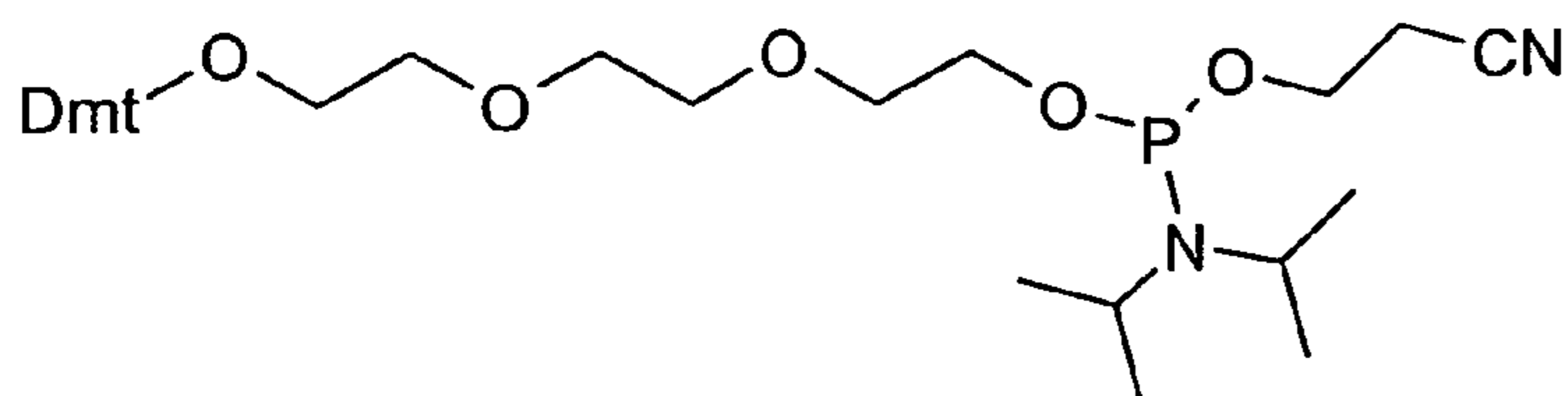
Spacer-9 phosphoramidite 8
