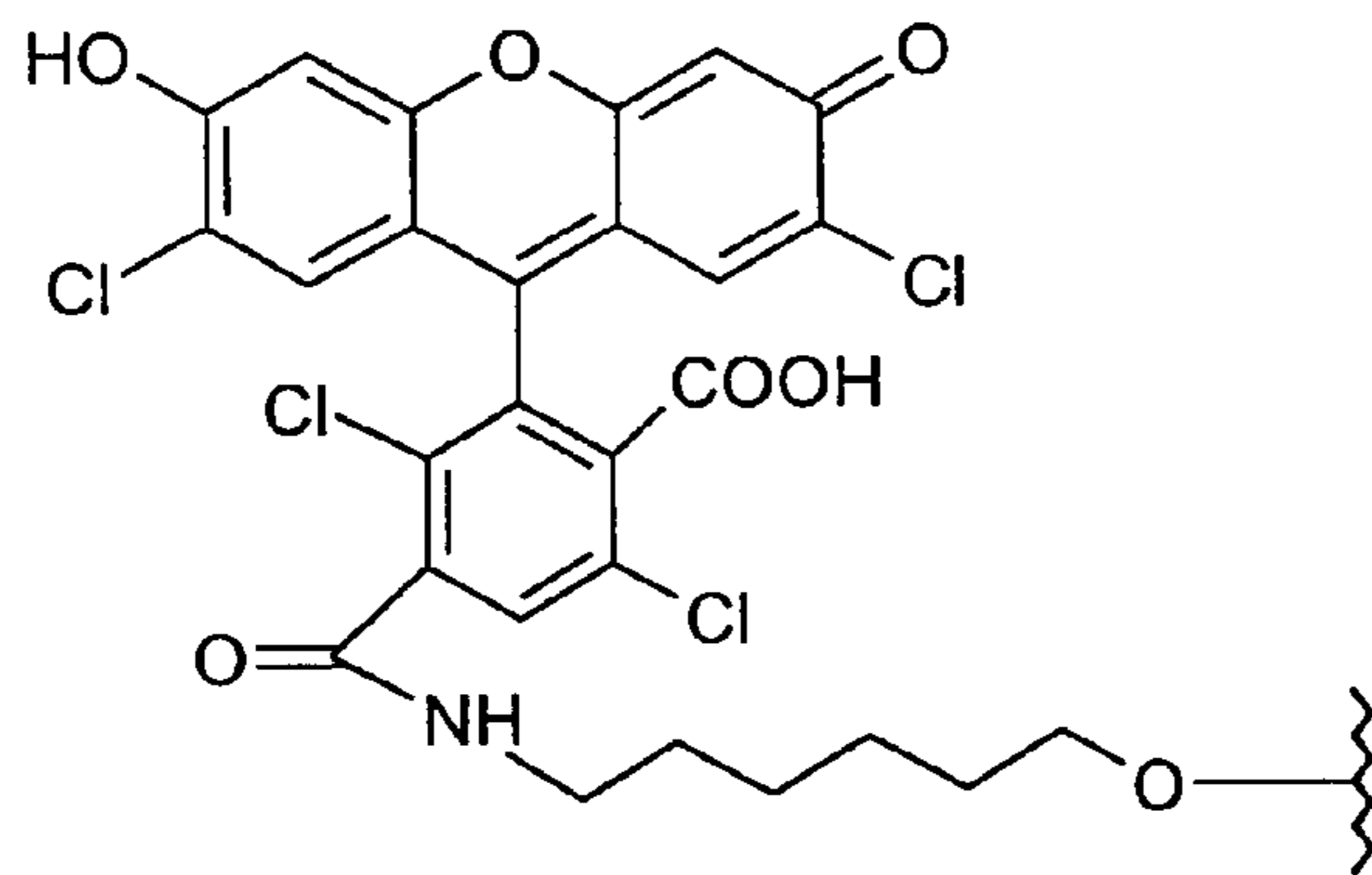
Tetrachlorofluorescein
