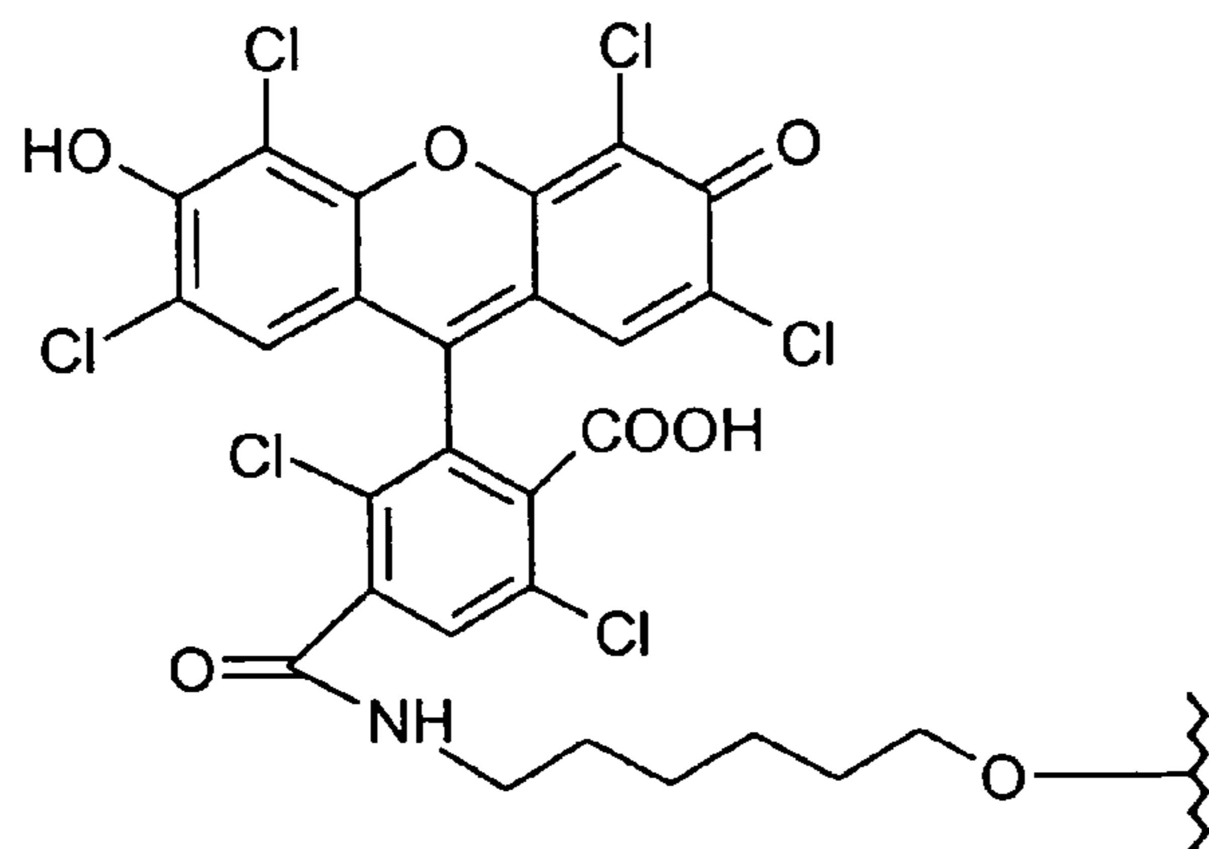
Hexachlorofluorescein
