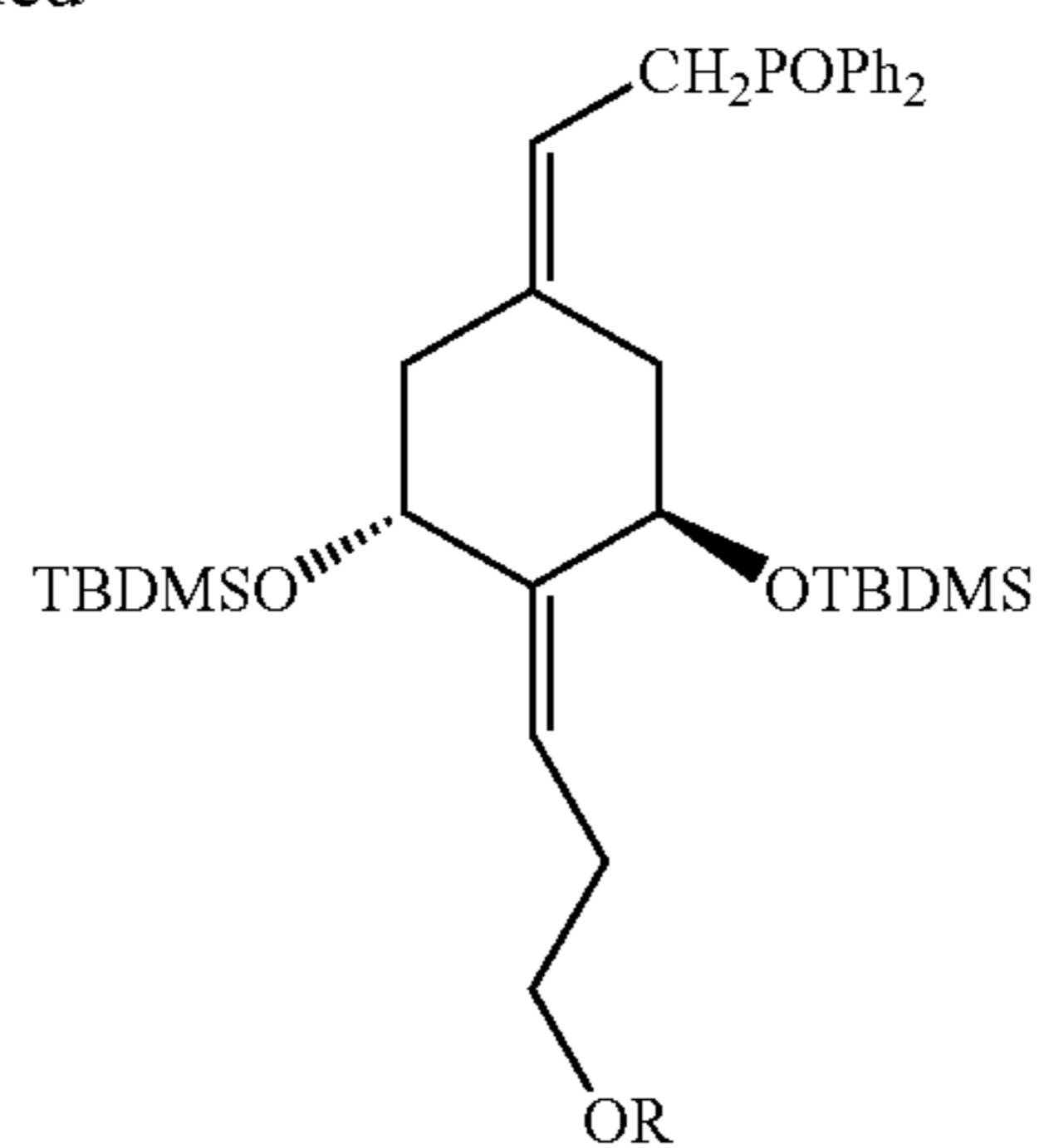
17b: R = MOM, Z-isomer 18b: R = TBDMS, Z-isomer
