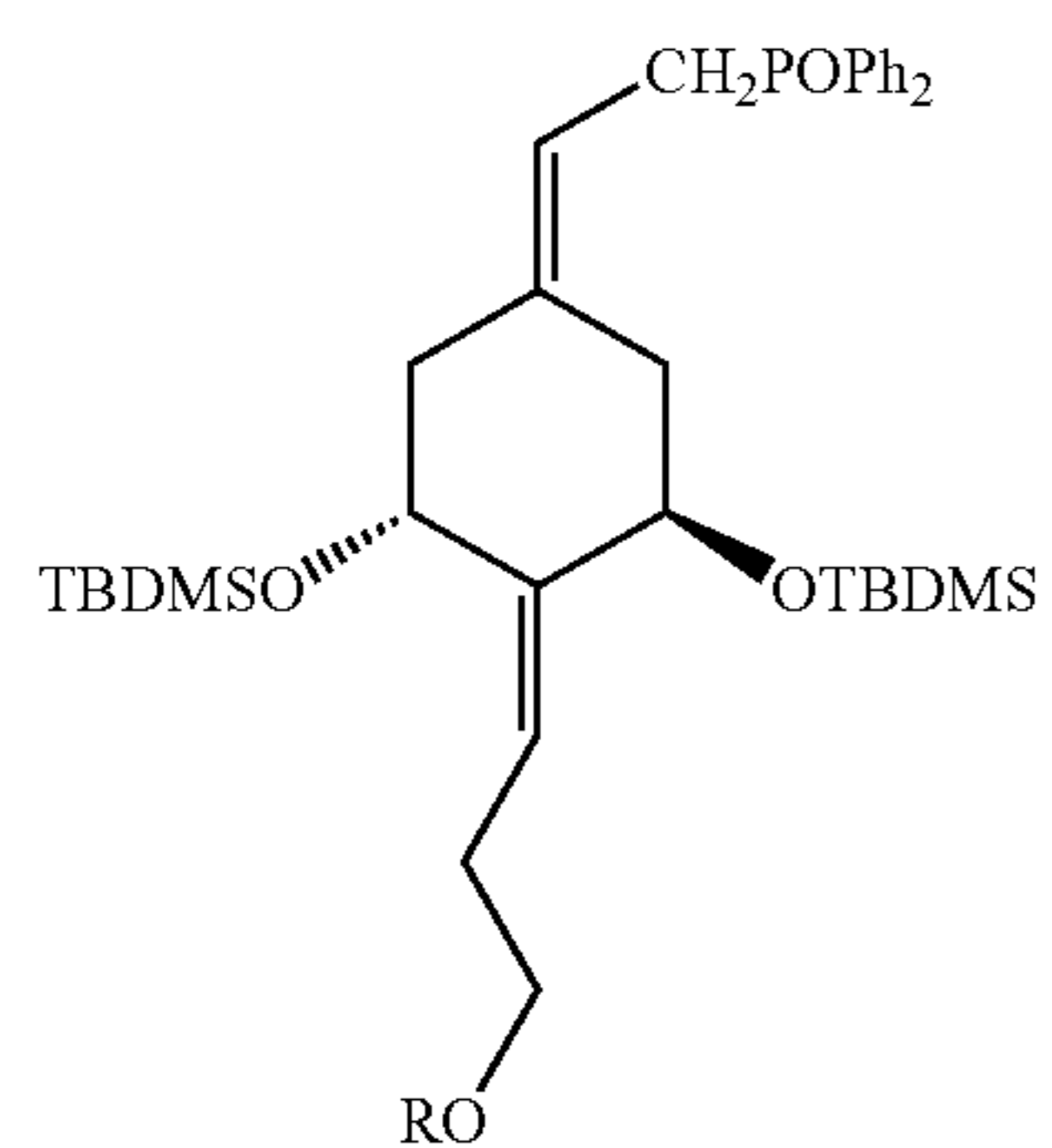
17a: R = MOM, E-isomer 18a: R = TBDMS, E-isomer
