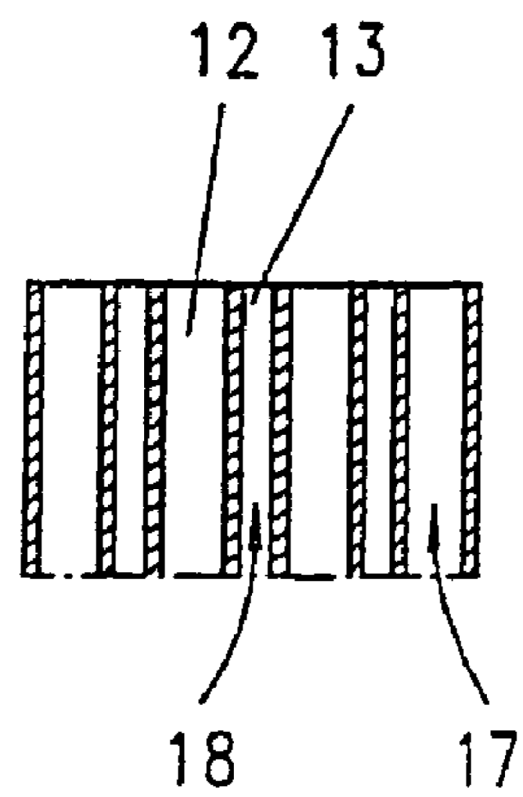
Fig. 4 Detail B
