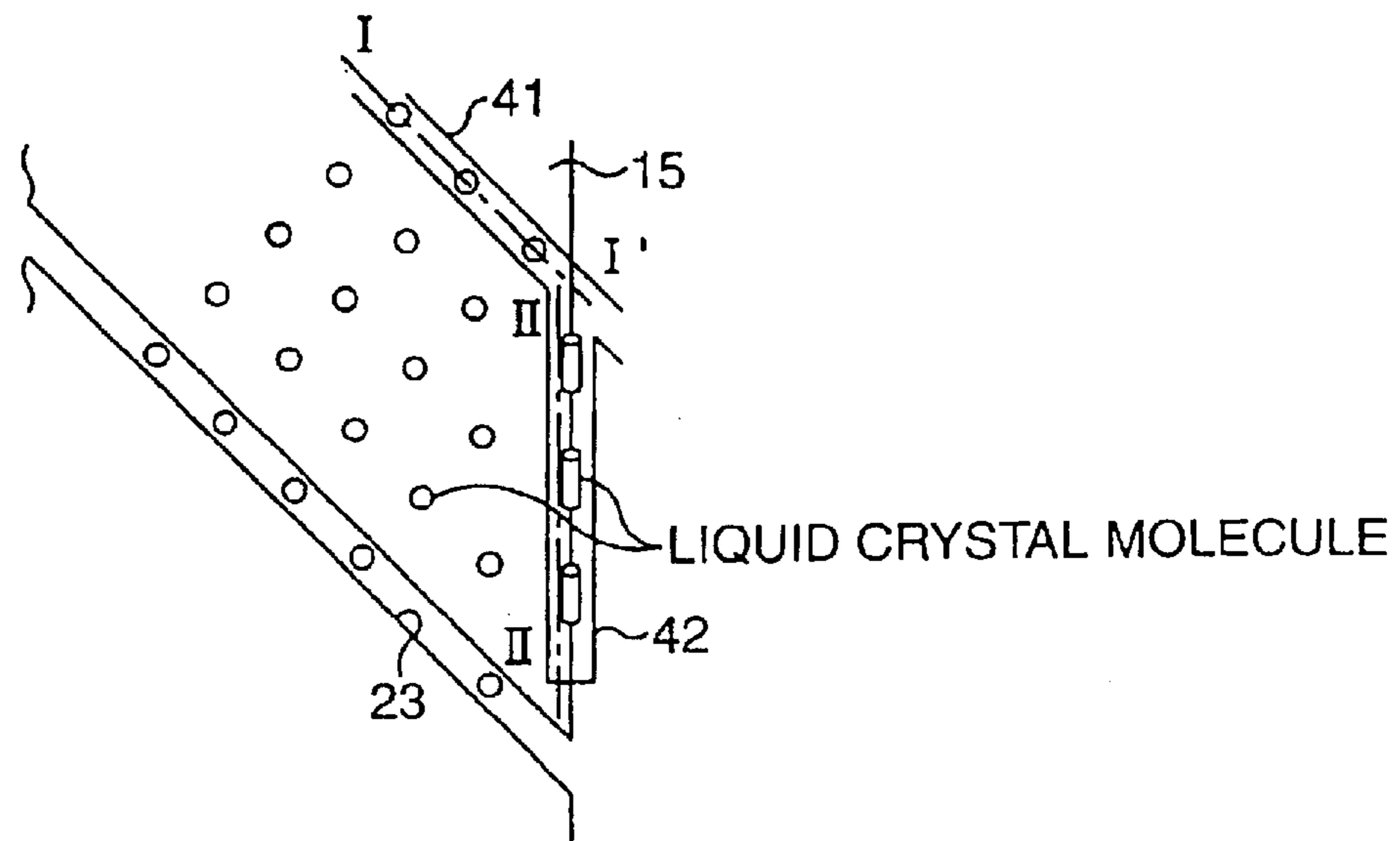
PLANE VIEW
