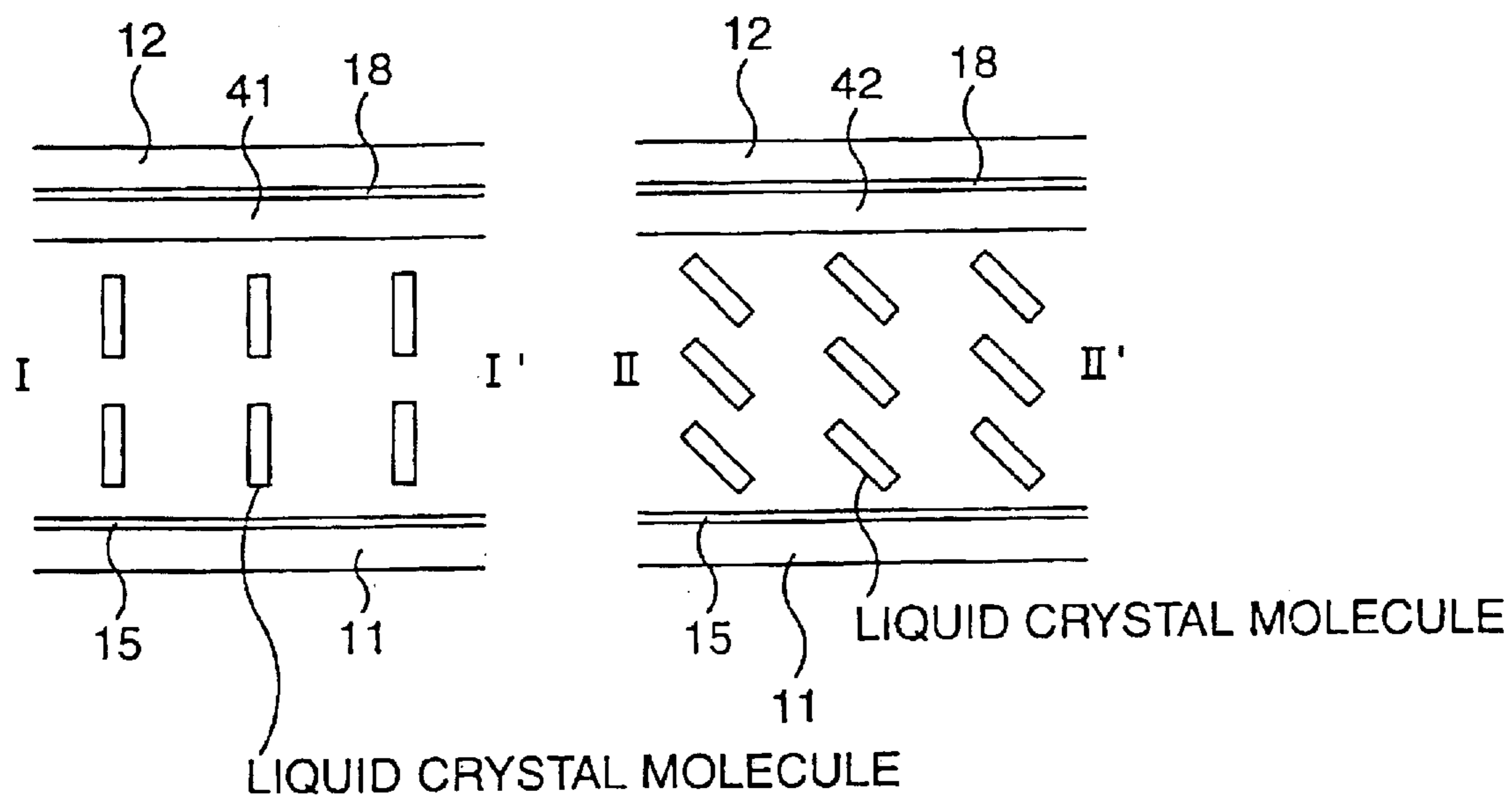
SECTIONAL VIEW
