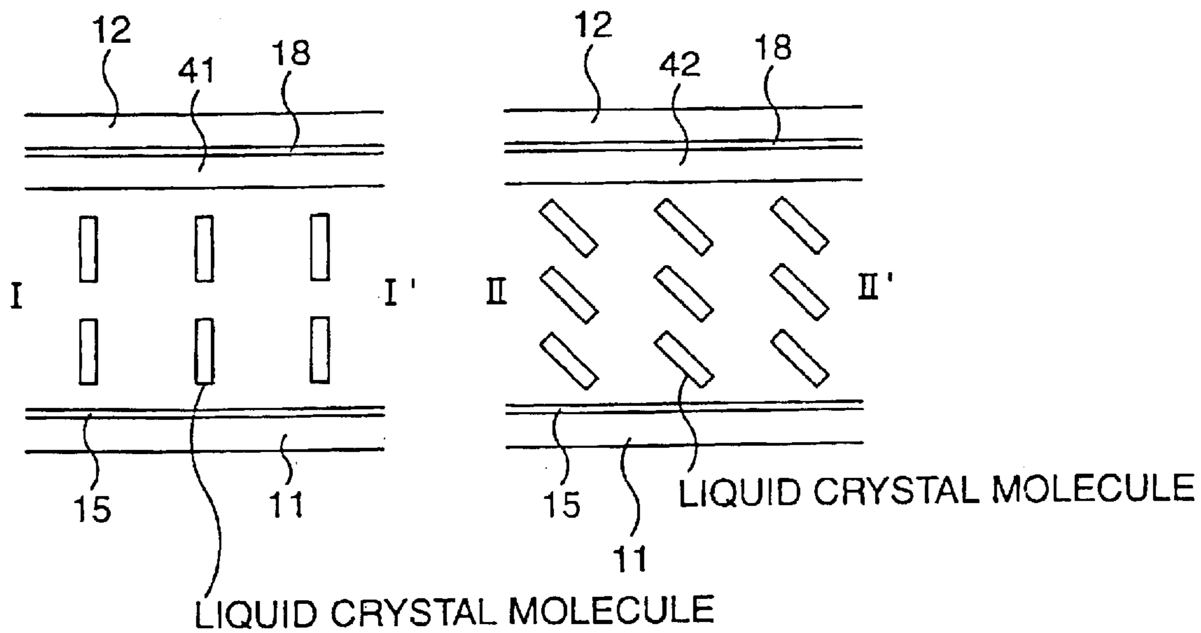
SECTIONAL VIEW
