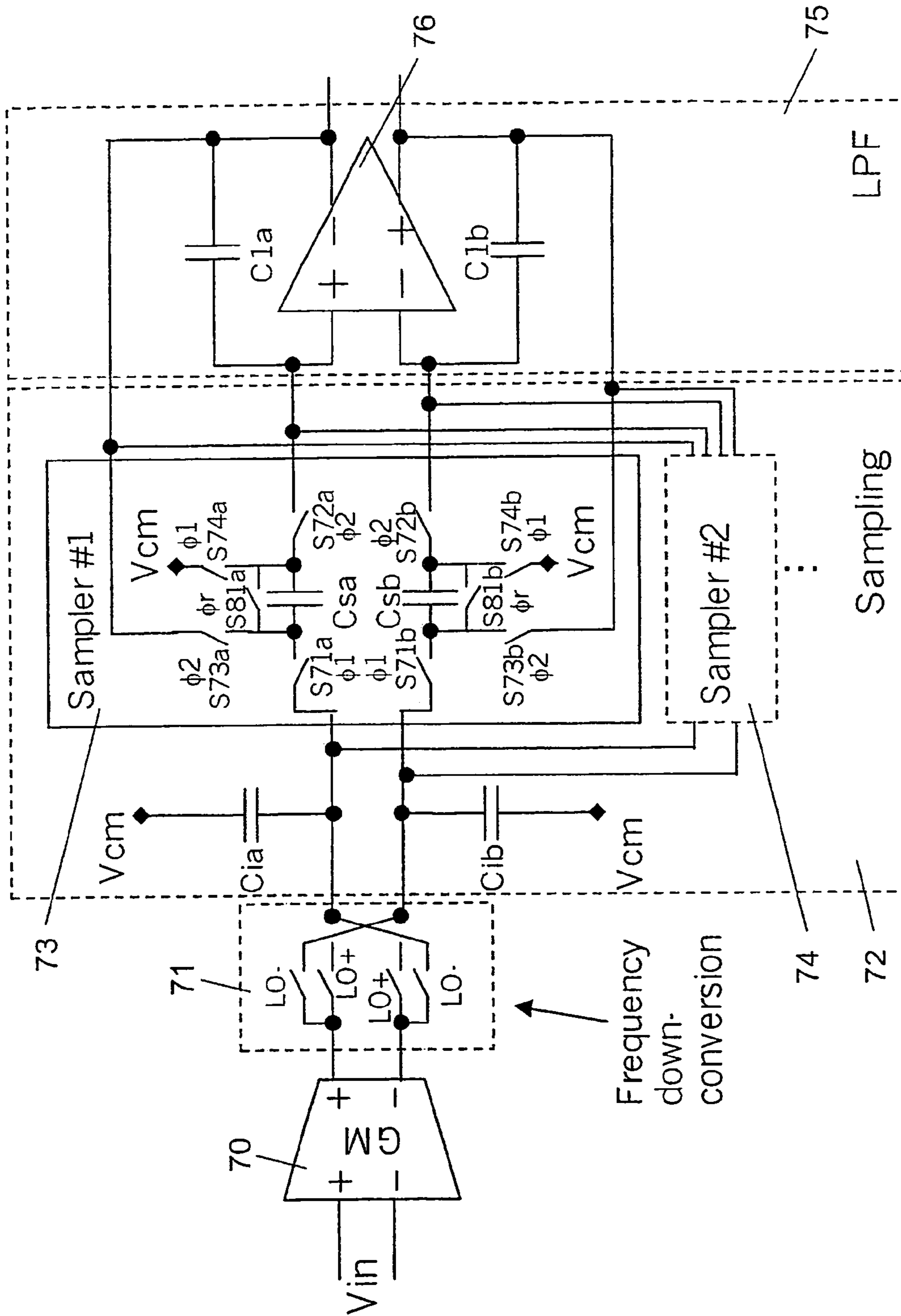
Fig. 8 (prior art)
