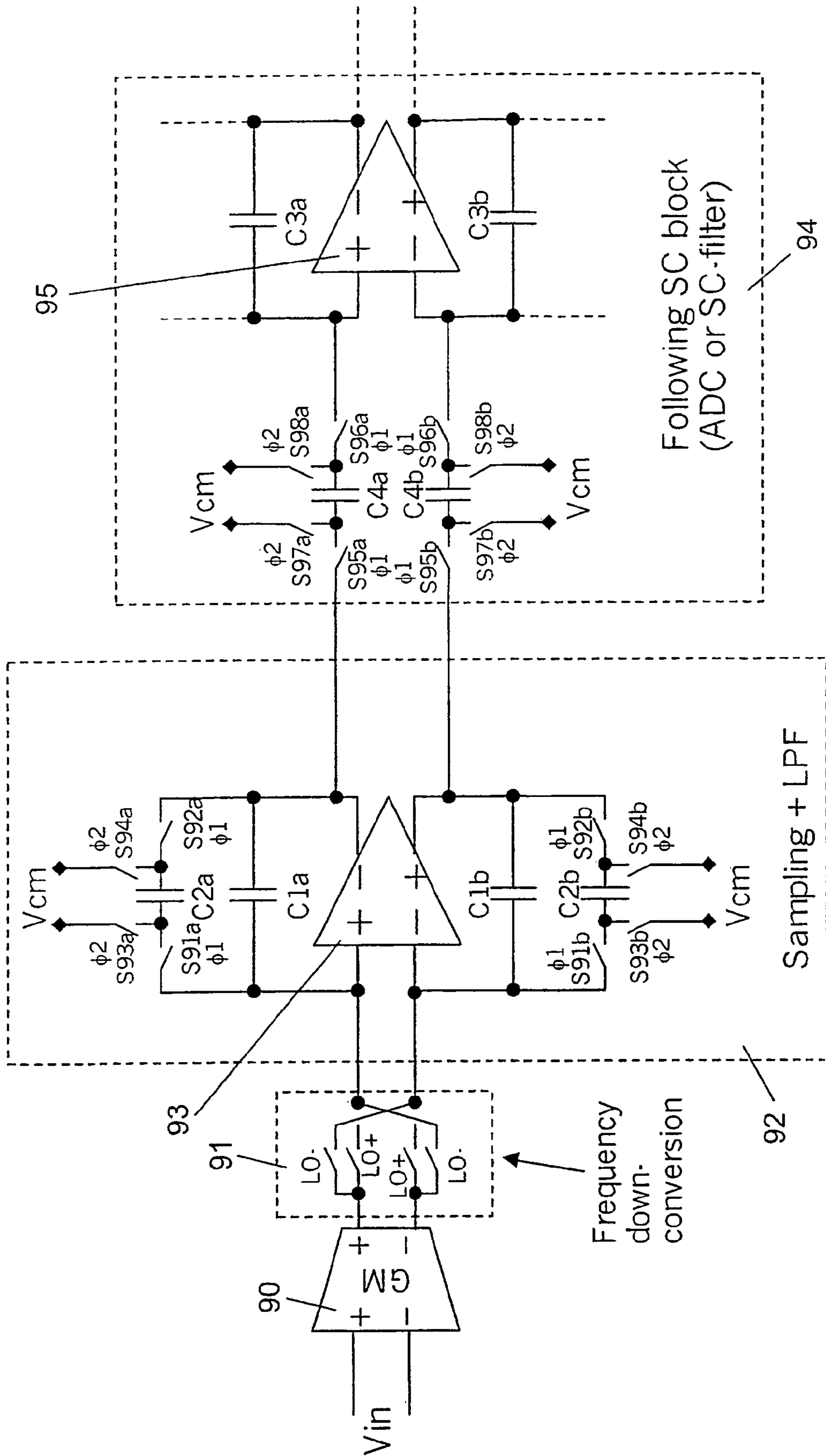
Fig. 9 (prior art)
