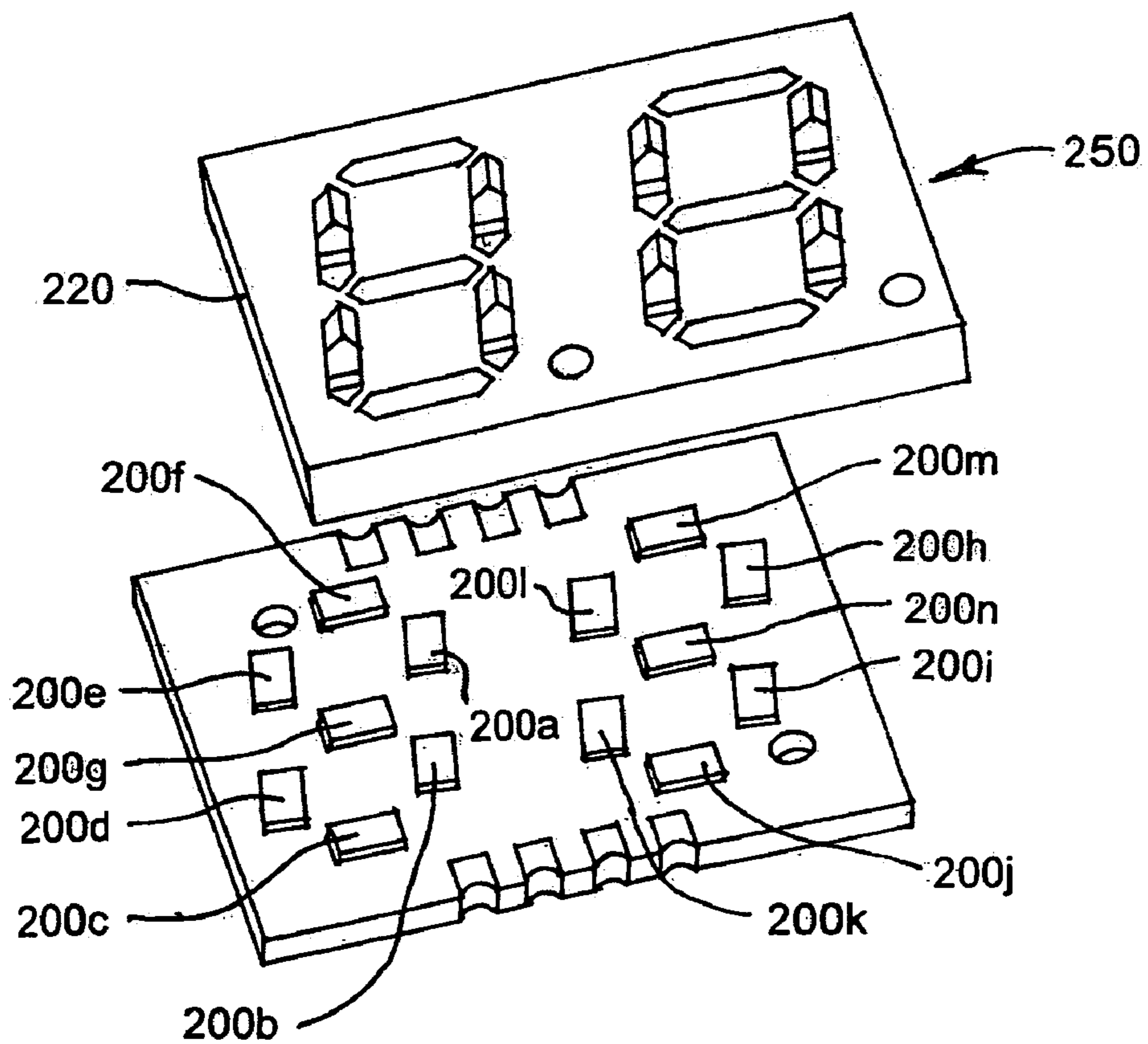
Figure 2 (PRIOR ART)
