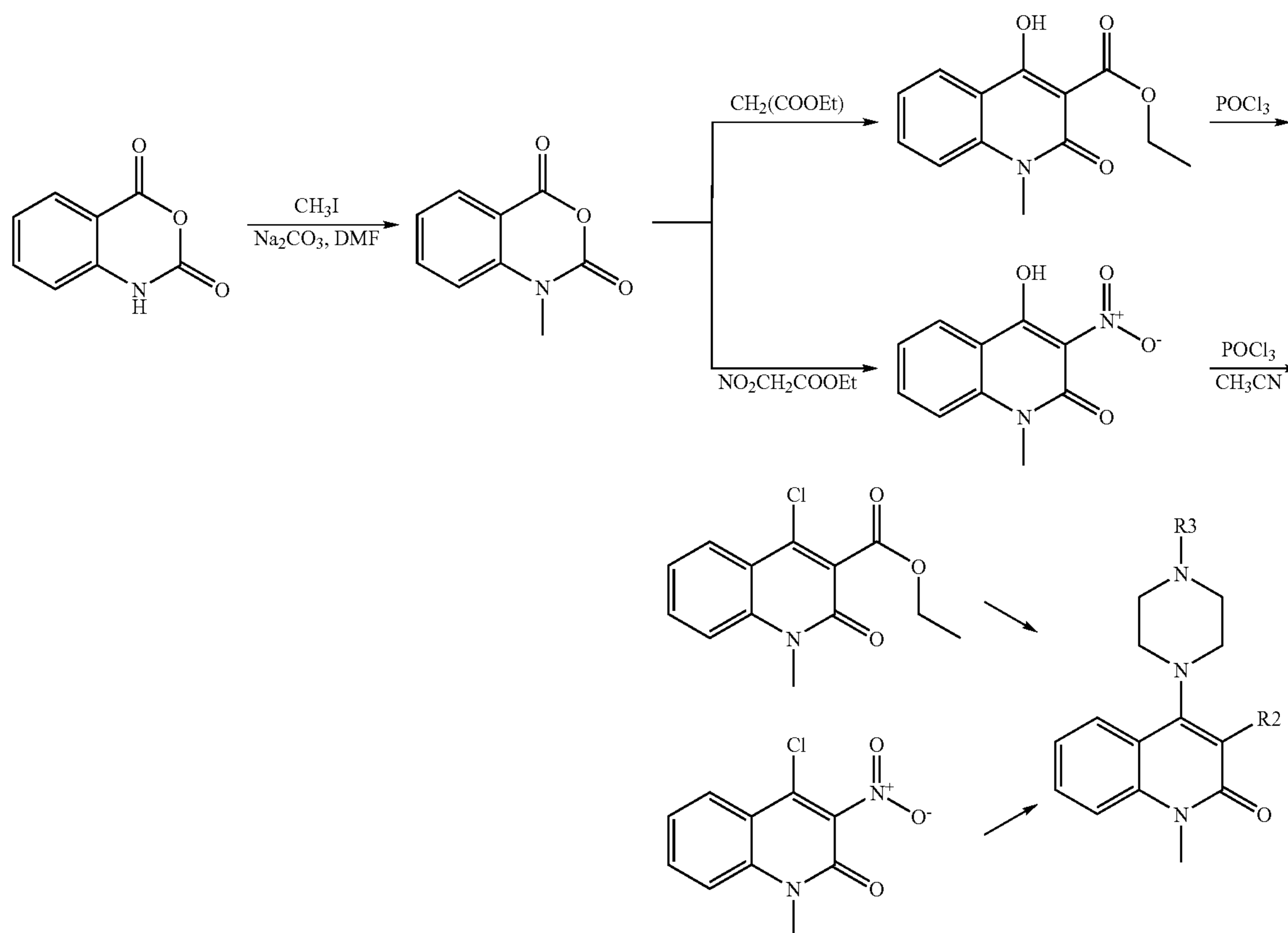
Reaction Scheme 9
