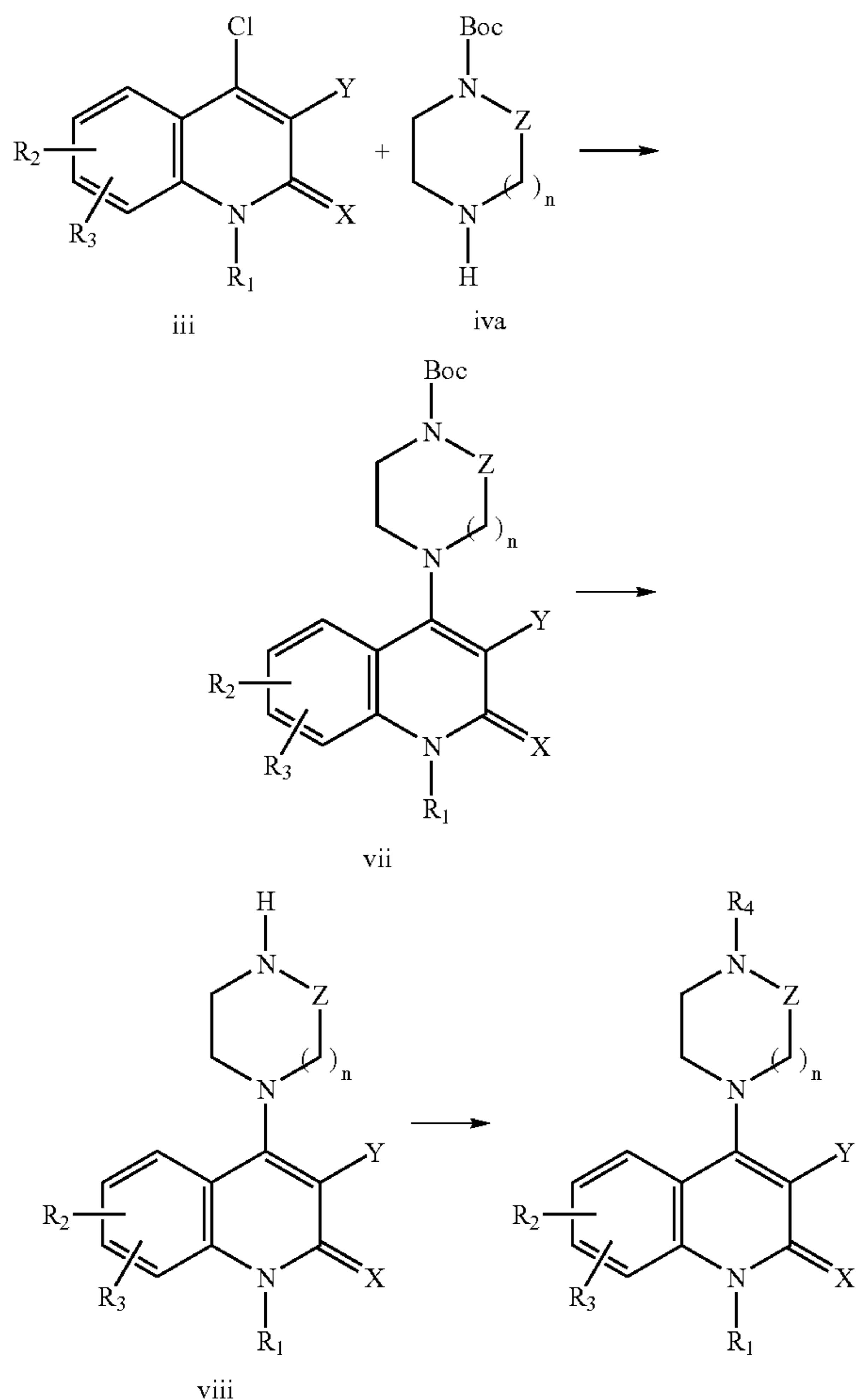
Reaction Scheme 4
