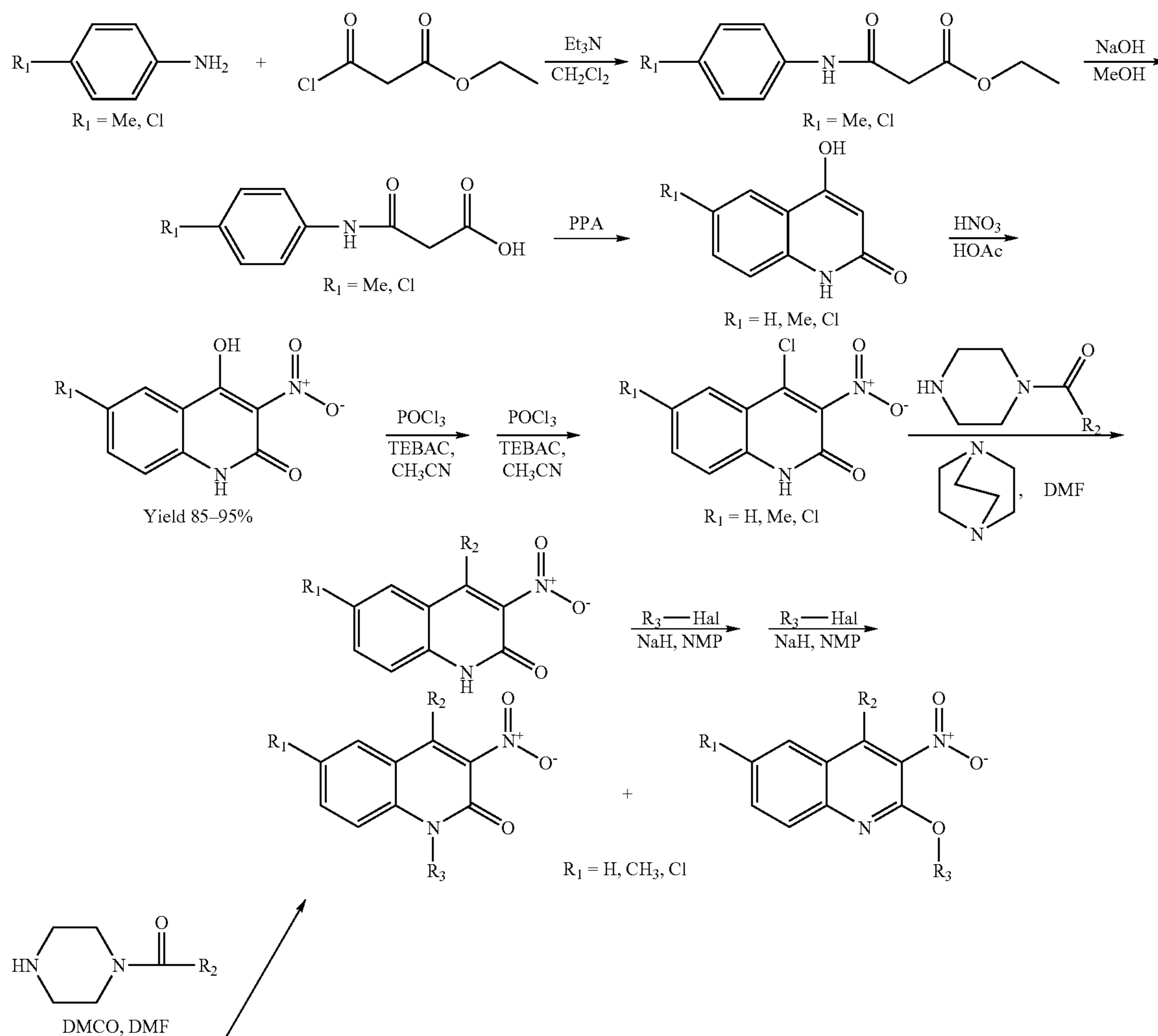
Reaction Scheme 22
