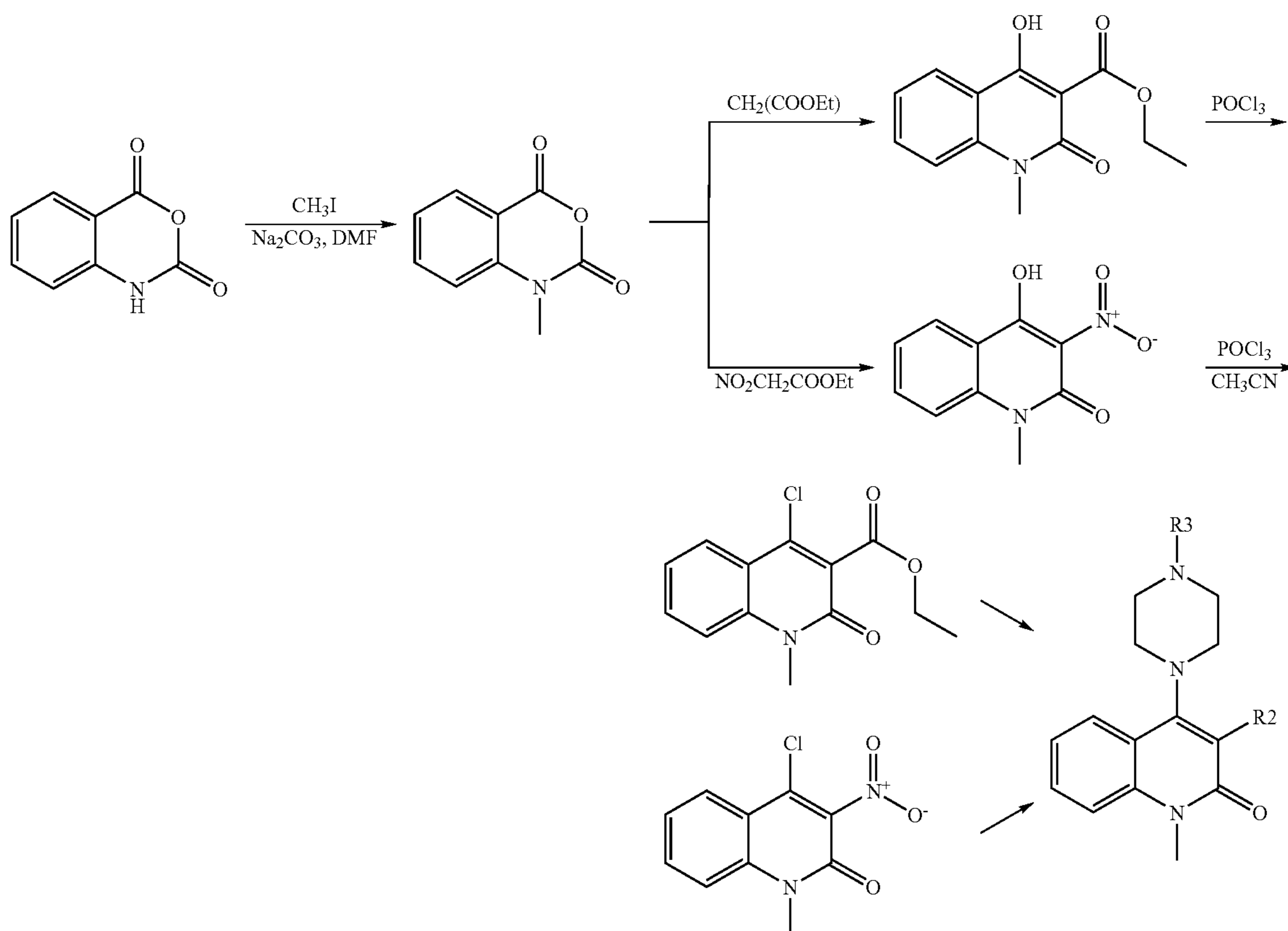
Reaction Scheme 9
