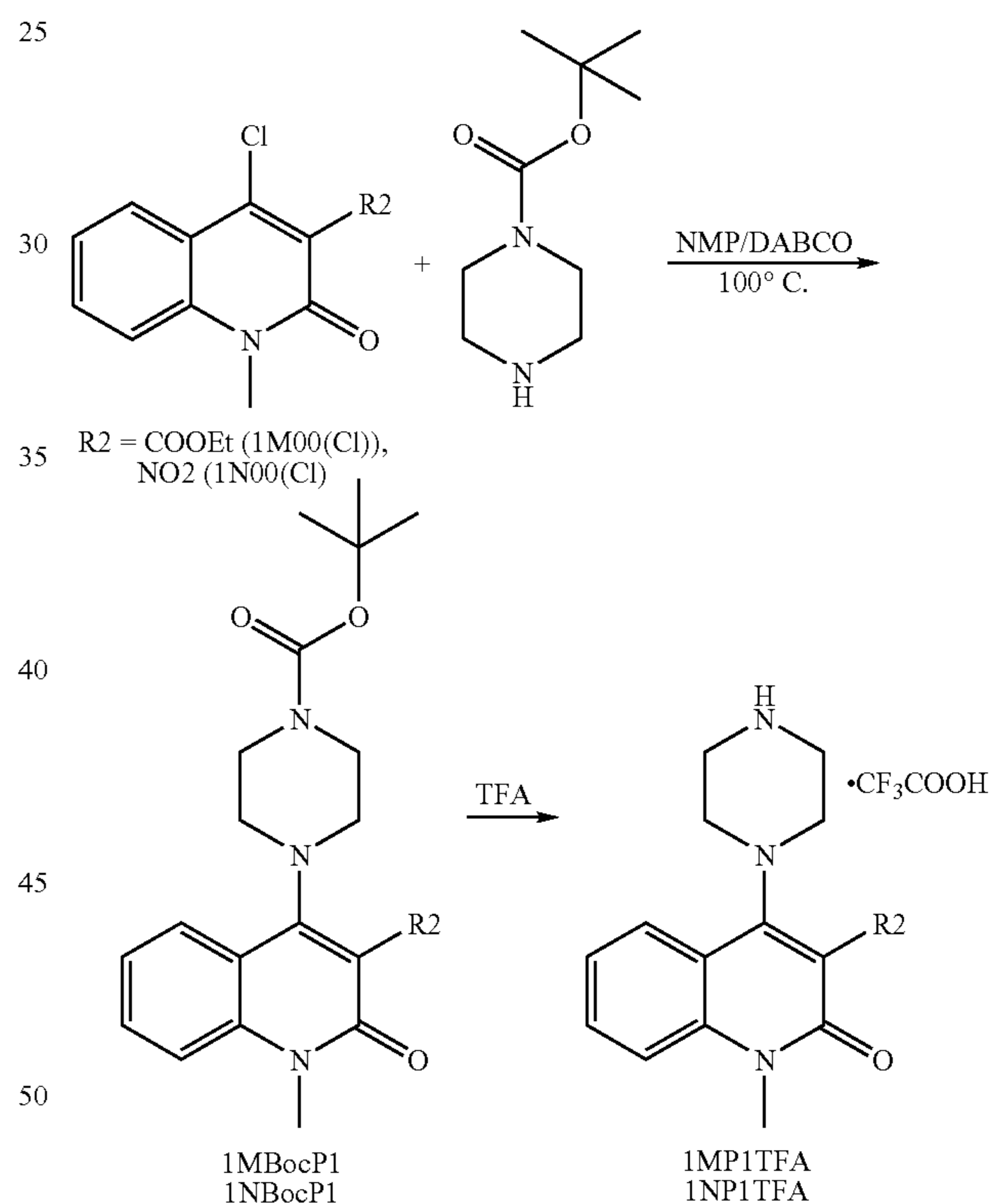
Reaction Scheme 15
