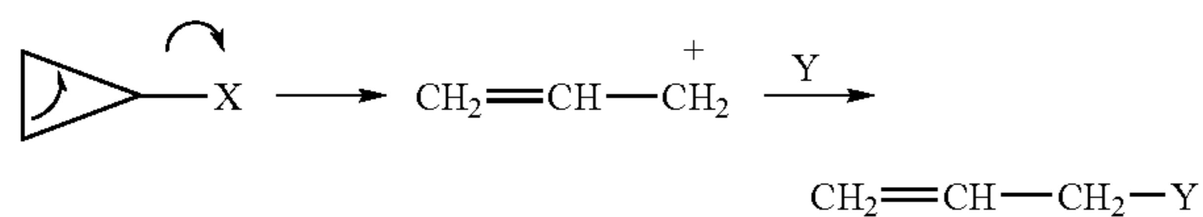
Reaction Scheme 7
