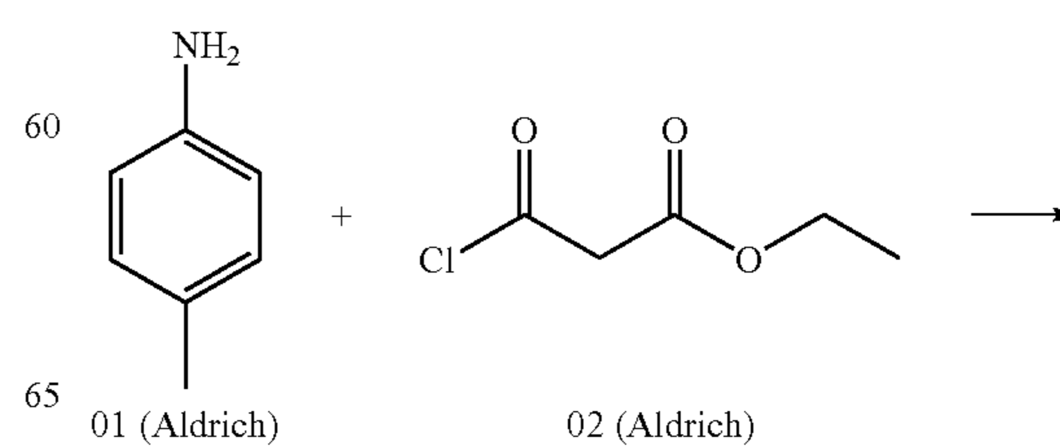
Reaction Scheme 25
