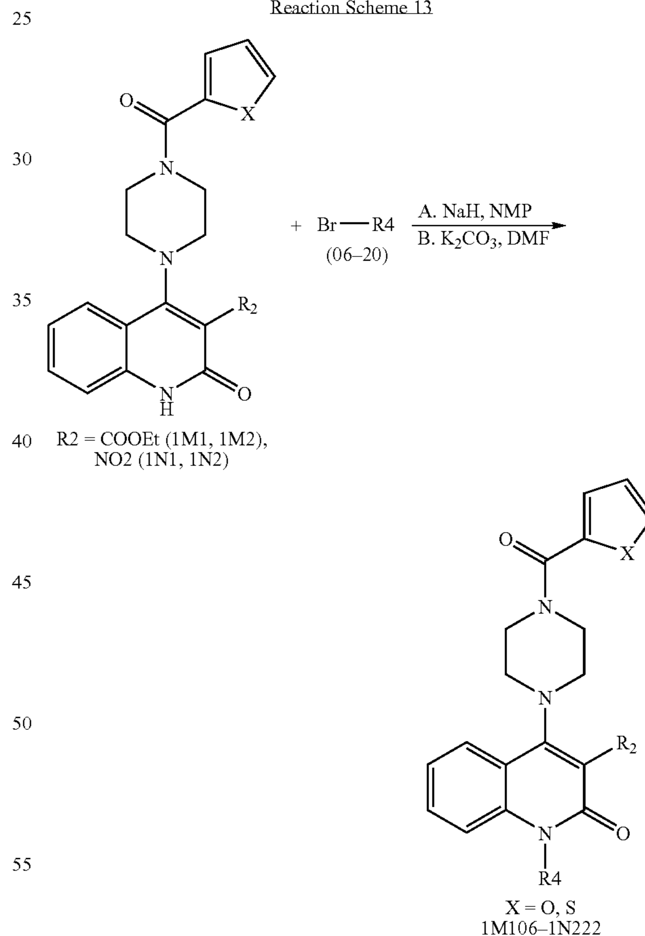
Reaction Scheme 13
