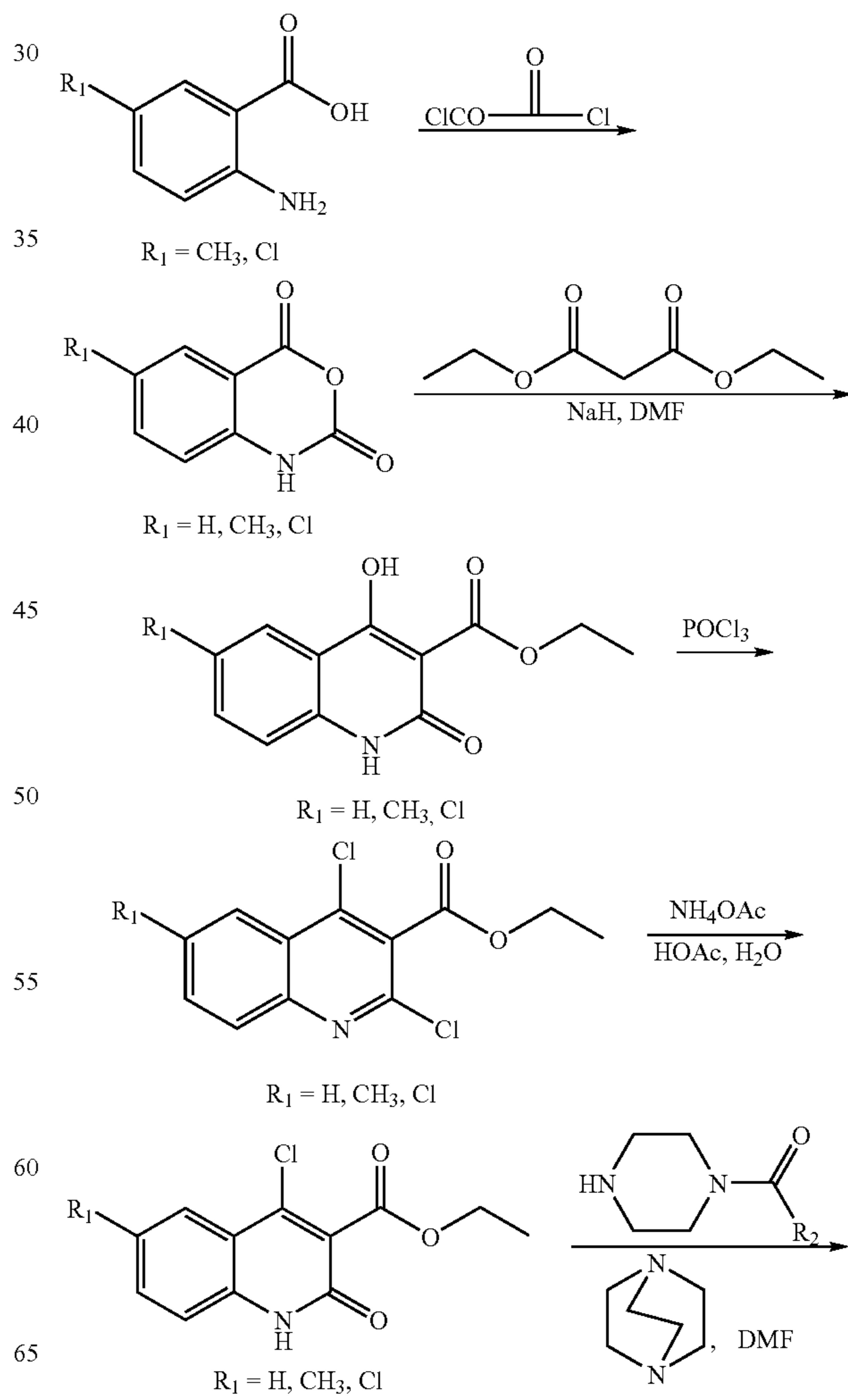
Reaction Scheme 21
