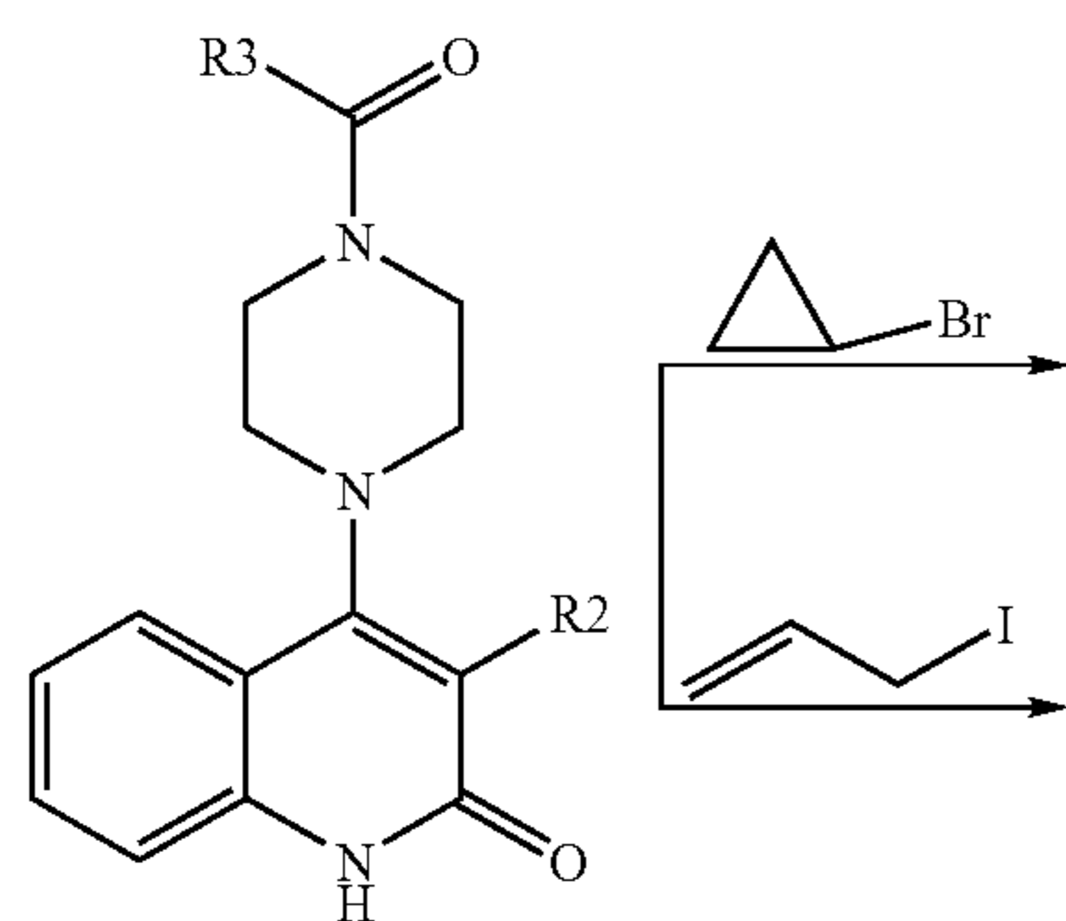
Reaction Scheme 8
