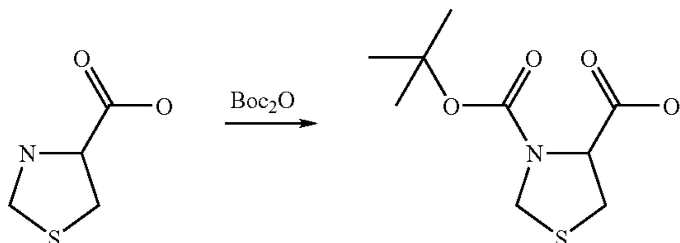
Reaction Scheme 20
