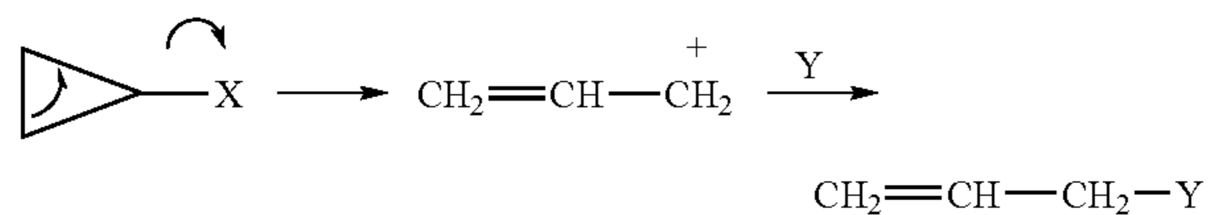
Reaction Scheme 7
