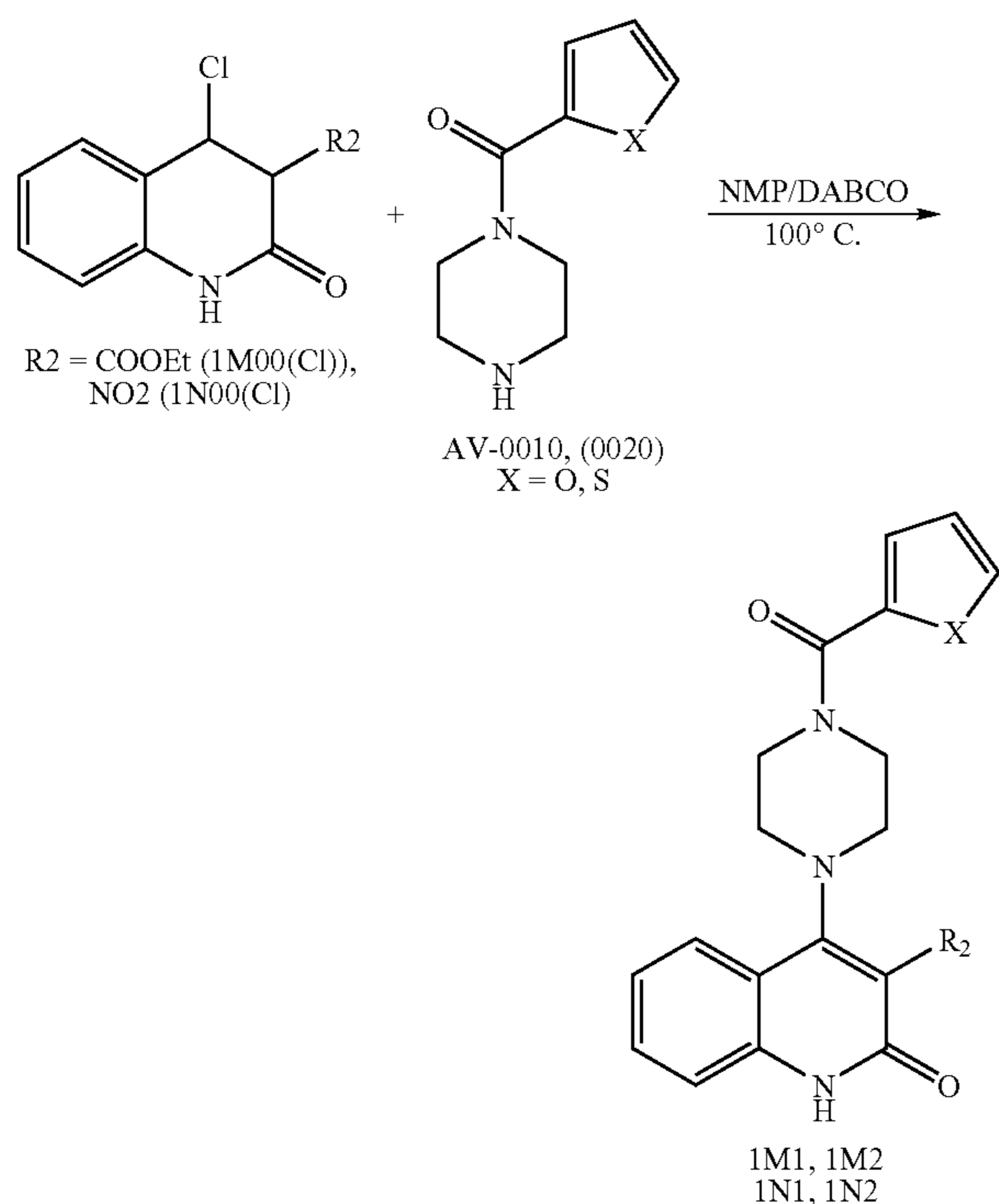
Reaction Scheme 12
