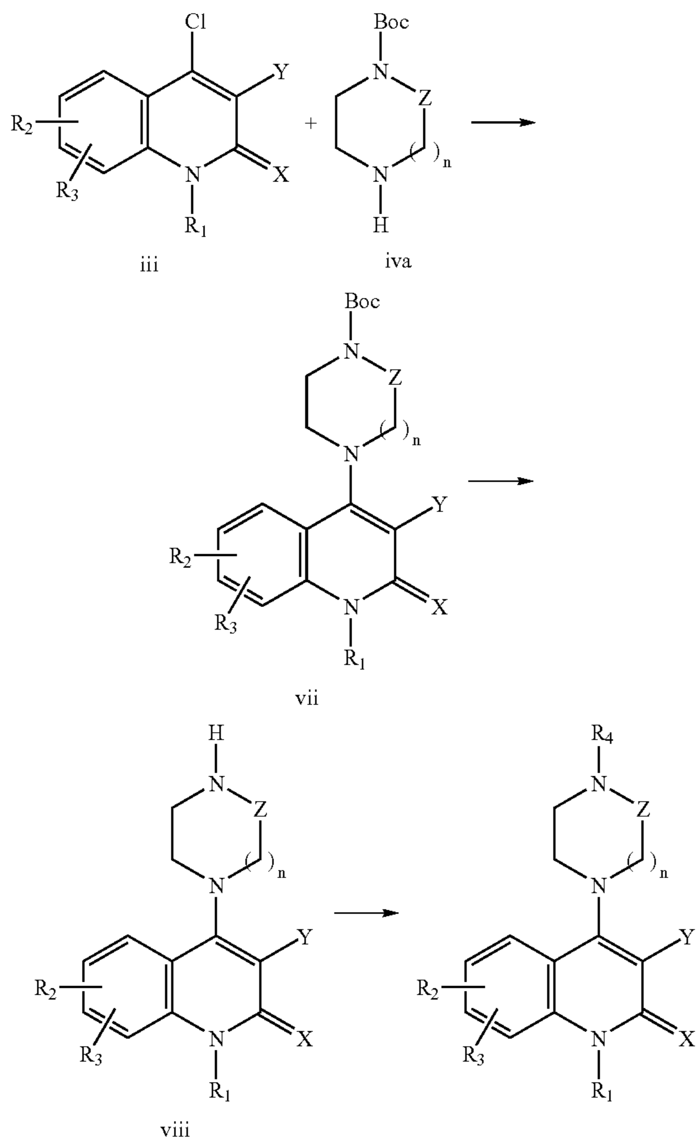
Reaction Scheme 4
