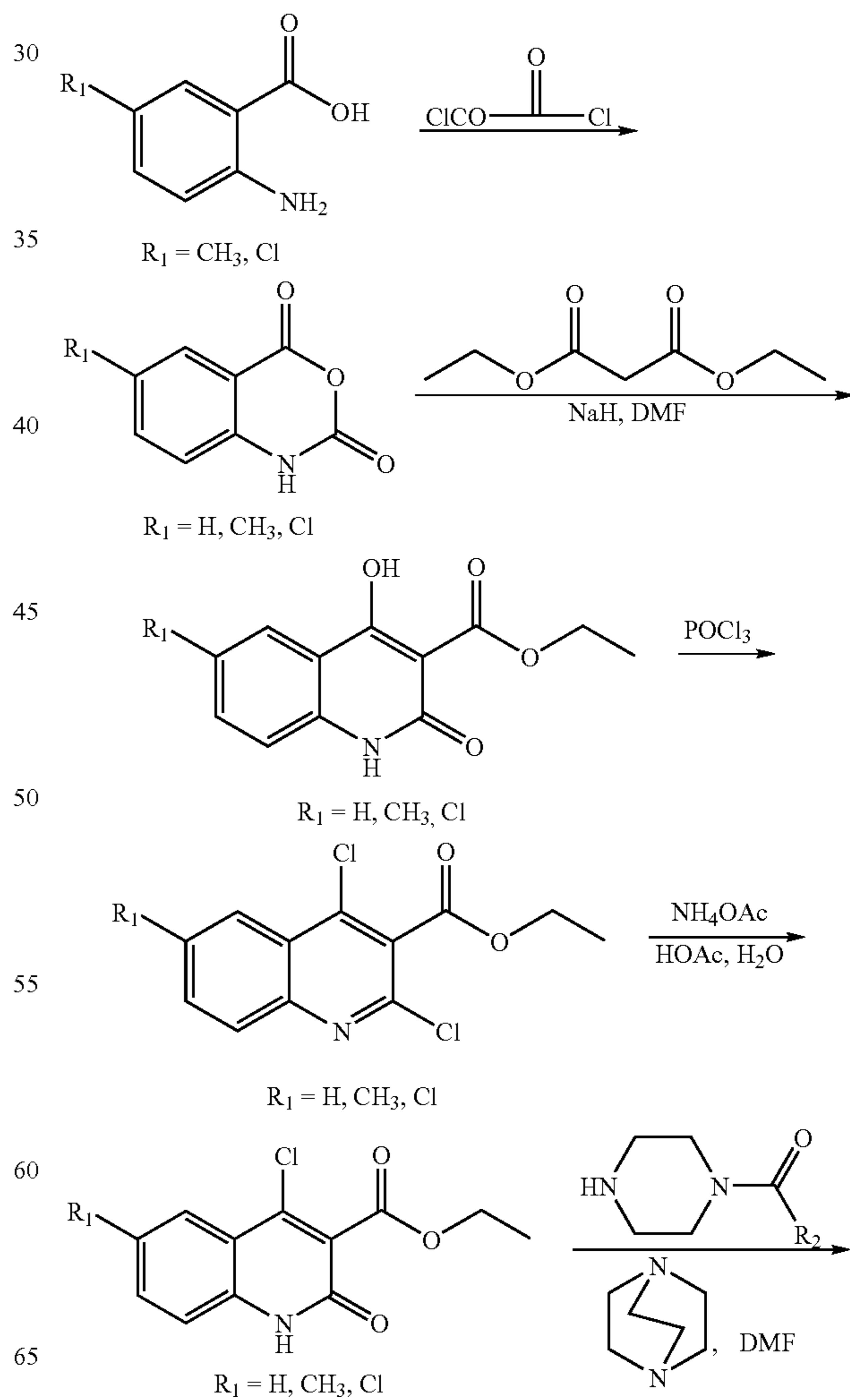
Reaction Scheme 21
