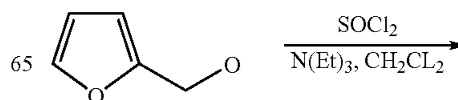
Reaction Scheme 22
