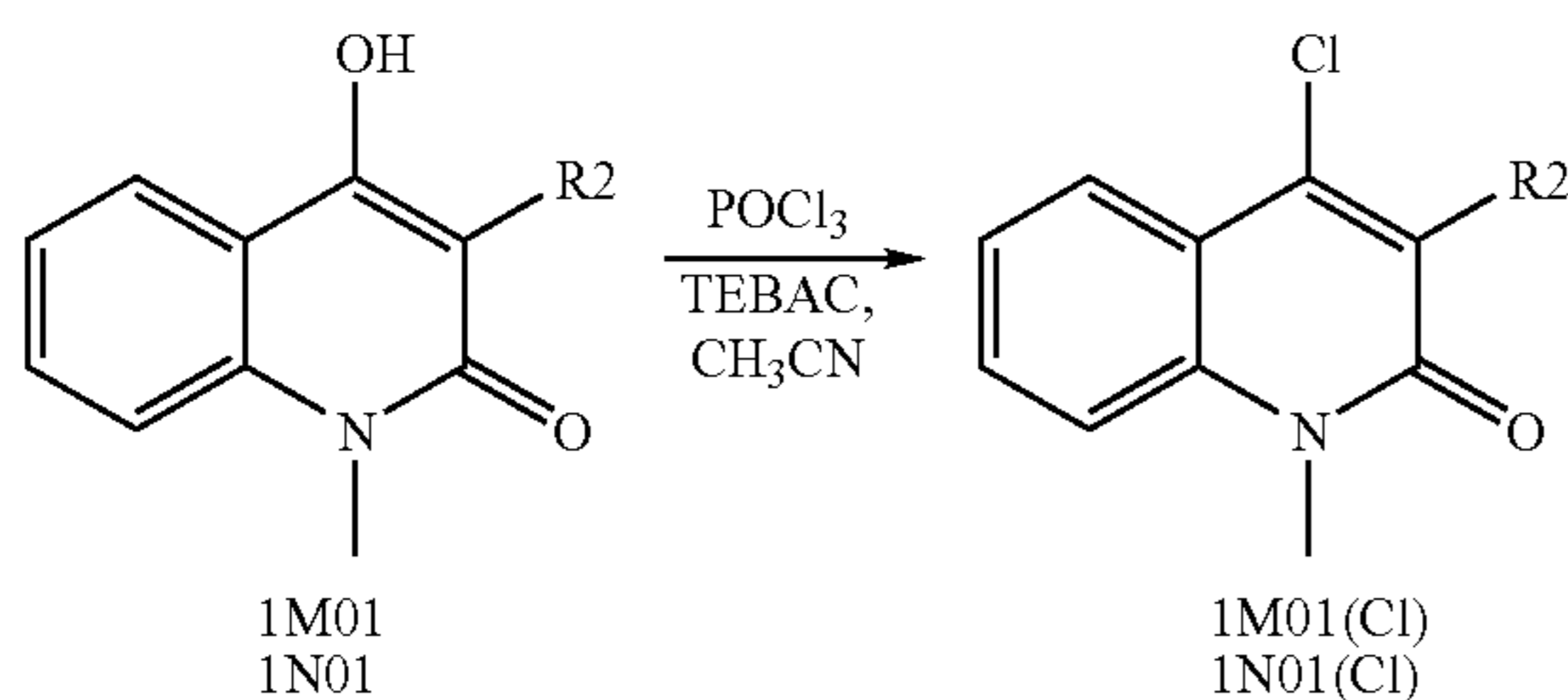
Reaction Scheme 14
