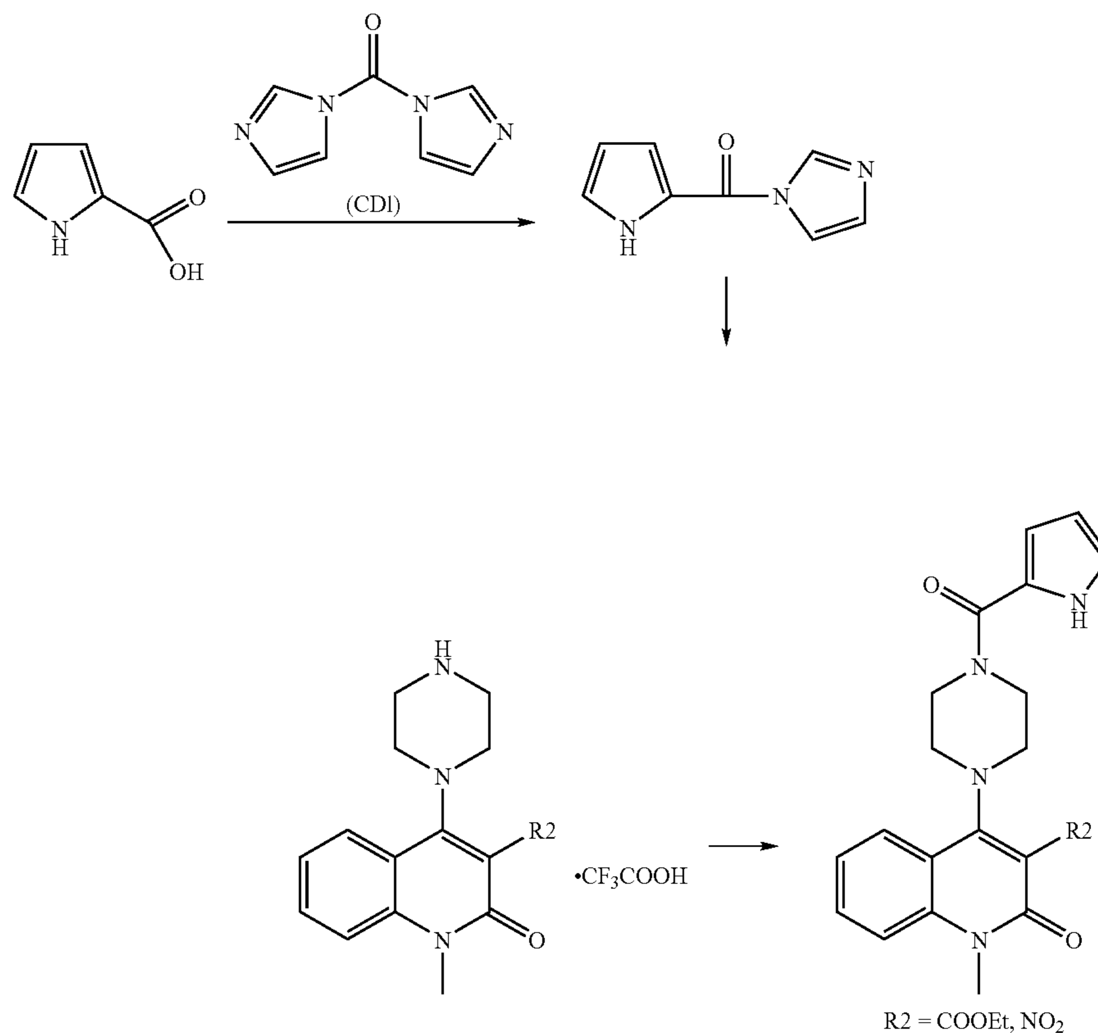
[Reaction Scheme 17]
