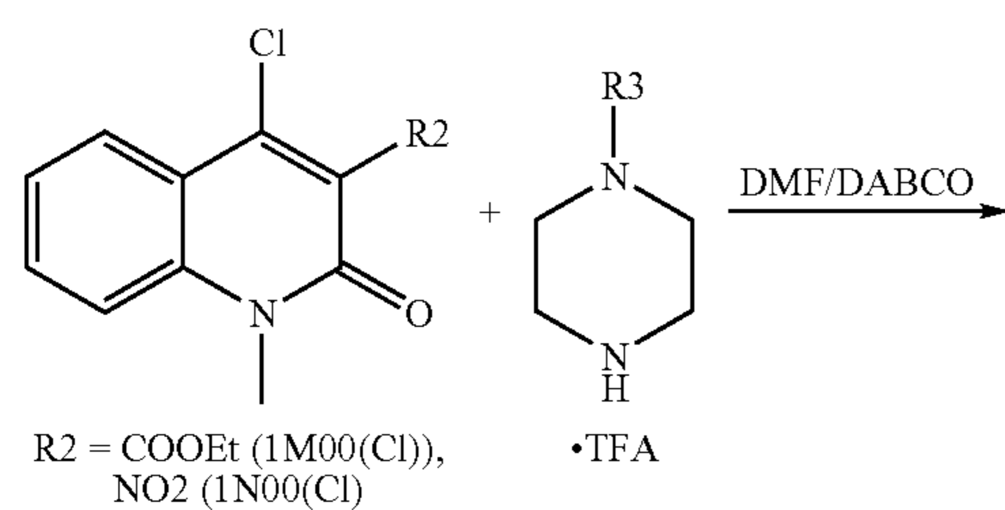
Reaction Scheme 16
