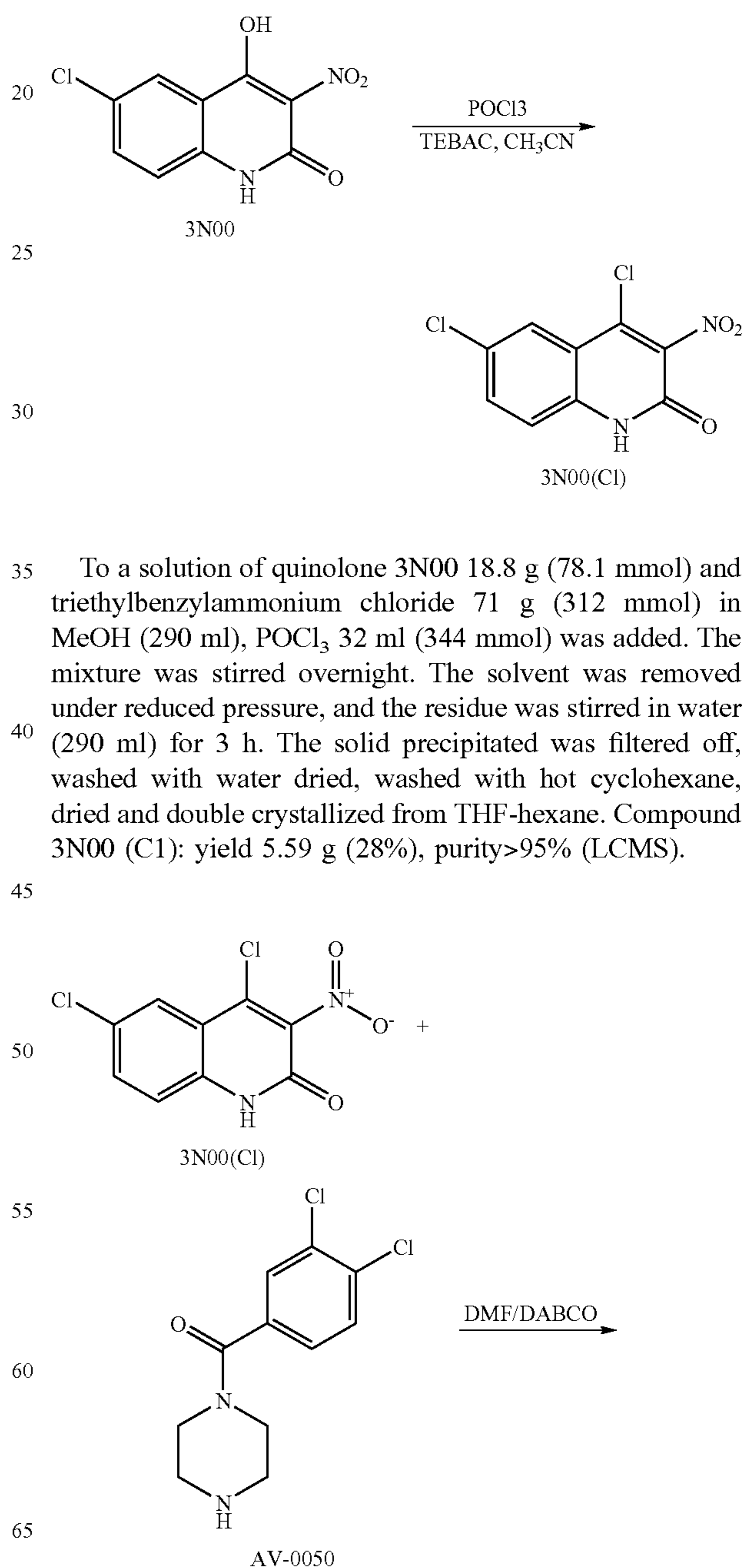
Reaction Scheme 27
