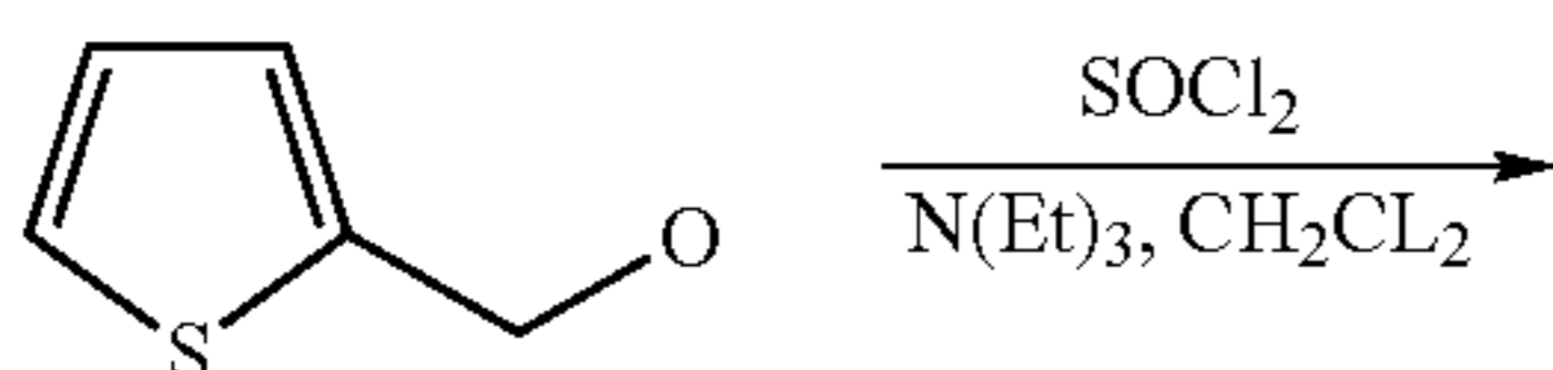
Reaction Scheme 21
