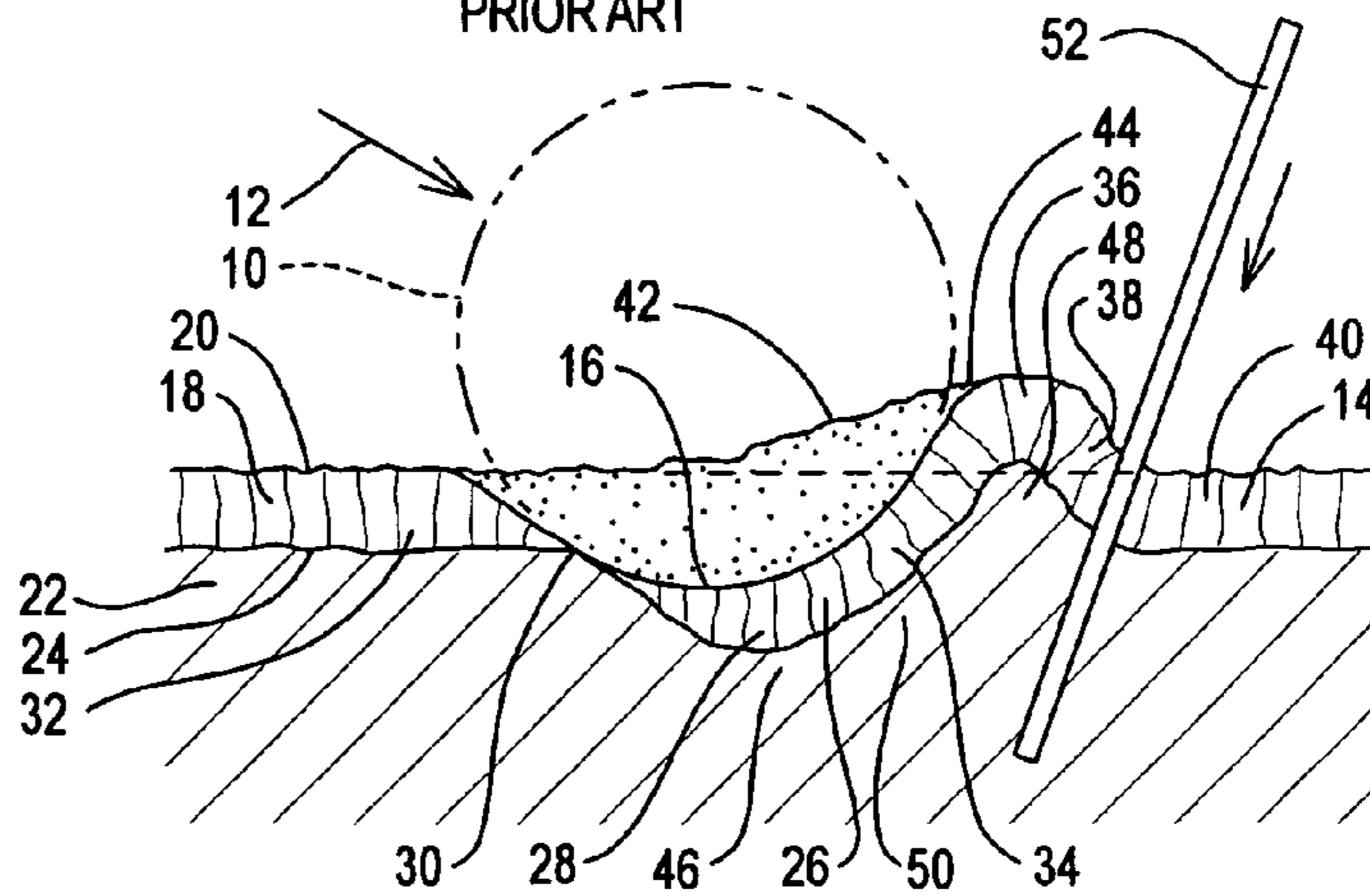
FIG. 2 PRIOR ART
