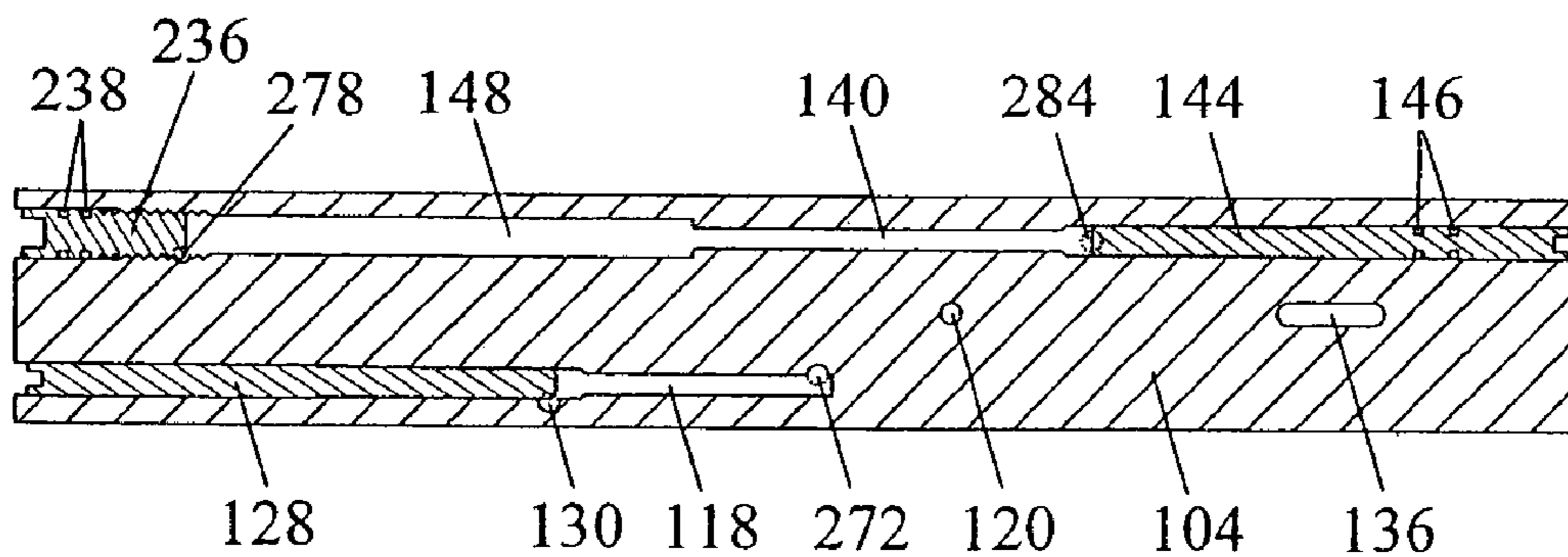
Top Sectional View
