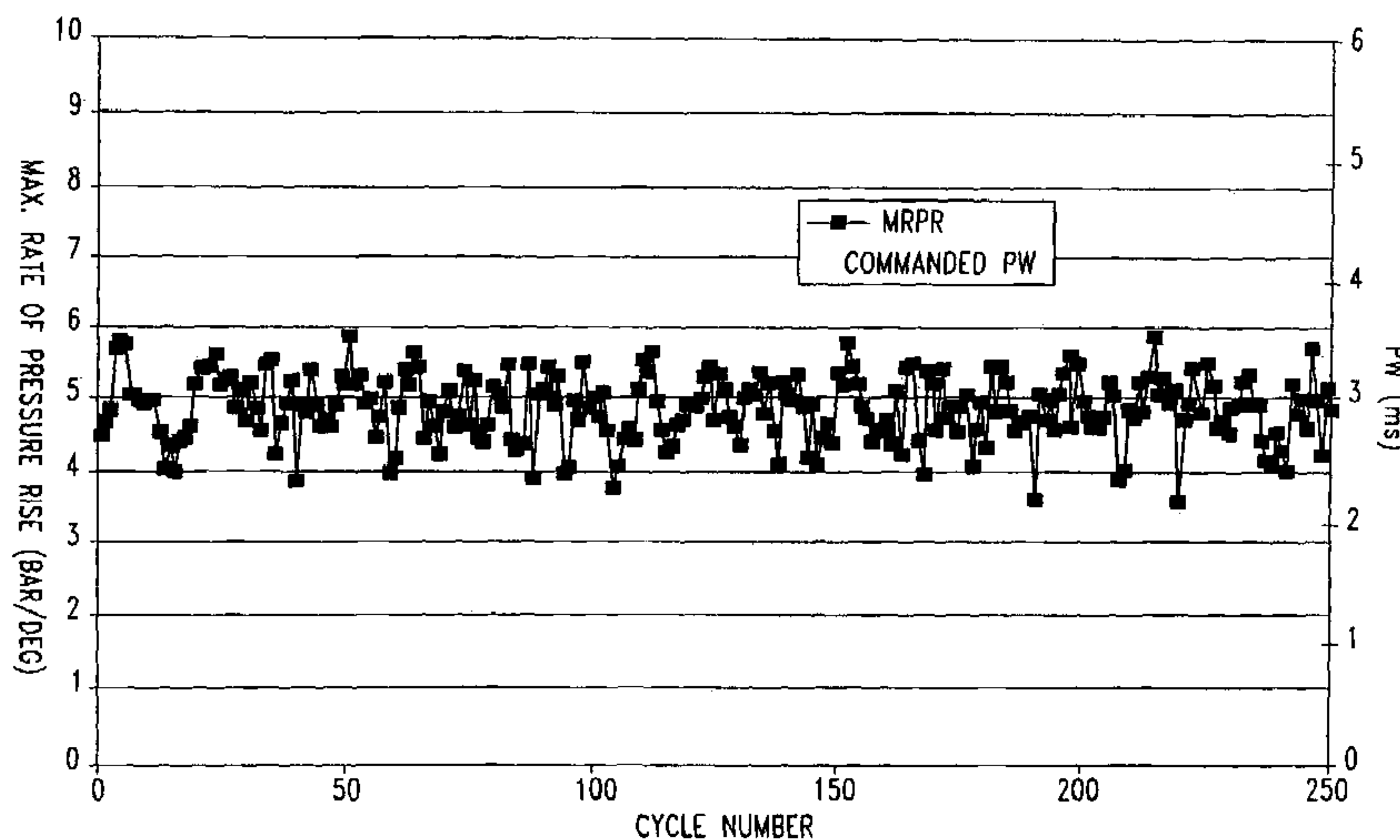
HCCI OPEN LOOP RESPONSE (CYLINDER 2) 1200RPM @ 52Nm
