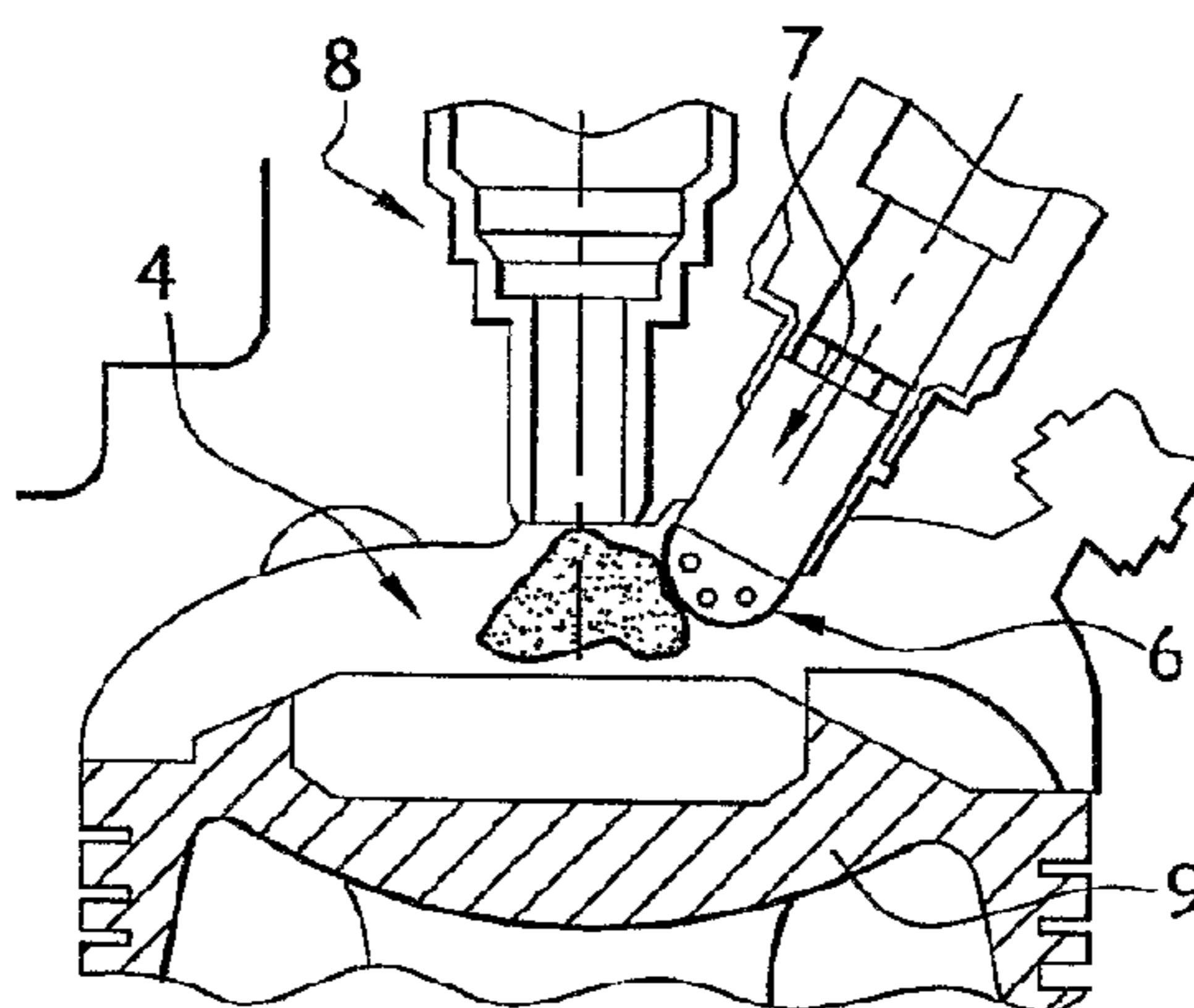
1/ INJECTION / WETTING OF THE PRECOMBUSTION CHAMBER HEAD
