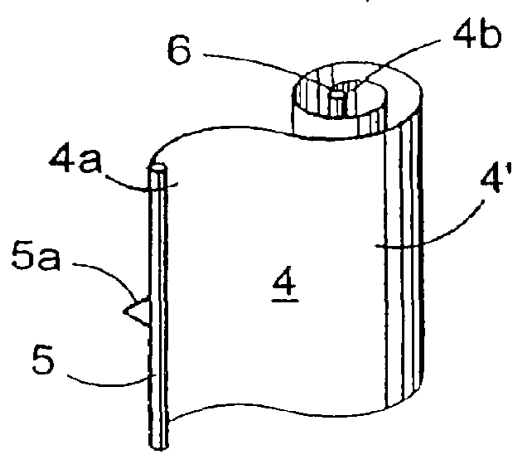
Fig. 4 (Prior Art)
