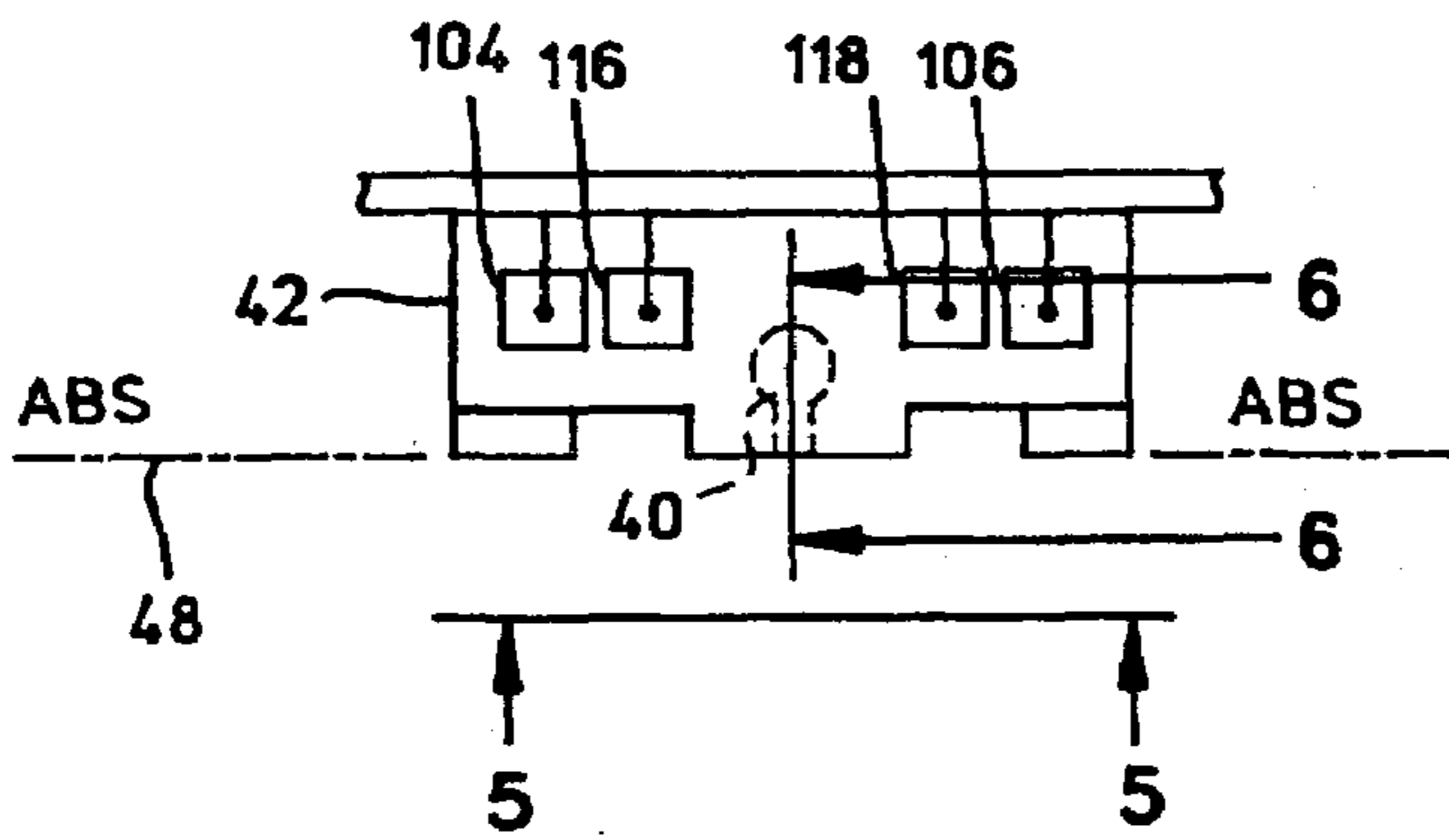
FIG. 2 (PRIOR ART)
