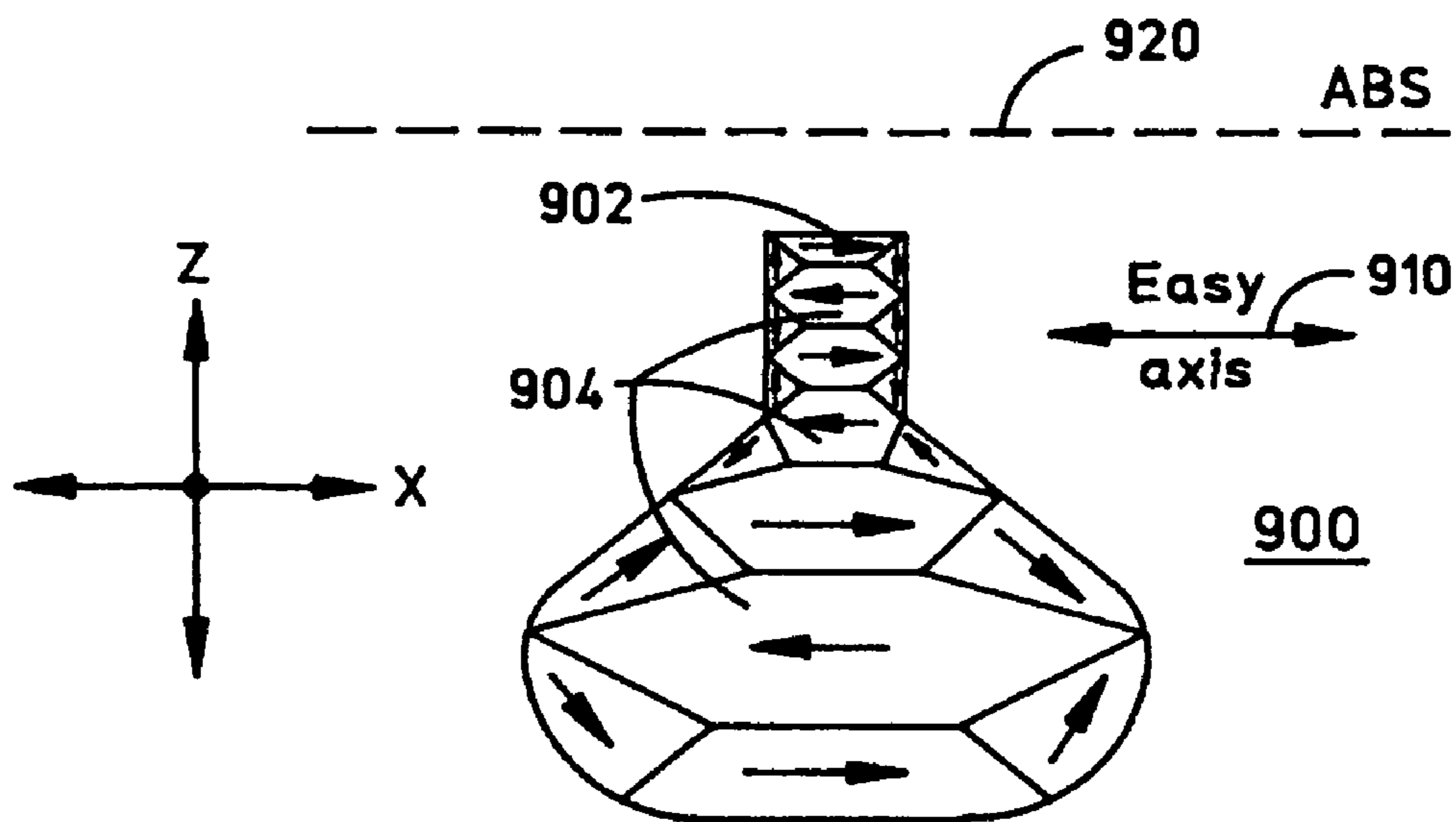
FIG. 9 (PRIOR ART)
