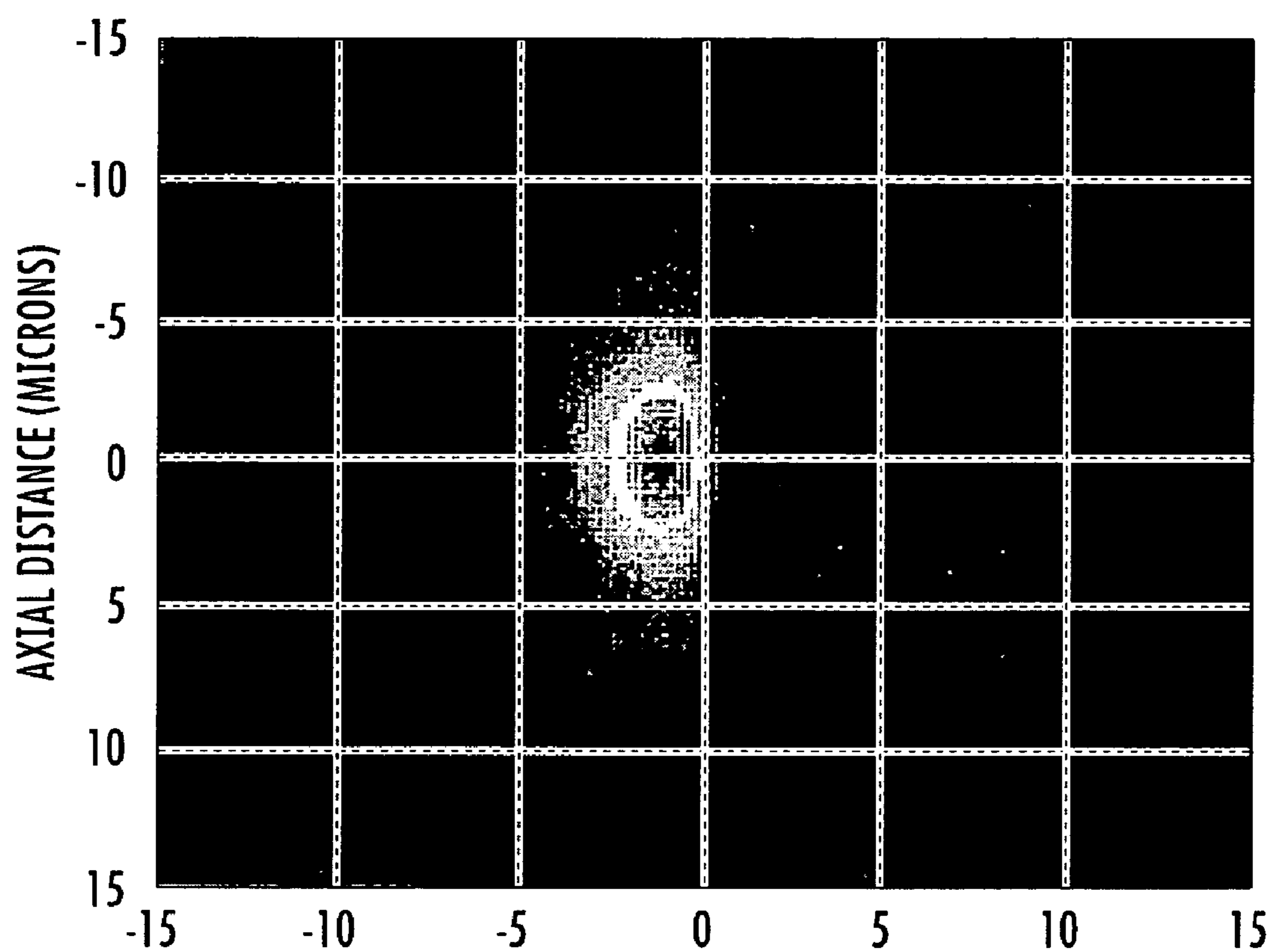
MODELED RIDGE-GUIDED WAVE ON A MICROCYLINDER
