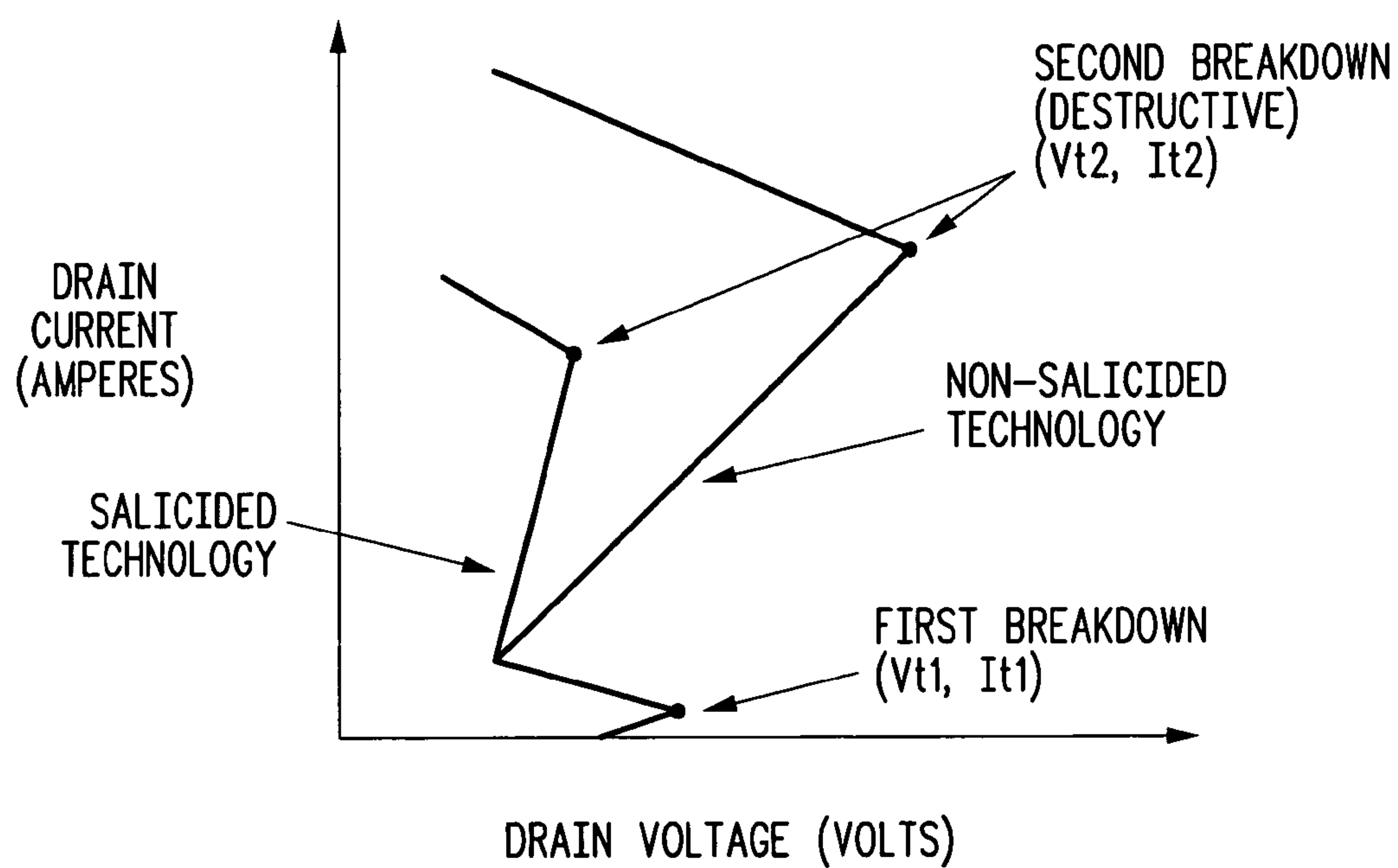
FIG. 2 -PRIOR ART-
