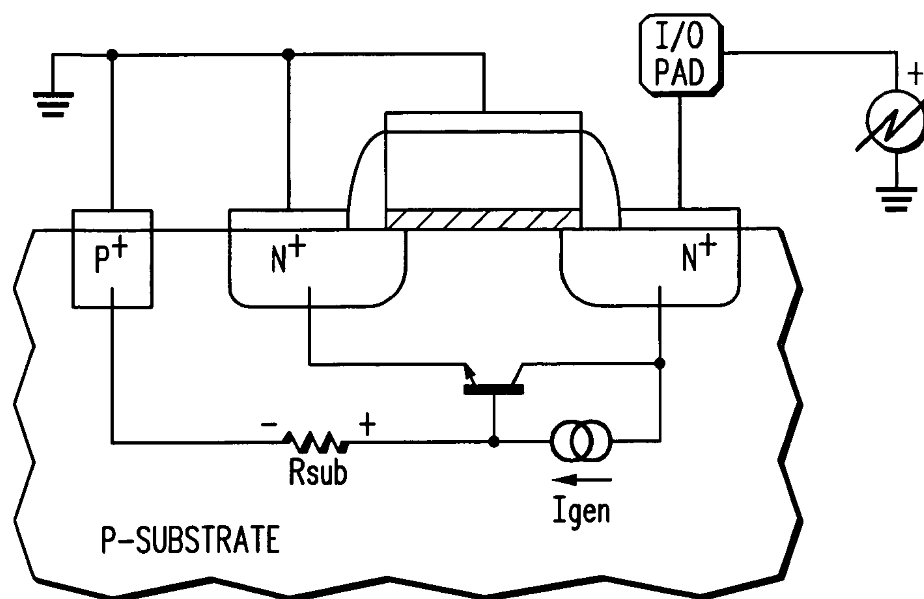
FIG. 1 -PRIOR ART-
