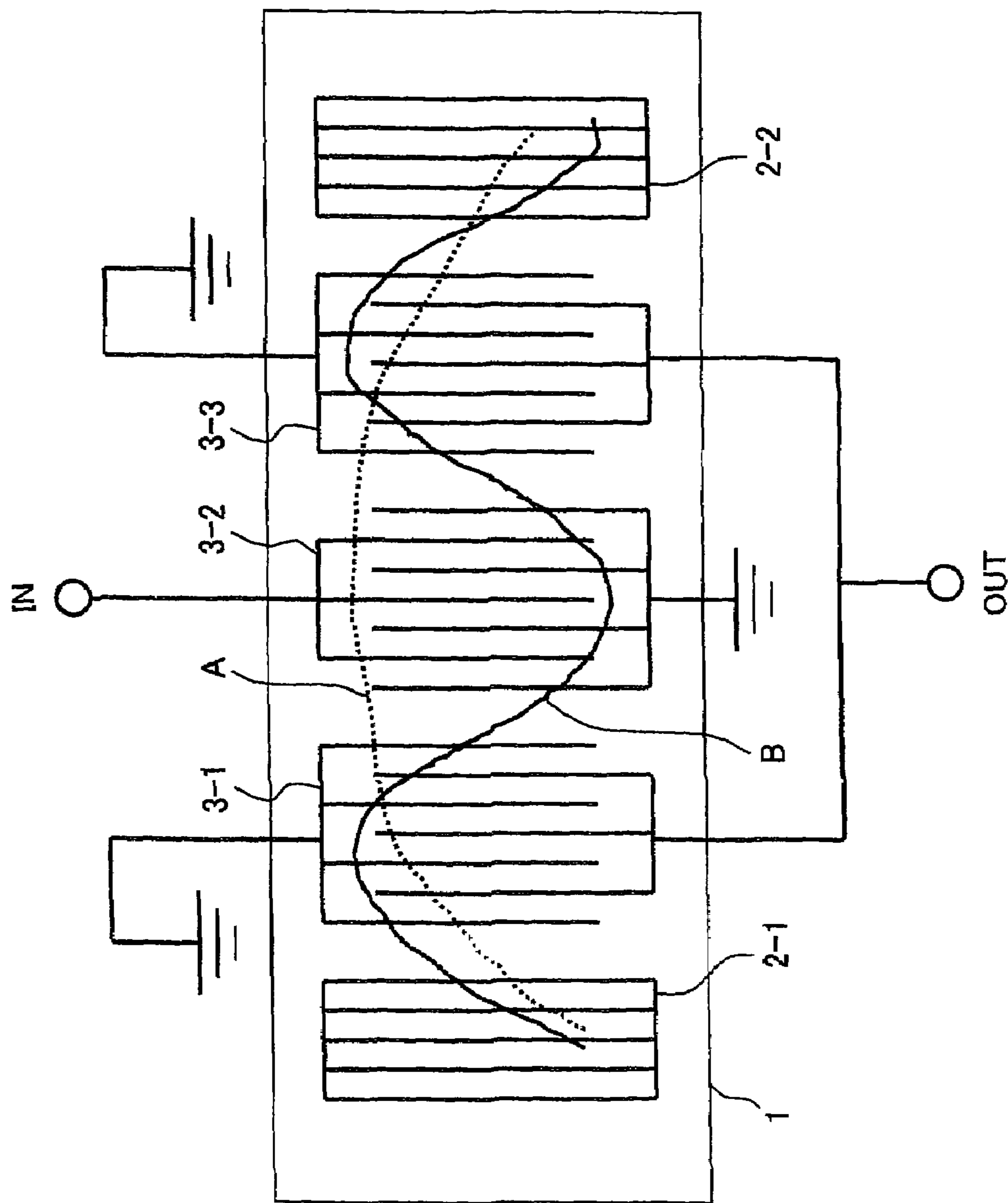
Fig. 1 PRIOR ART
