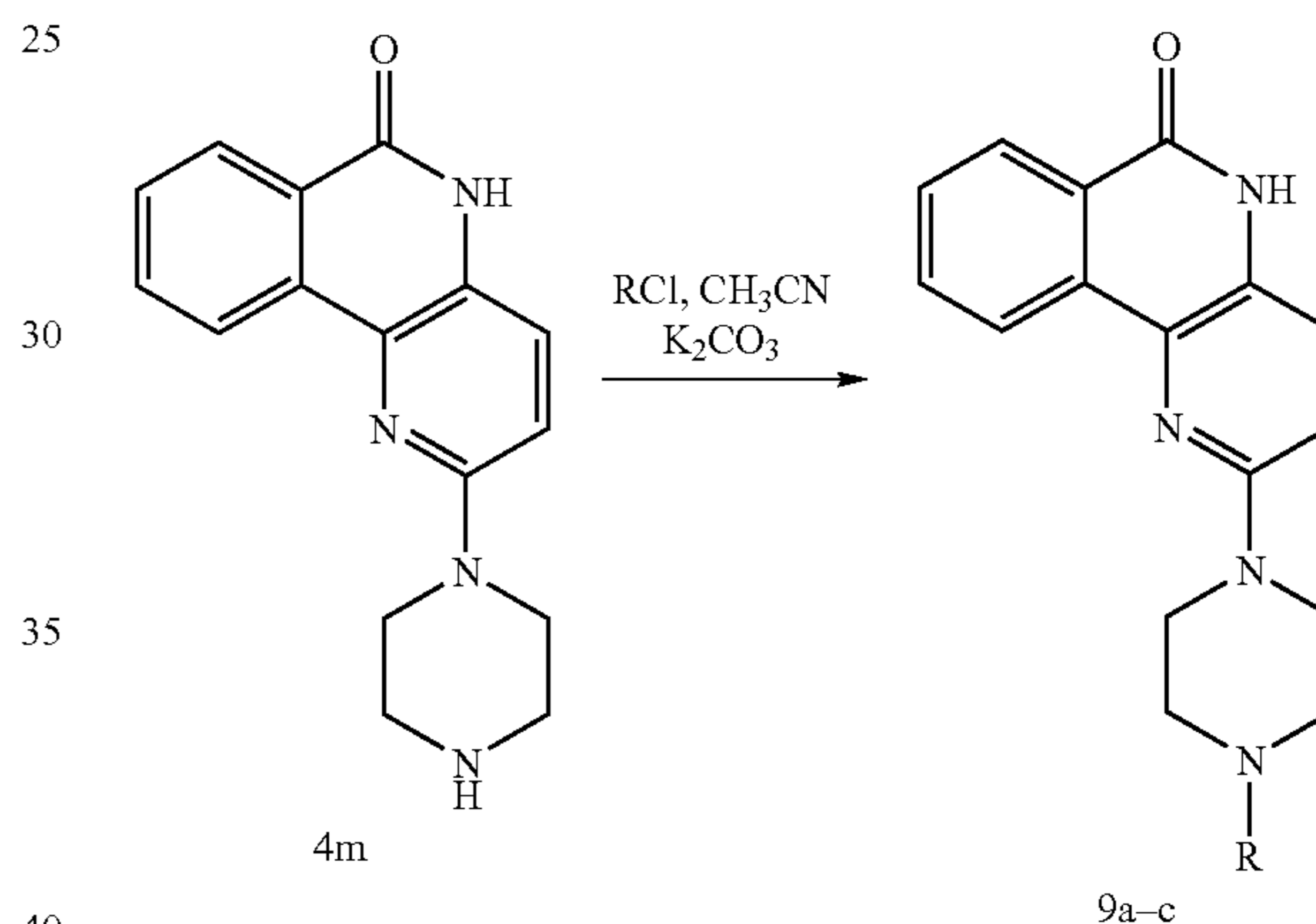
Scheme 6-5. Synthesis of amines 9a-c.
