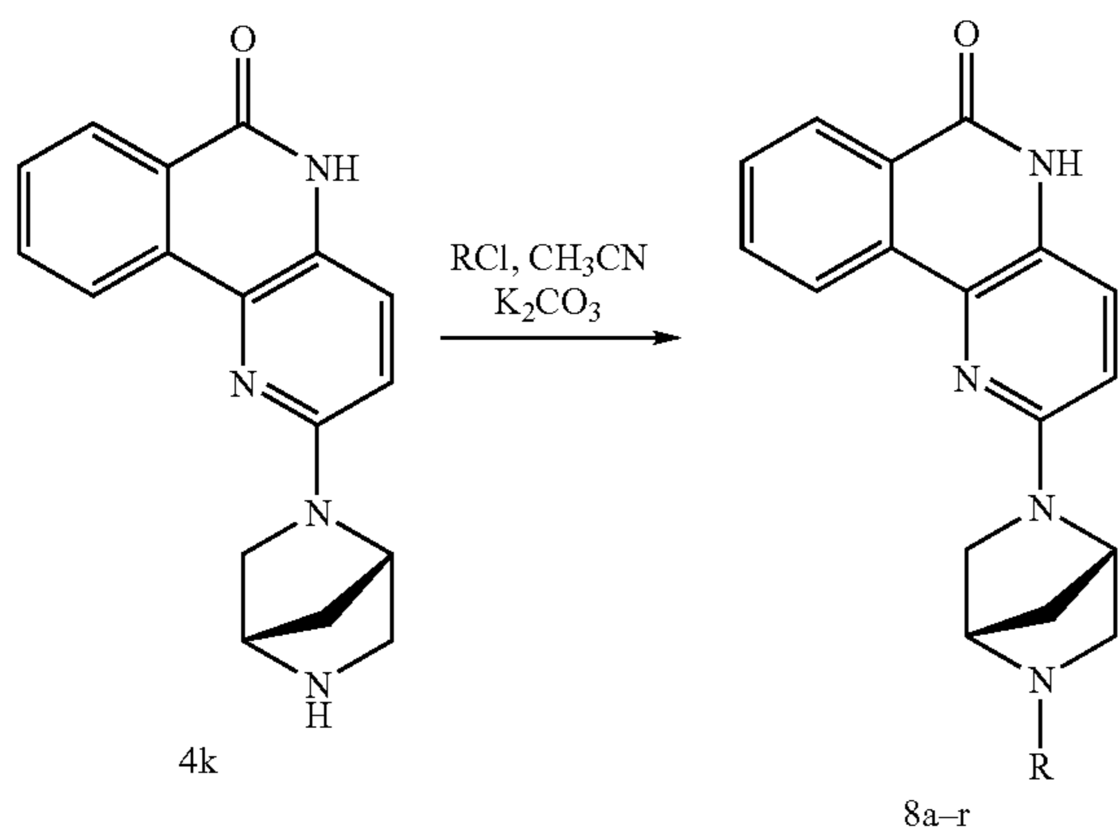
Scheme 5-5. Synthesis of the amines 8a-r.
