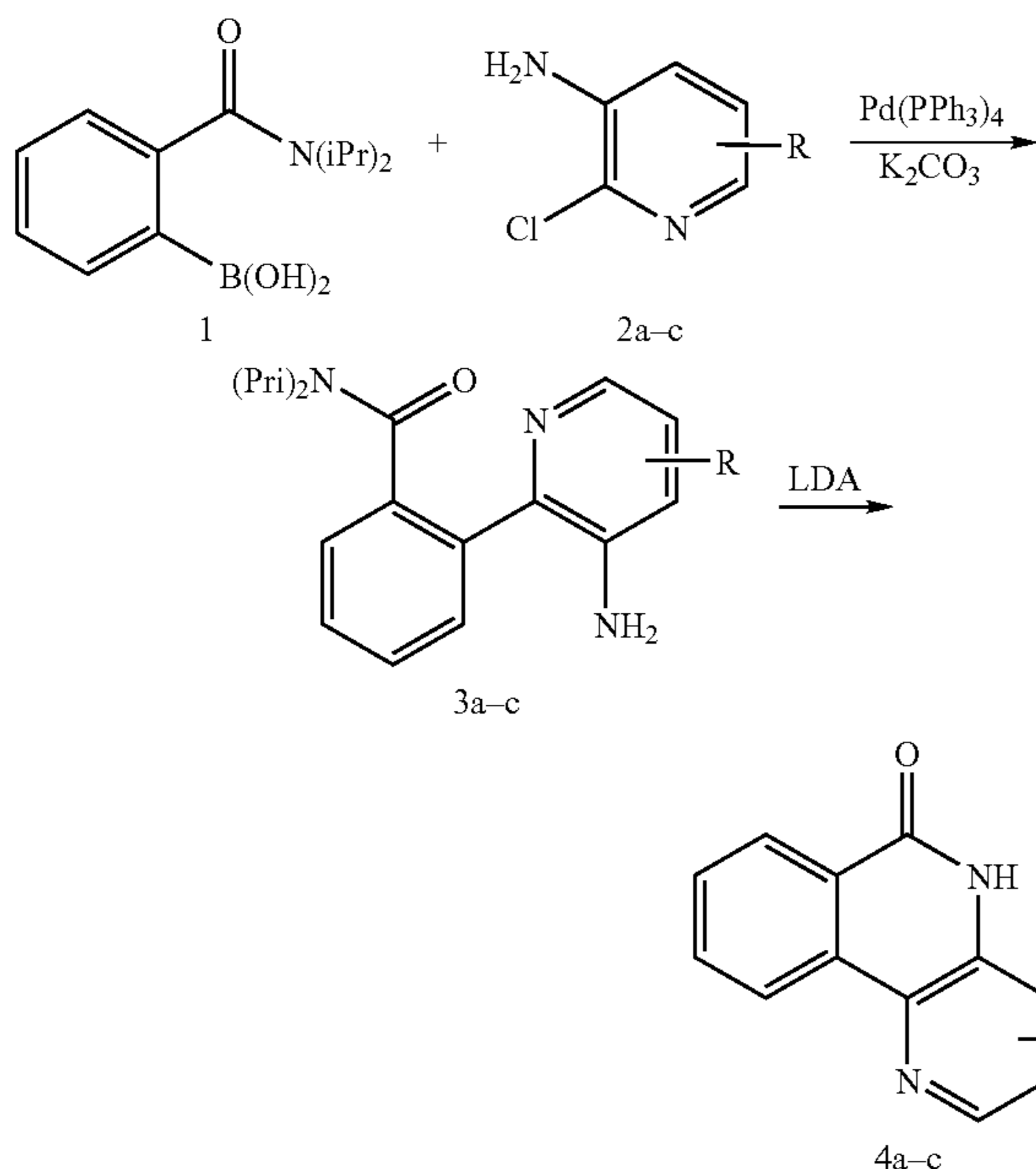
Scheme 1-5. General Scheme for synthesis of azaphenanthridones 4a-c.
