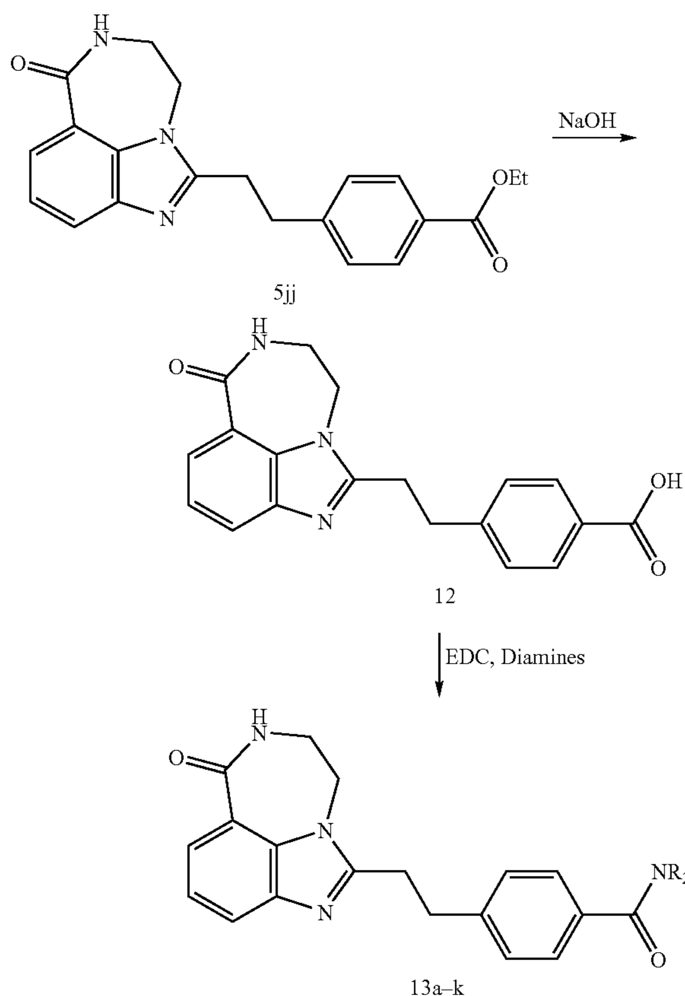
Scheme 7-4. Synthesis of amides 13a-k.
