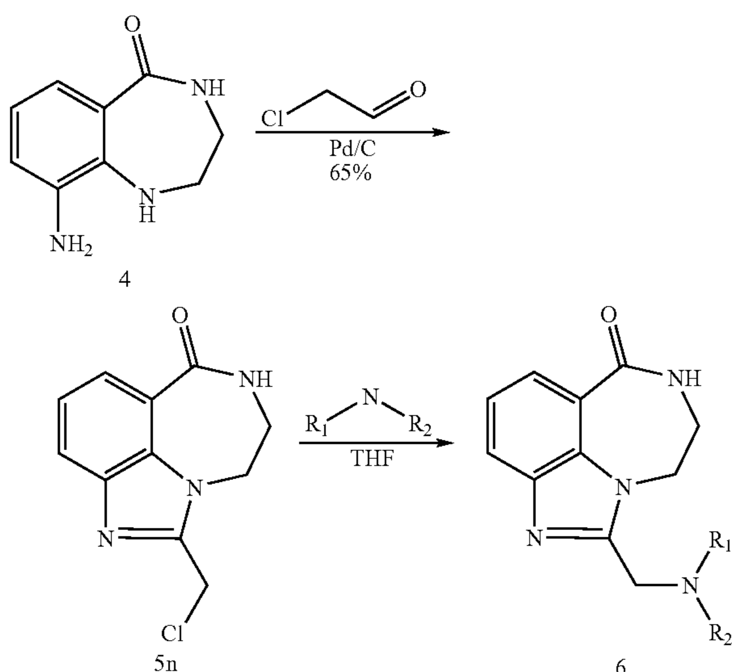
Scheme 3-4 Synthesis of imidazobenzodiazepine amines 6a–dd.
