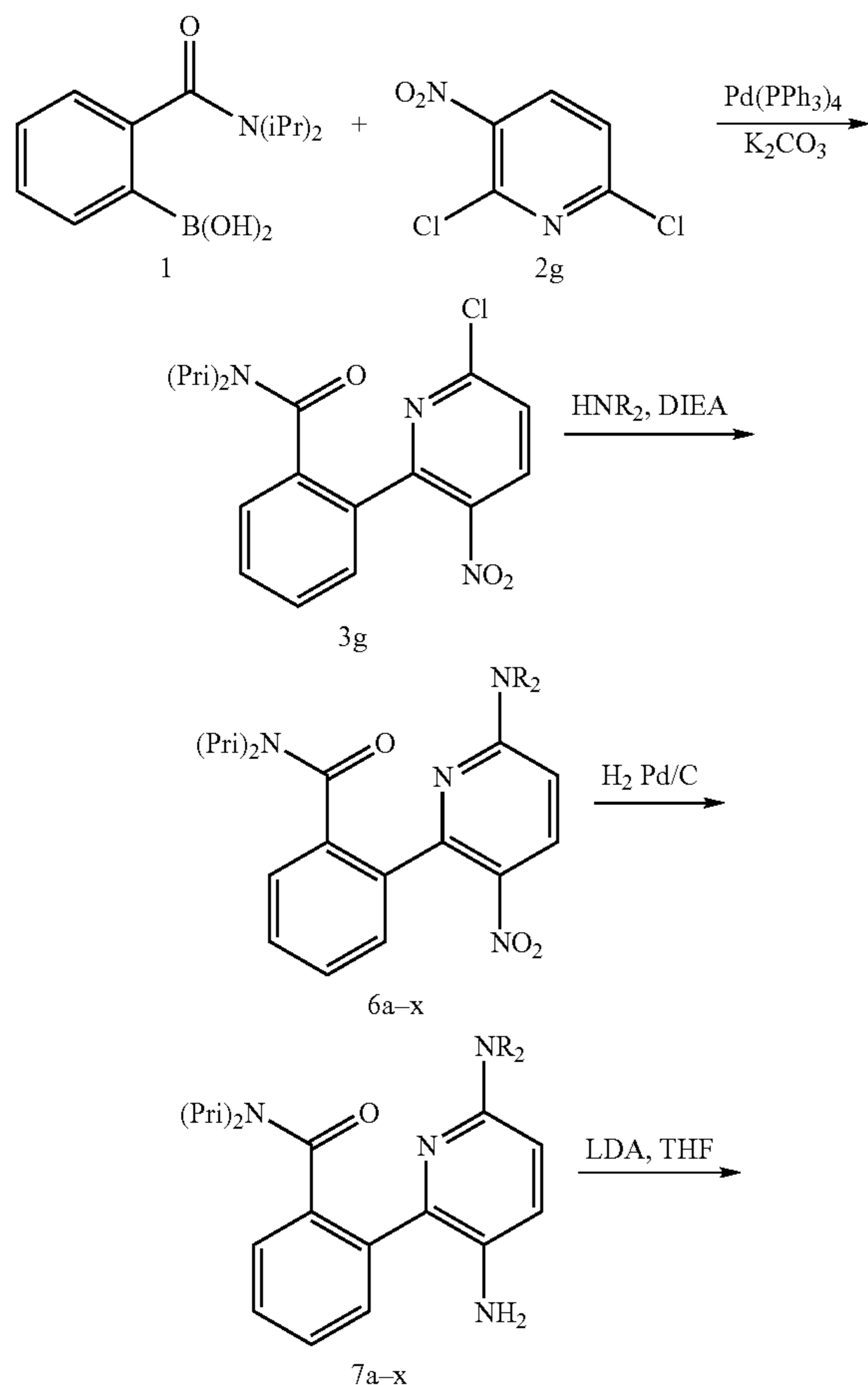
Scheme 4-5. General Scheme for synthesis of azaphenanthridone amines 4h–x.
