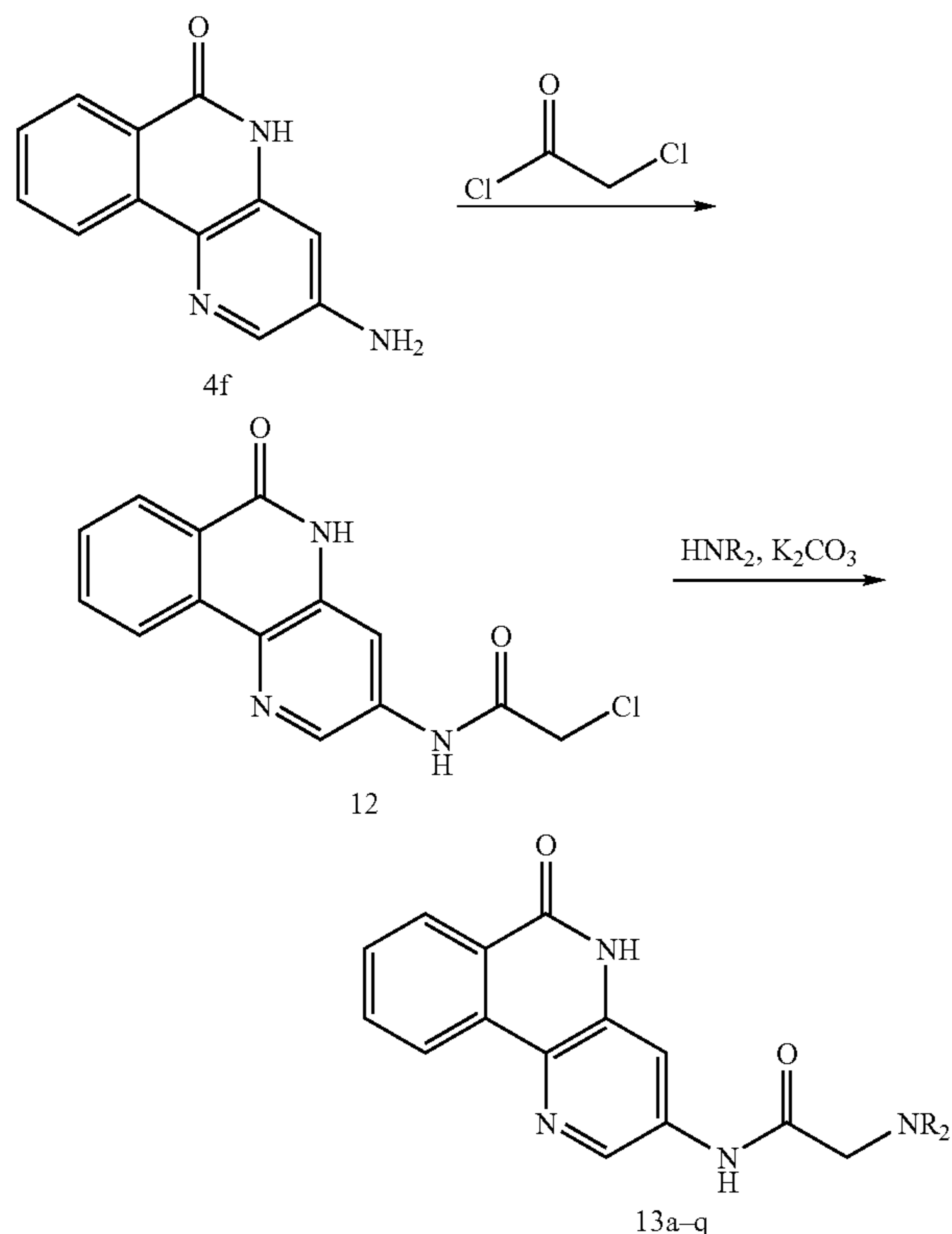
Scheme 8-5. Amides derivatives of aniline 4f.
