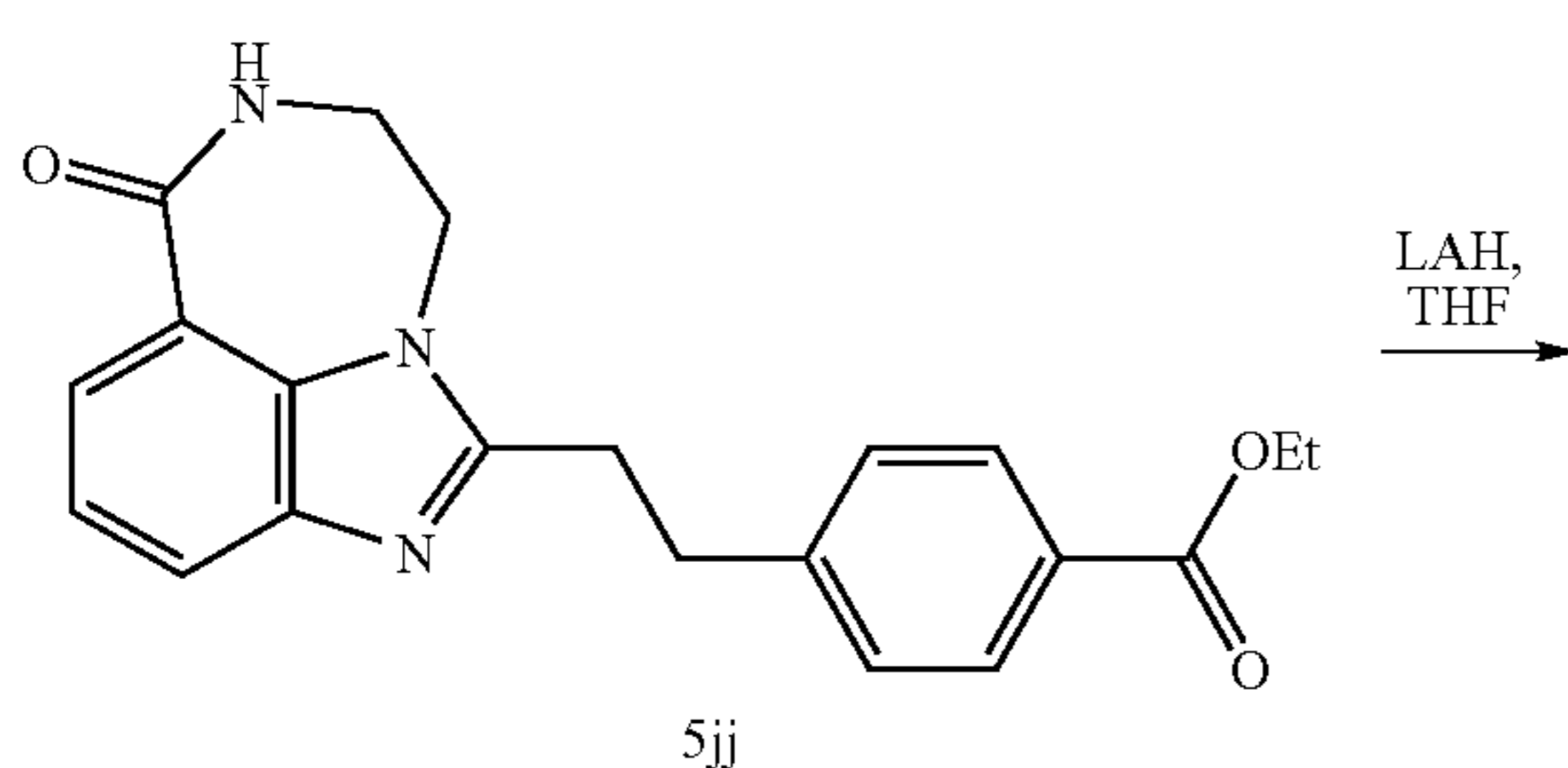
Scheme 6-4. Synthesis of amines 11a-f.
