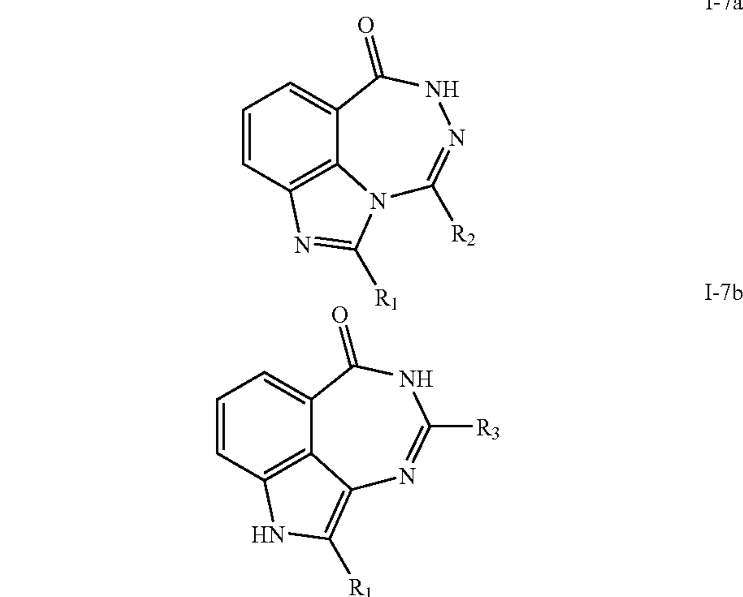
Scheme I-7 Synthesis of Imidazolobenz-1,3,4-triazepin-5-one
