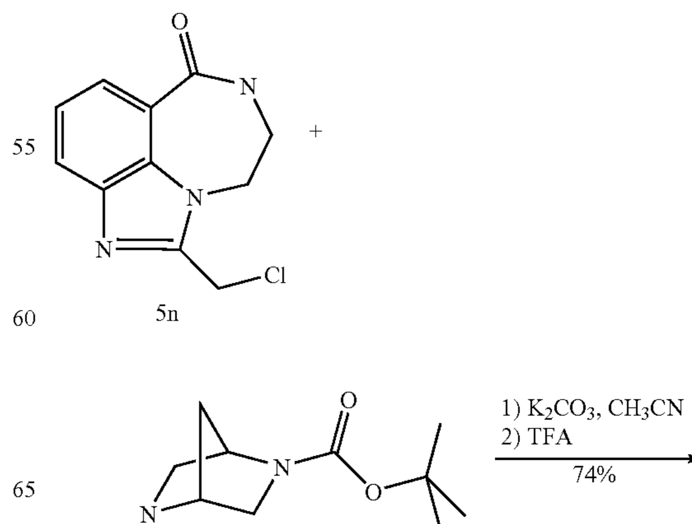
Synthesis of Bicyclic Amines 8a-t.
