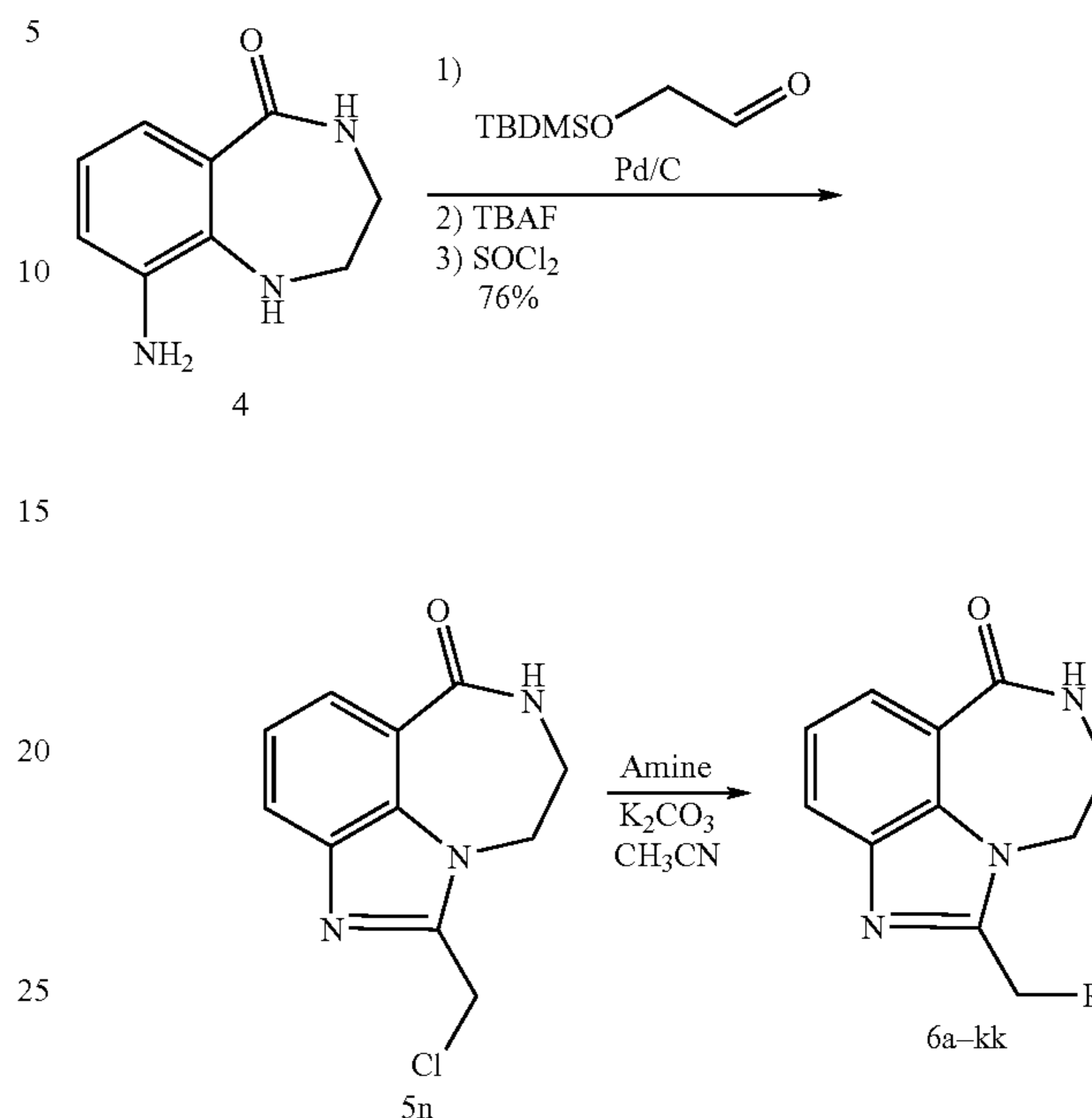
Scheme 3-4a. Alternative Synthesis of imidazobenzodiazepine amines 6a–kk.
