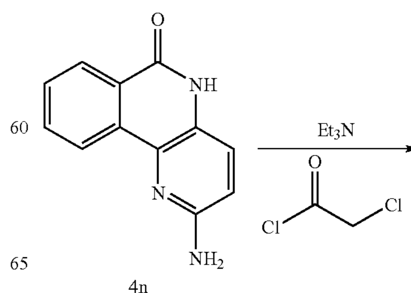
Scheme 7-5. Synthesis of amines 11a-x.
