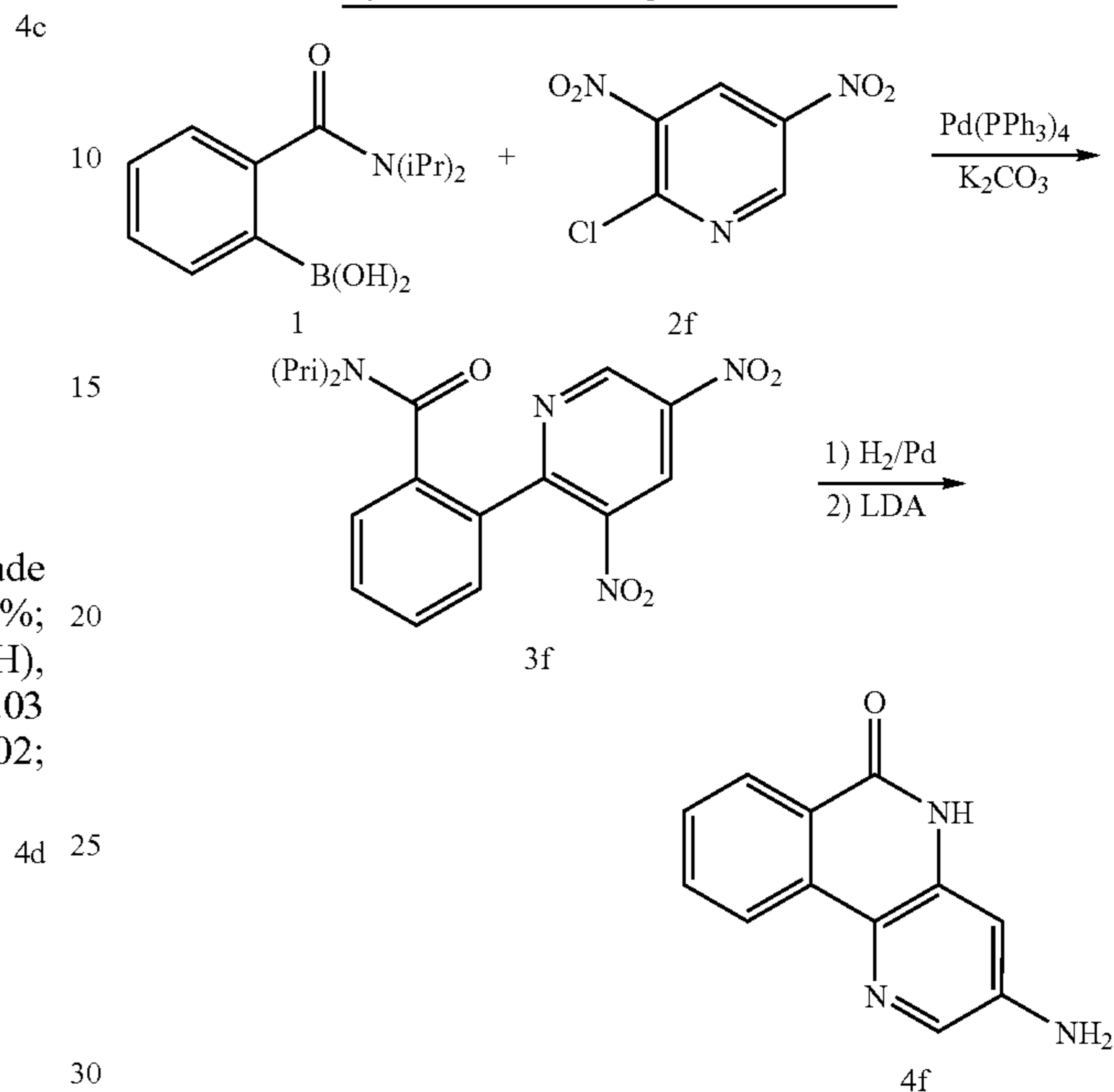
Scheme 2-5. Synthesis of Aminoazaphenanthridone 4f.
