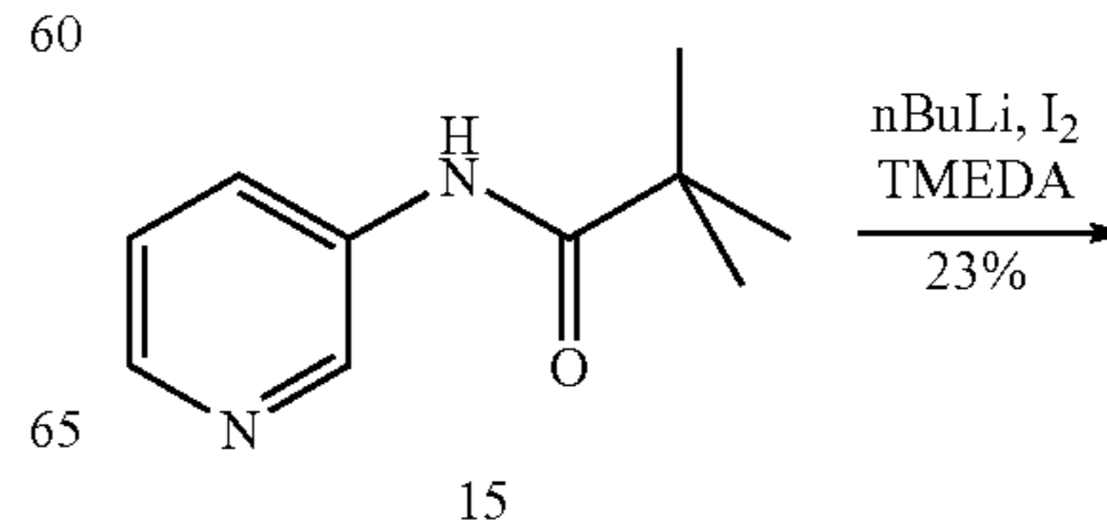
Scheme 1-10. General Synthesis of 3-azaphenanthridones.
