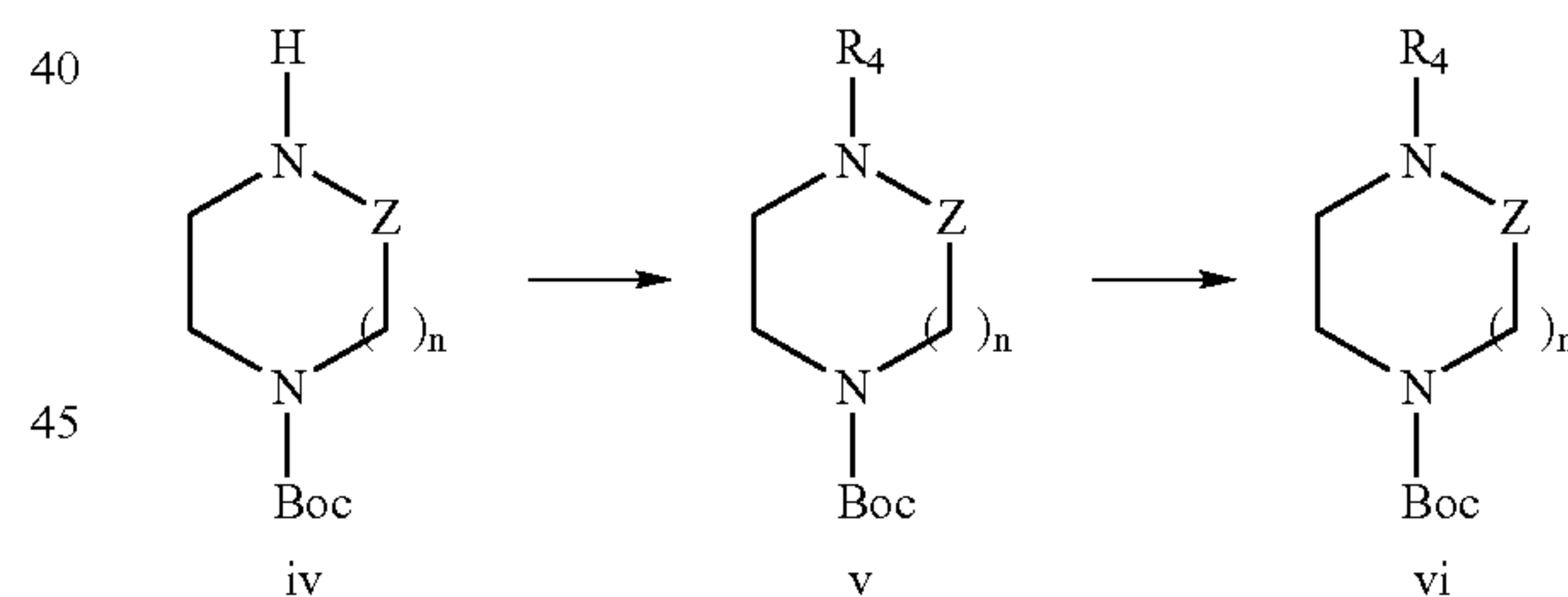
Reaction Scheme 8
