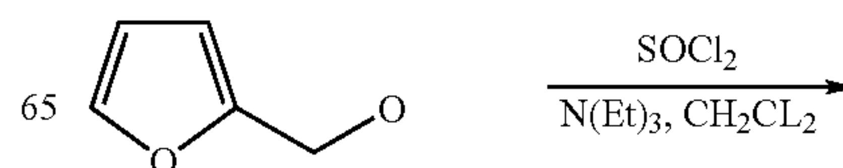
Reaction Scheme 7
