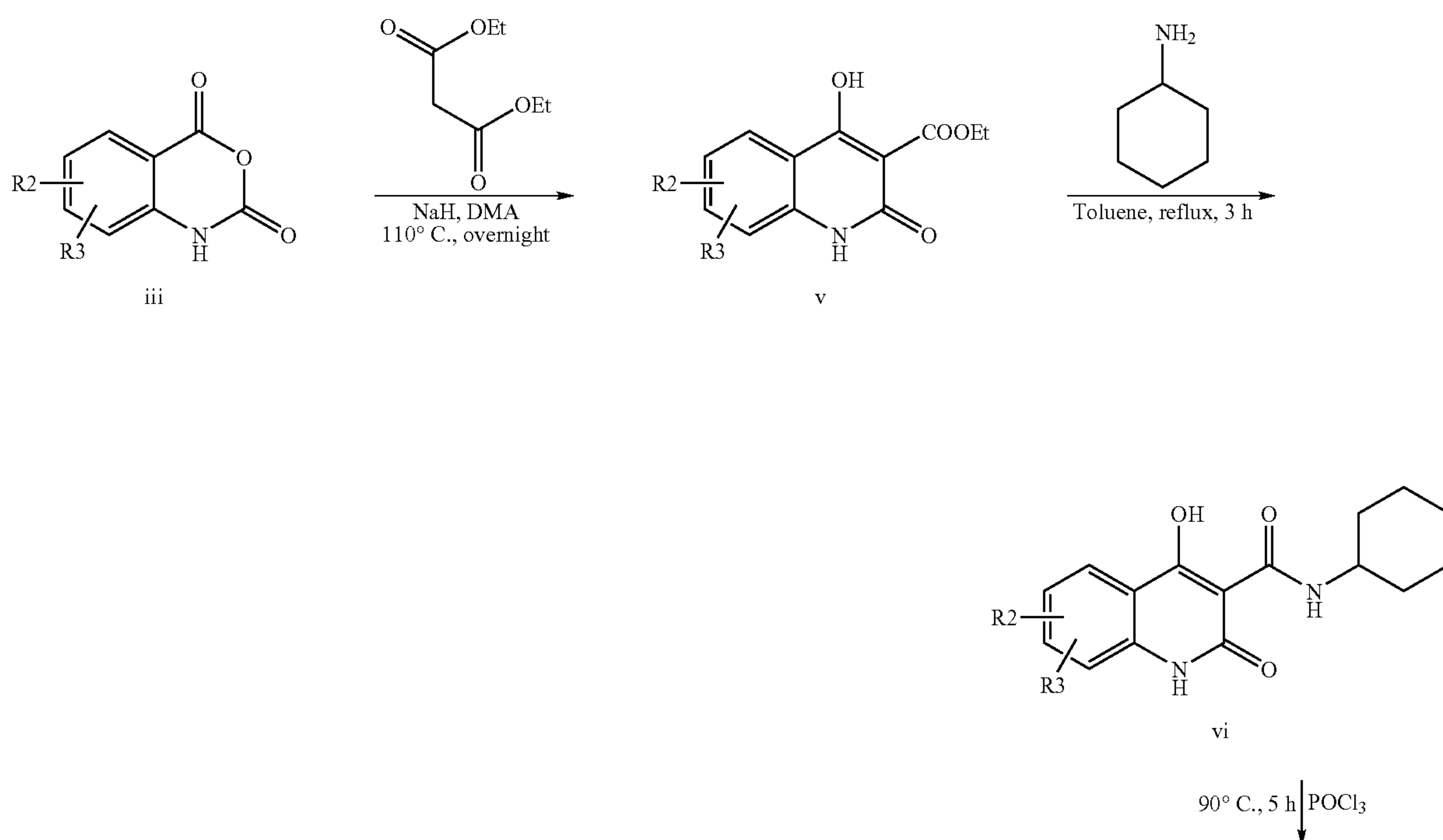
Reaction Scheme 4
