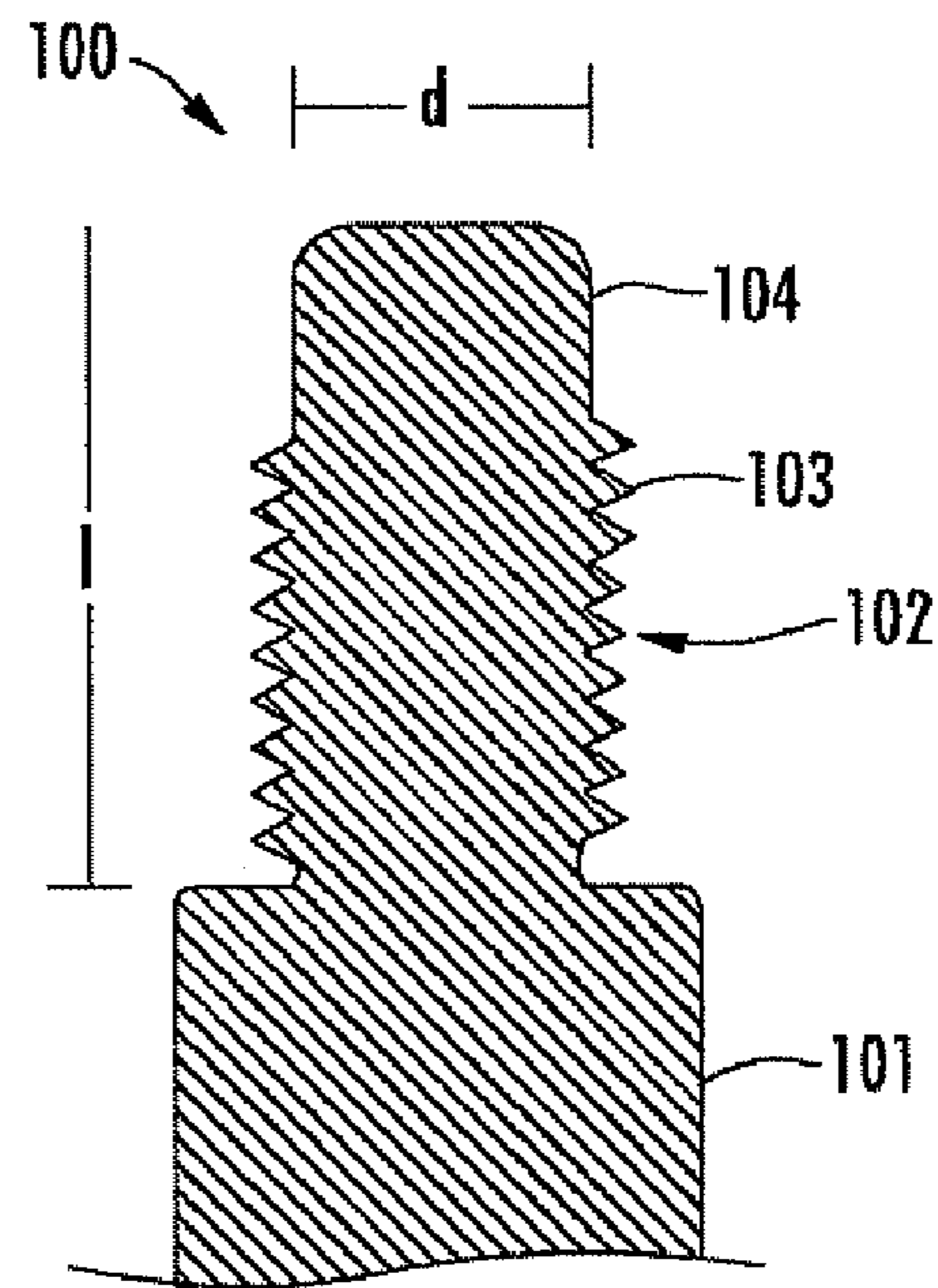
FIG. 6 PRIOR ART
