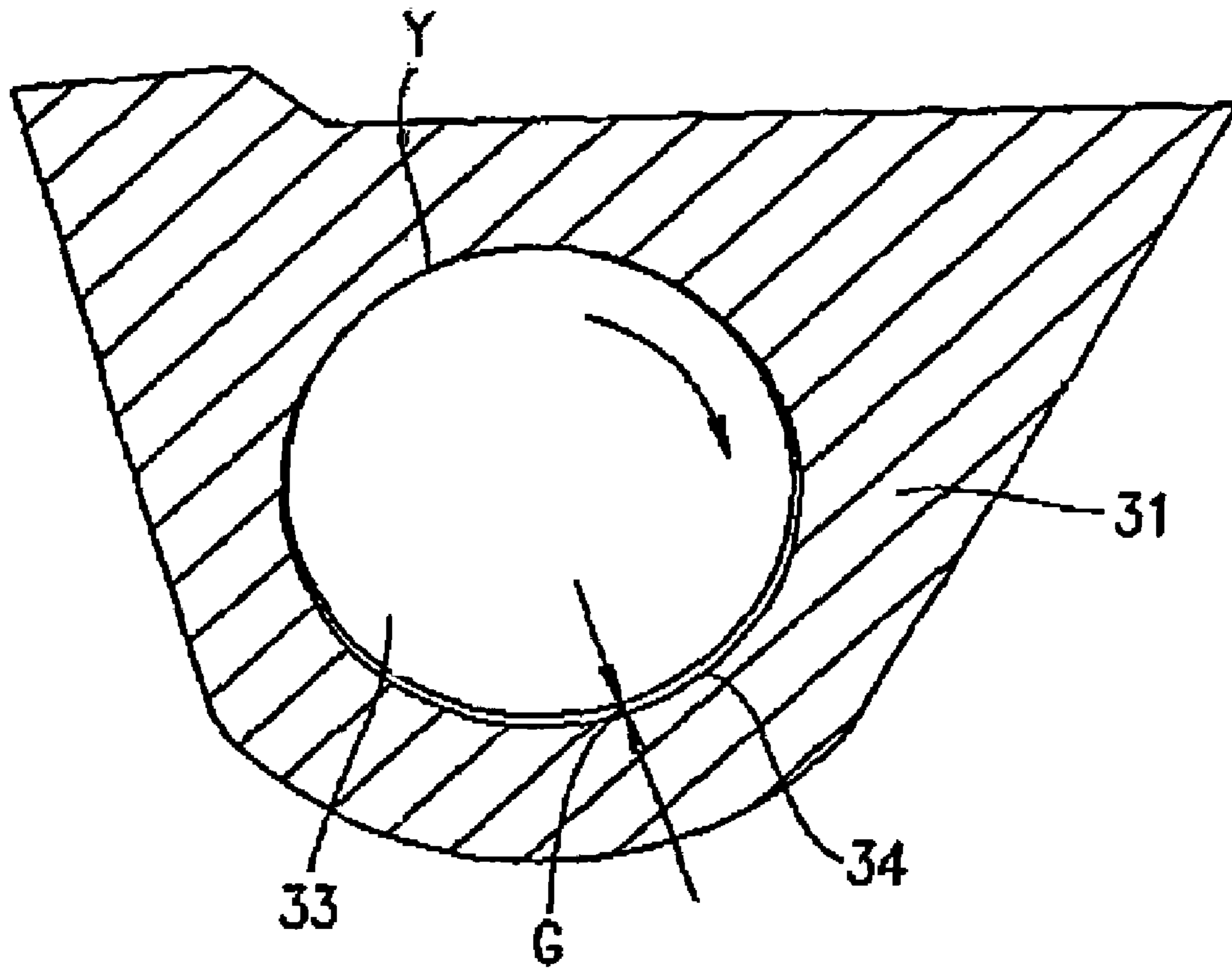
FIG. 16 CONVENTIONAL ART
