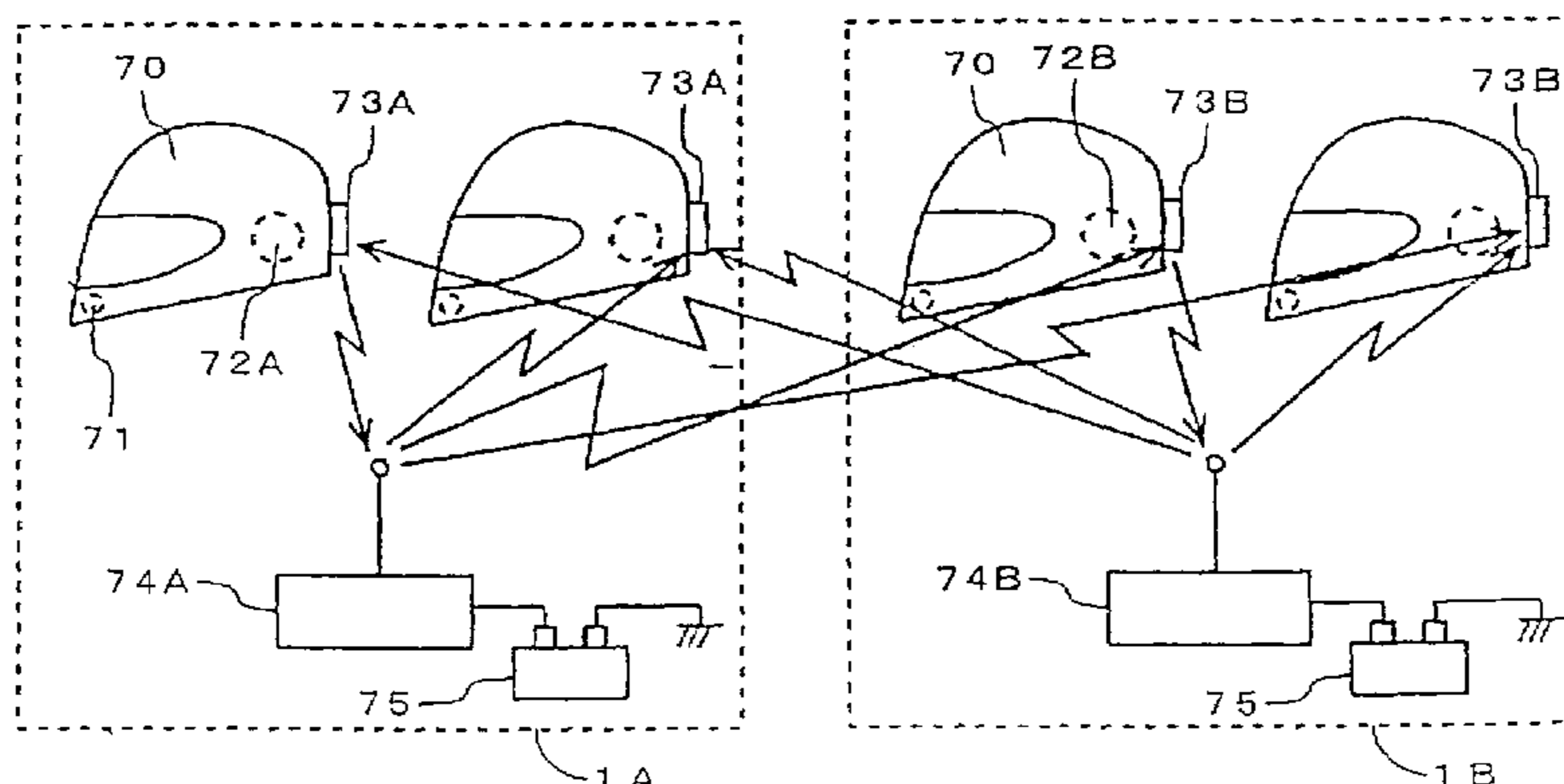
74A, 74B: REPEATING APPARATUS
