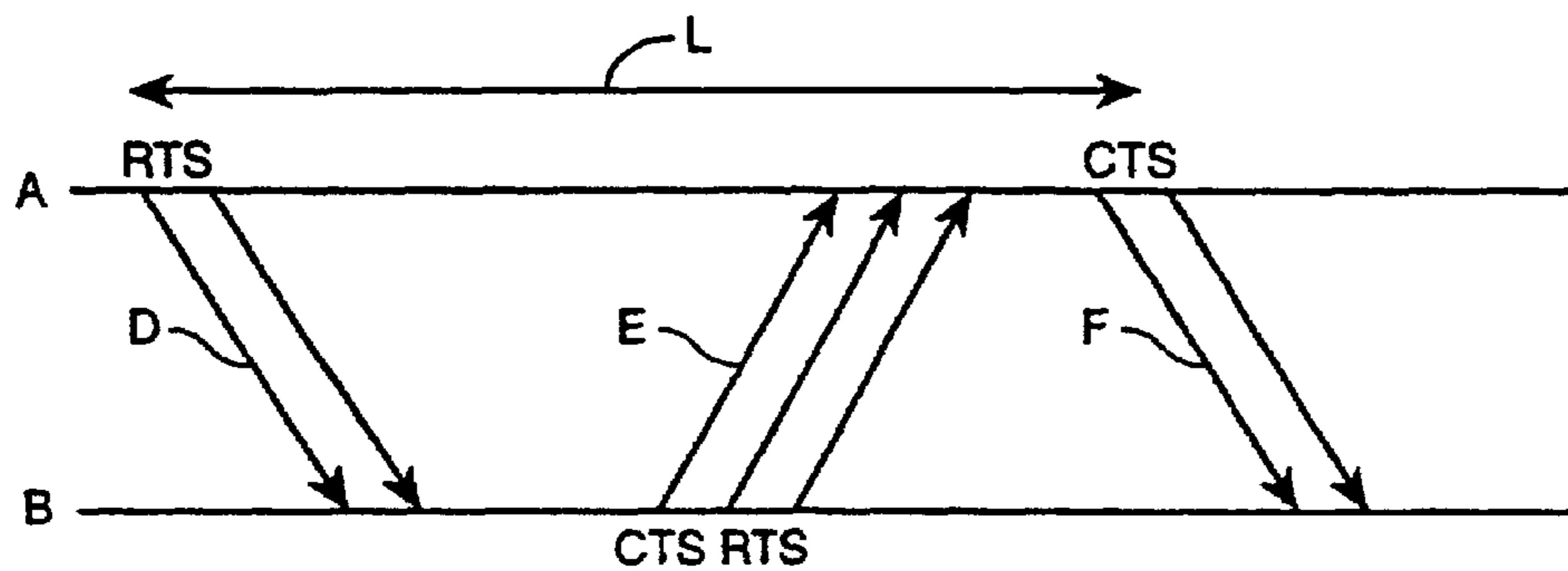
Fig. 4 (Prior Art)
