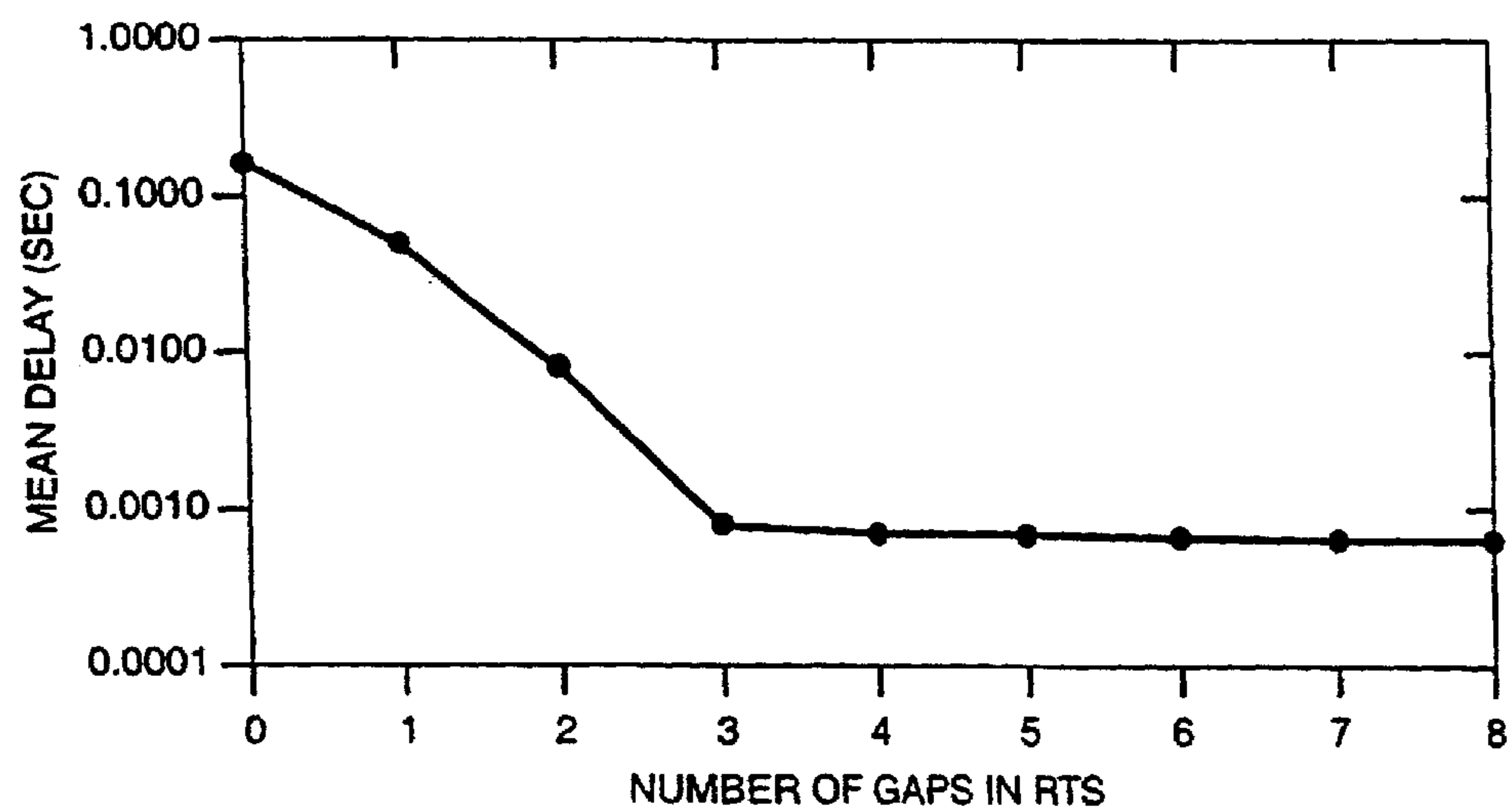
Fig. 7 (Prior Art)
