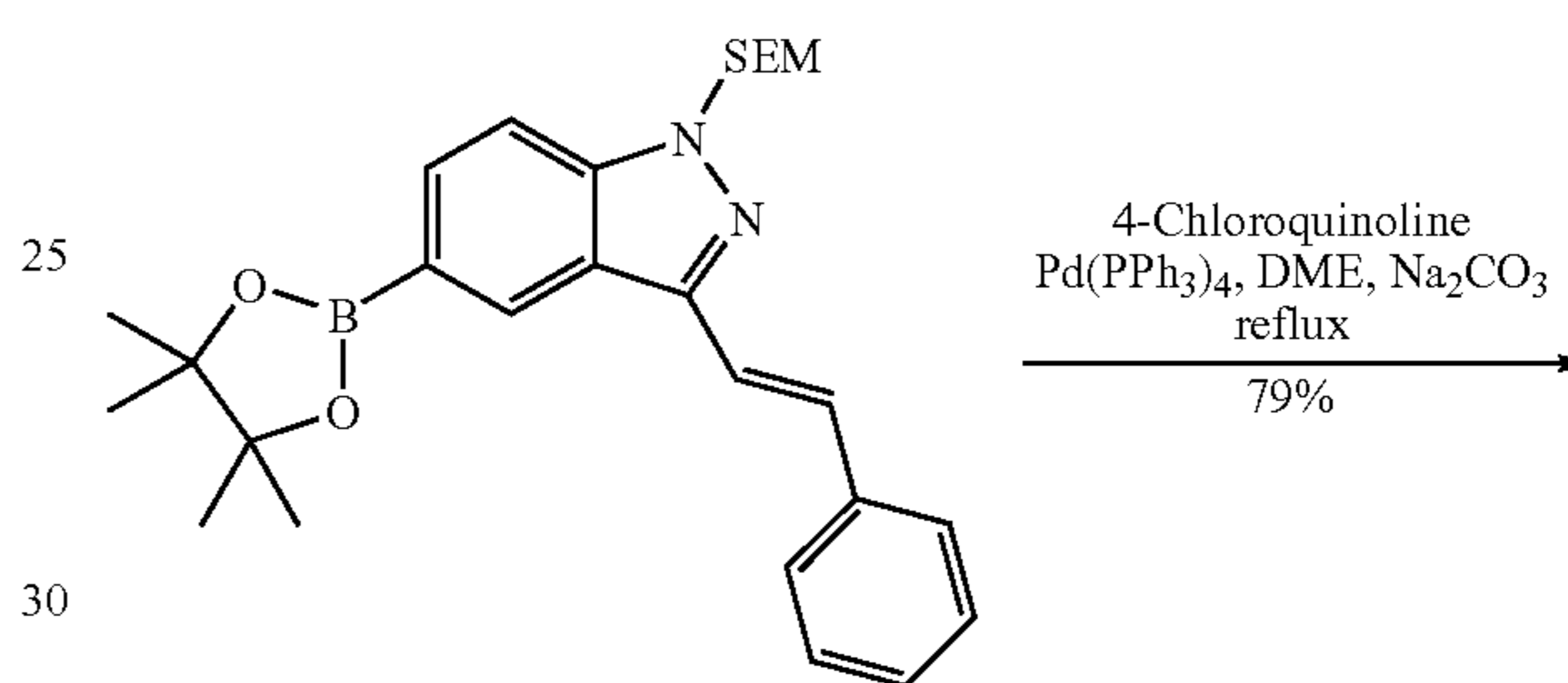
(a) Intermediate 16a—3-((E)-Styryl)-5-(4,4,5,5-tetramethyl-[1,3,2]dioxaborolan-2-yl)-1-(2-trimethylsilylanyl-ethoxymethyl)-1H-indazole
