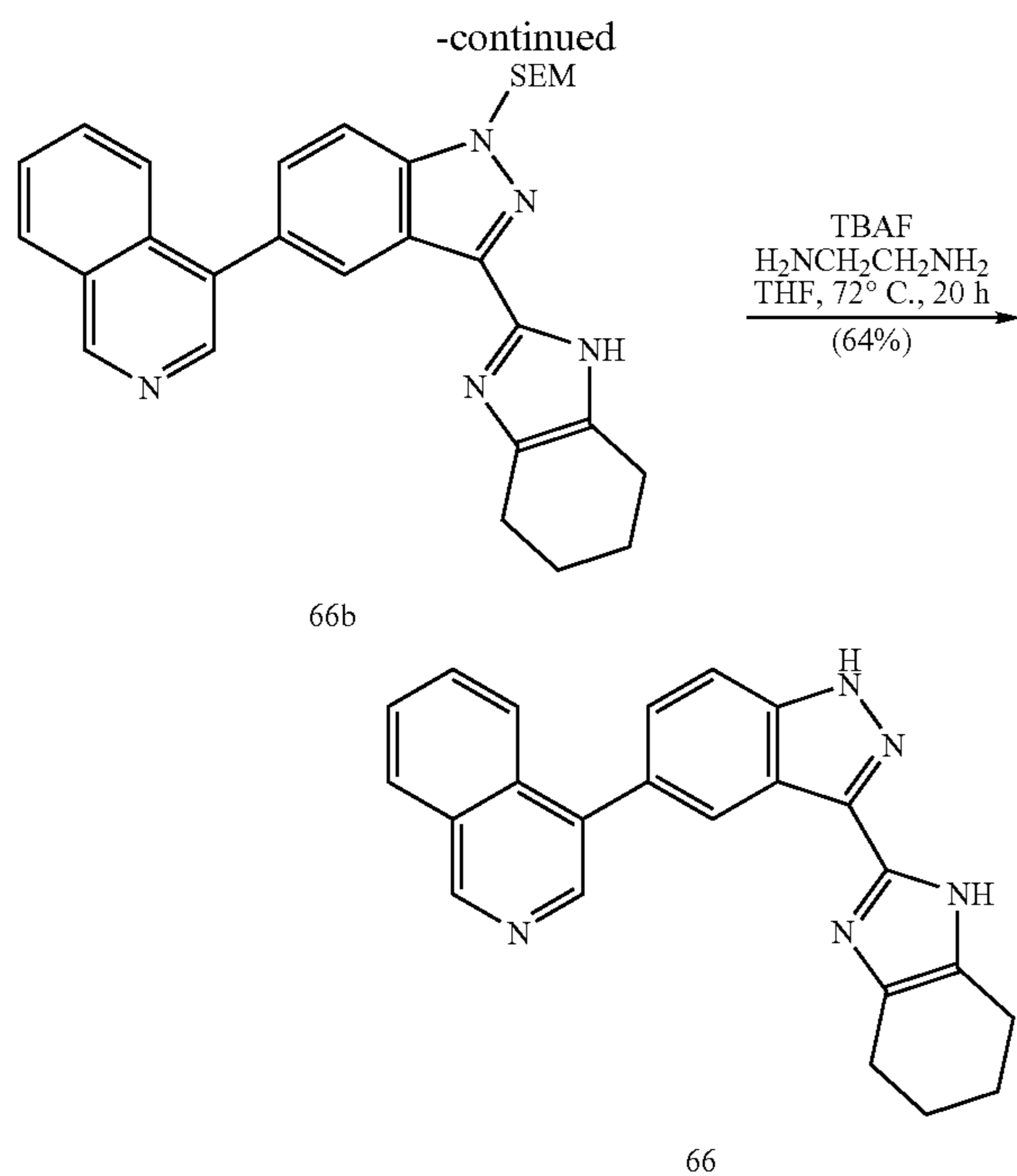
(a) Intermediate 66a—5-Iodo-3-(4,5,6,7-tetrahydro-1H-benzimidazol-2-yl)-1H indazole
