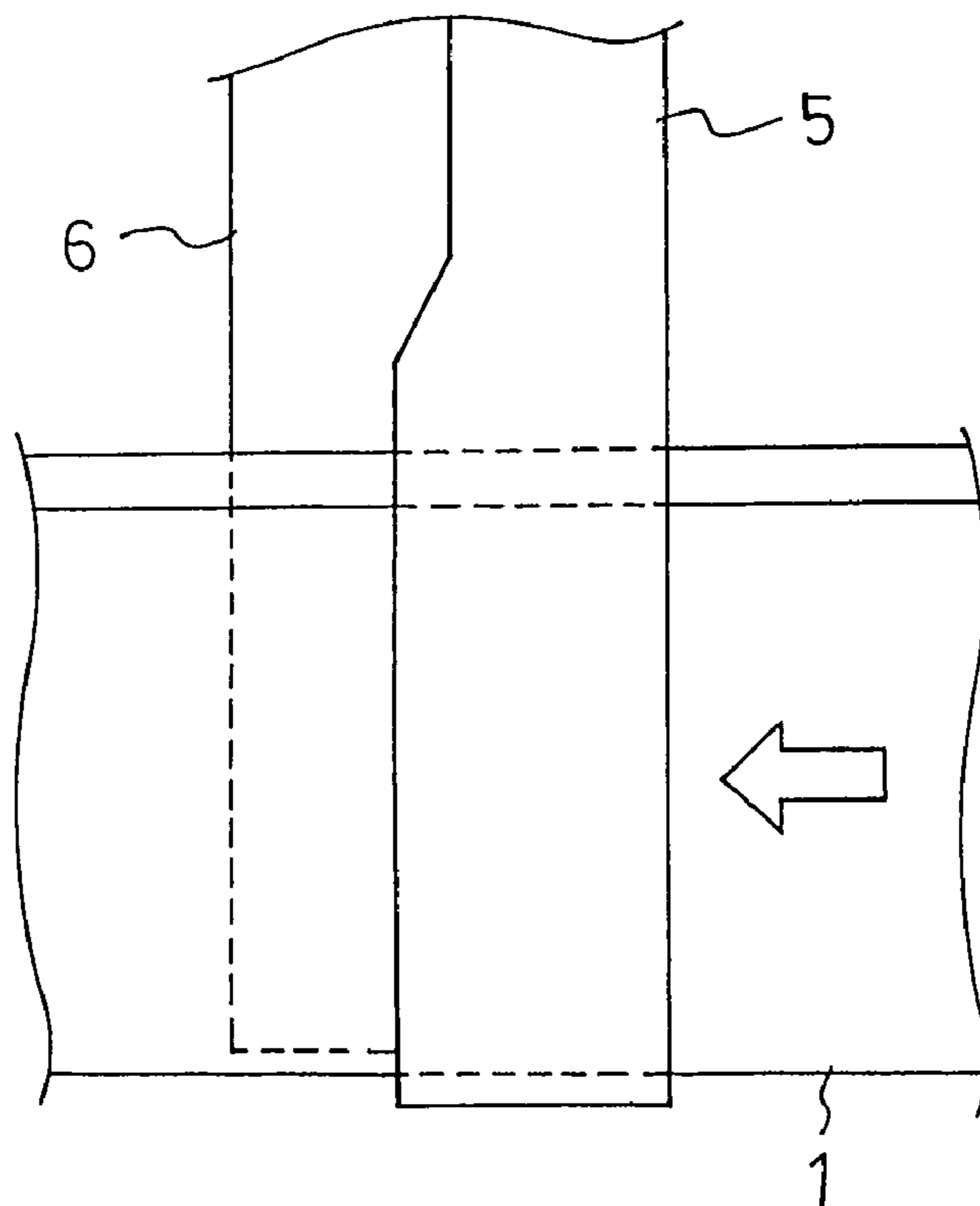
Fig. 59 (PRIOR ART)
