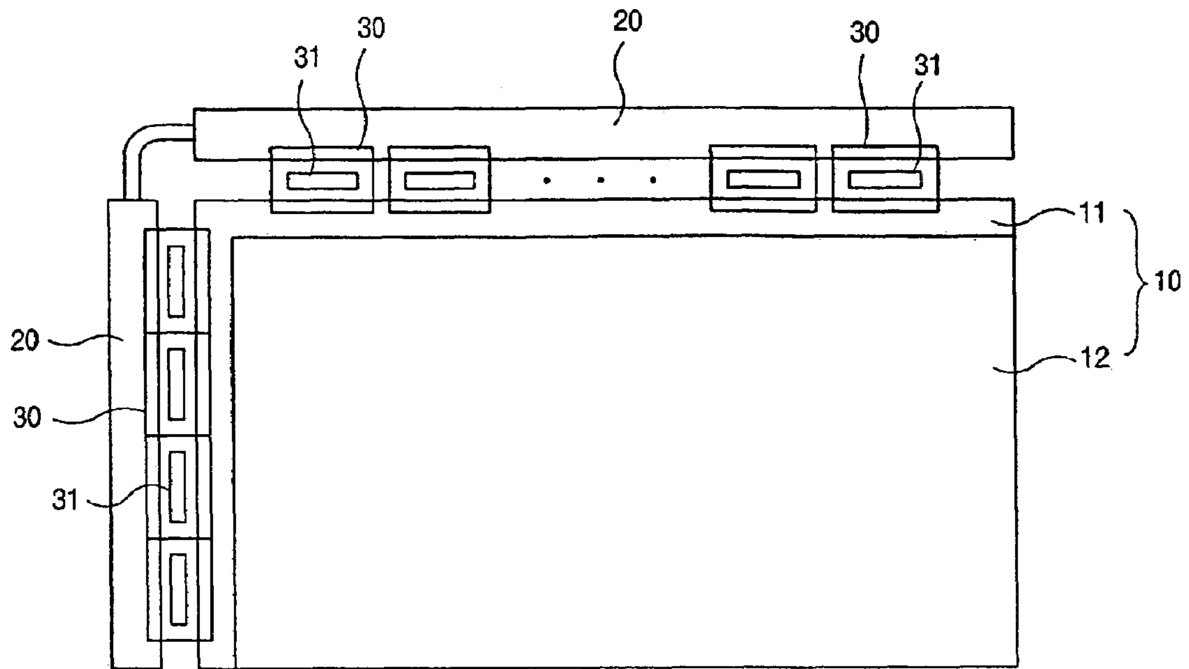
FIG. 1 (RELATED ART)
