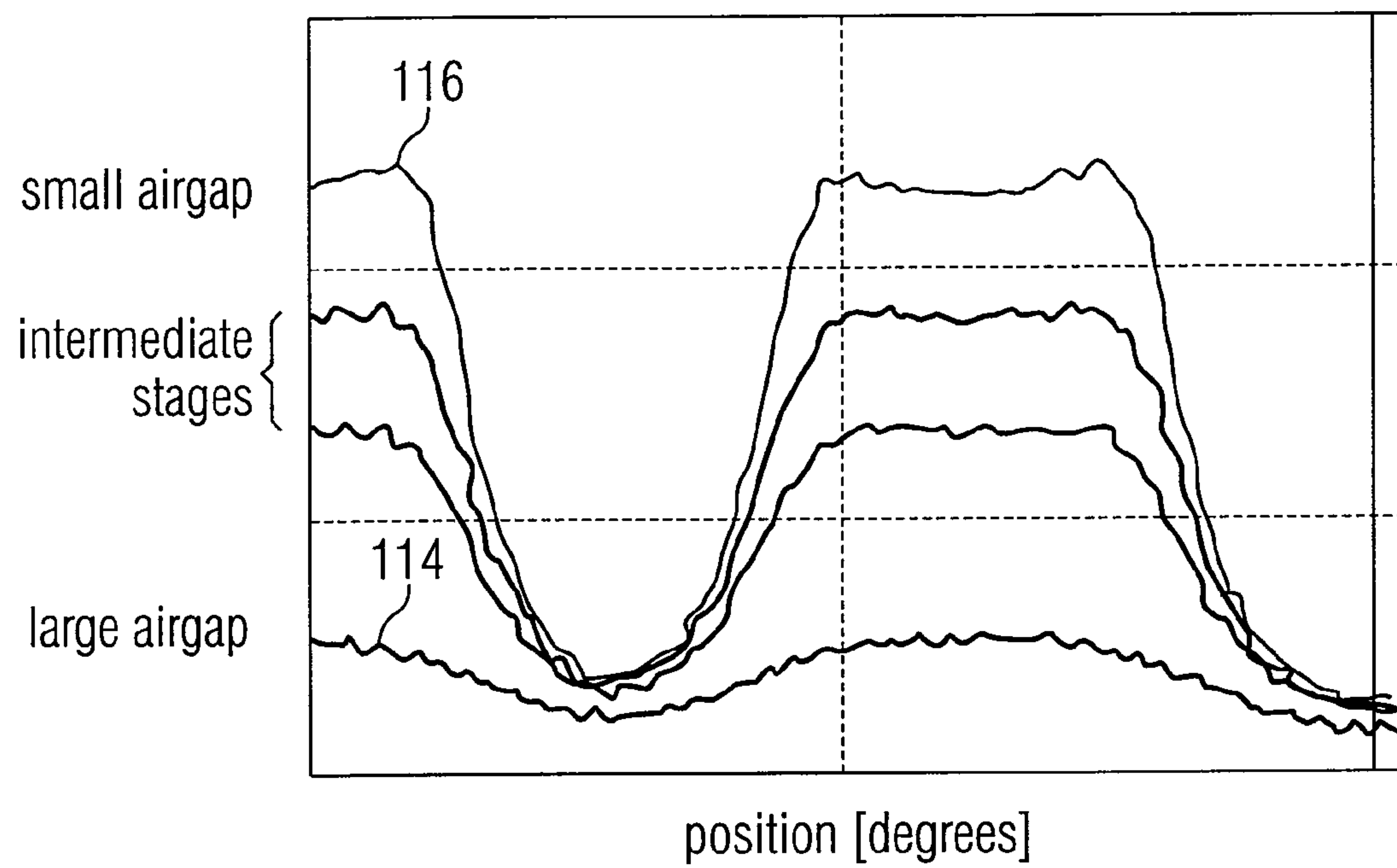
FIG 6C PRIOR ART
