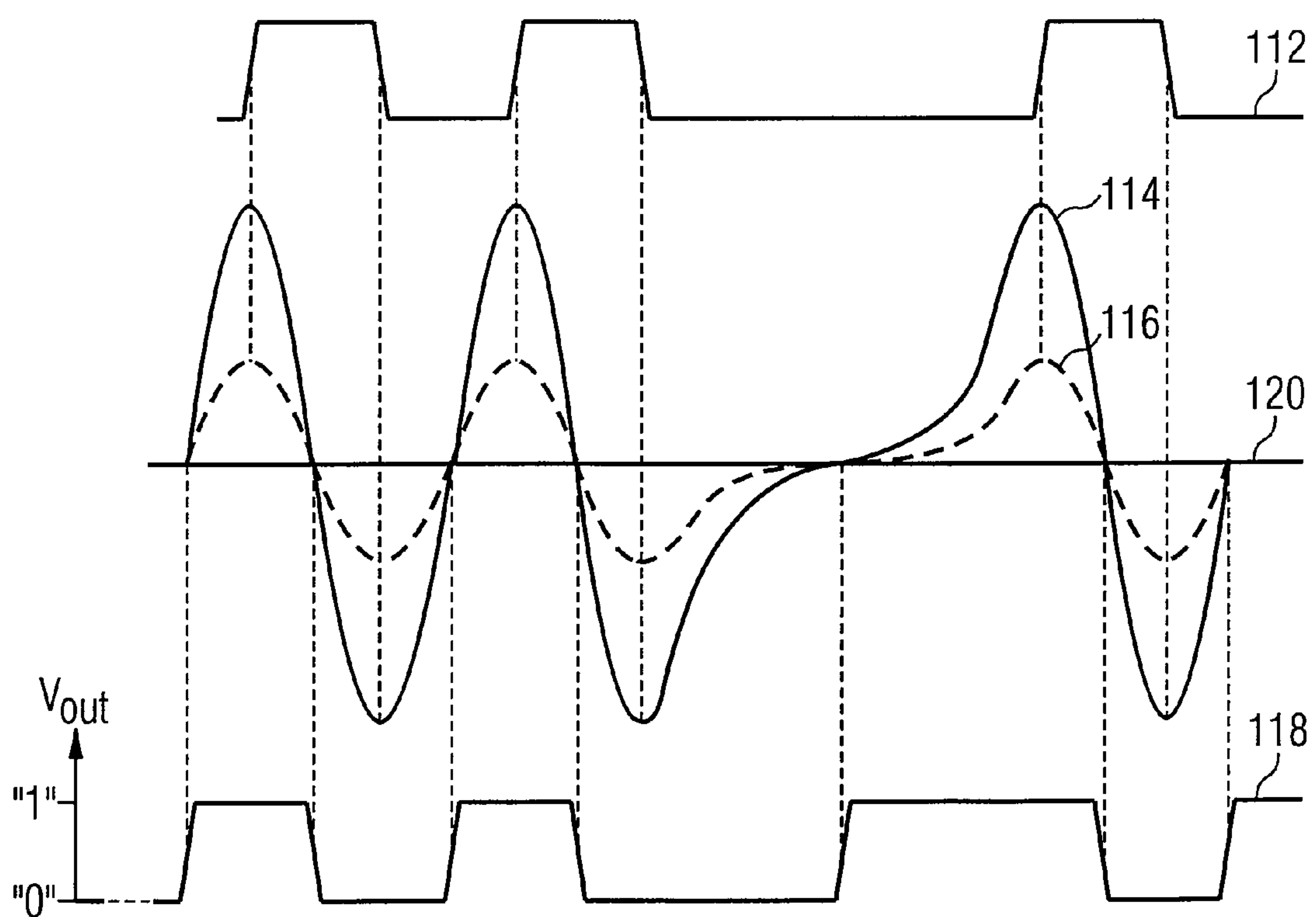
FIG 5 PRIOR ART
